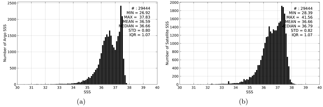
Figure 2: Histograms of SSS from Argo (a) and SMOS-L3-ICDC-V3-MONTHLY-0.5DEG (b) considering all match-up pairs per bins of 0.1 over the Amazon and Orinoco river plumes Pi-MEP region and for the full satellite product period.
