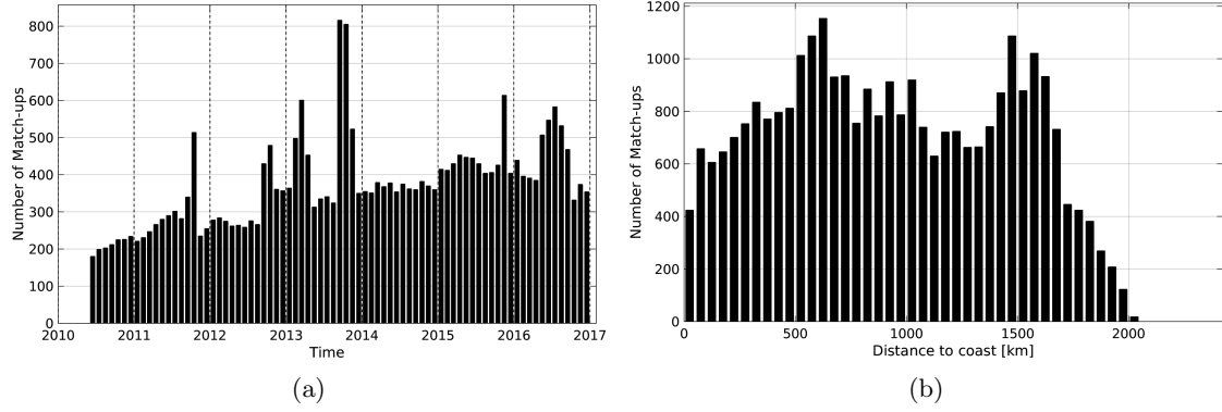
Figure 1: Number of match-ups between Argo and SMOS-L3-ICDC-V3-MONTHLY-0.5DEG SSS as a function of time (a) and as function of the distance to coast (b) over the Amazon and Orinoco river plumes Pi-MEP region and for the full satellite product period.
