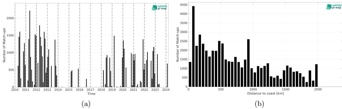
Figure 2: Number of match-ups between TSG (SAMOS) and SMOS SSS L2Q v331 - With FLAG (CMEMS-CATDS-CPDC) SSS as a function of time (a) and as function of the distance to coast (b) over the Amazon and Orinoco river plumes Pi-MEP region and for the full satellite product period.
