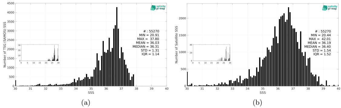
Figure 3: Histograms of SSS from TSG (SAMOS) (a) and SMOS SSS L2Q v331 - With FLAG (CMEMS-CATDS-CPDC) (b) considering all match-up pairs per bins of 0.1 over the Amazon and Orinoco river plumes Pi-MEP region and for the full satellite product period.
