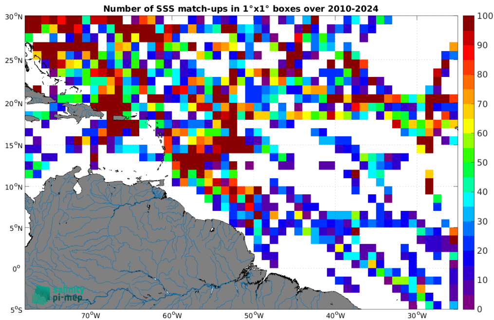
Figure 5: Number of SSS match-ups between TSG (SAMOS) SSS and the SMOS SSS L2Q v331 - With FLAG (CMEMS-CATDS-CPDC) SSS product for the Amazon and Orinoco river plumes Pi-MEP region over 1^\circ \times 1^\circ boxes and for the full satellite product period.
