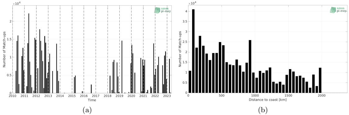
Figure 1: Number of match-ups between TSG (SAMOS) and SMOS SSS L2Q v331 - With FLAG (CMEMS-CATDS-CPDC) SSS as a function of time (a) and as function of the distance to coast (b) over the Amazon and Orinoco river plumes Pi-MEP region and for the full satellite product period.
