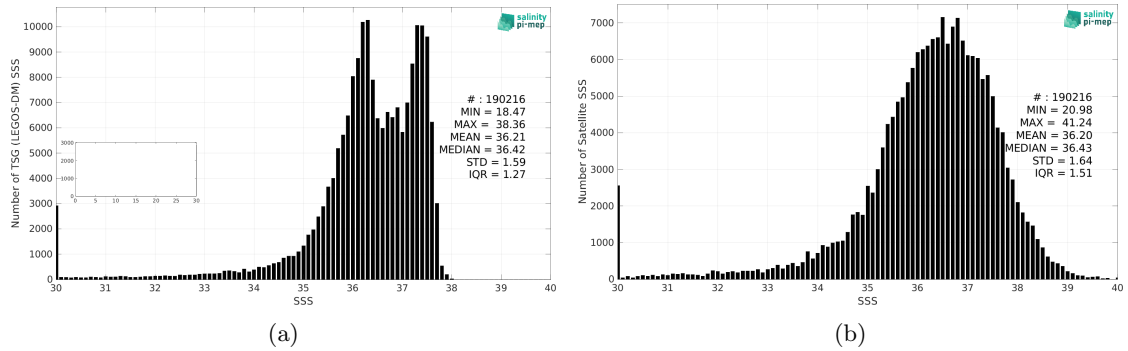
Figure 2: Histograms of SSS from TSG (LEGOS-DM) (a) and SMOS SSS L2Q v331 - With FLAG (CMEMS-CATDS-CPDC) (b) considering all match-up pairs per bins of 0.1 over the Amazon and Orinoco river plumes Pi-MEP region and for the full satellite product period.
