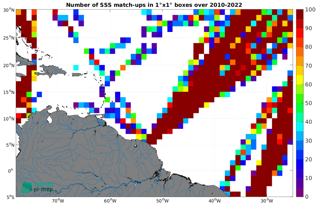
Figure 4: Number of SSS match-ups between TSG (LEGOS-DM) SSS and the SMOS SSS L2Q v331 - With FLAG (CMEMS-CATDS-CPDC) SSS product for the Amazon and Orinoco river plumes Pi-MEP region over 1^\circ \times 1^\circ boxes and for the full satellite product period.
