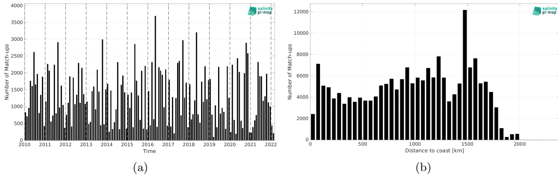
Figure 1: Number of match-ups between TSG (LEGOS-DM) and SMOS SSS L2Q v331 - With FLAG (CMEMS-CATDS-CPDC) SSS as a function of time (a) and as function of the distance to coast (b) over the Amazon and Orinoco river plumes Pi-MEP region and for the full satellite product period.
