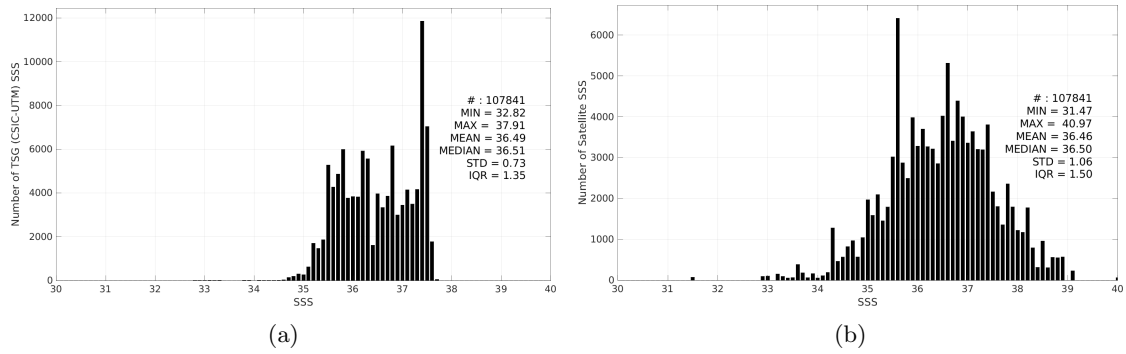
Figure 3: Histograms of SSS from TSG (CSIC-UTM) (a) and SMOS SSS L2Q v331 - With FLAG (CMEMS-CATDS-CPDC) (b) considering all match-up pairs per bins of 0.1 over the Amazon and Orinoco river plumes Pi-MEP region and for the full satellite product period.
