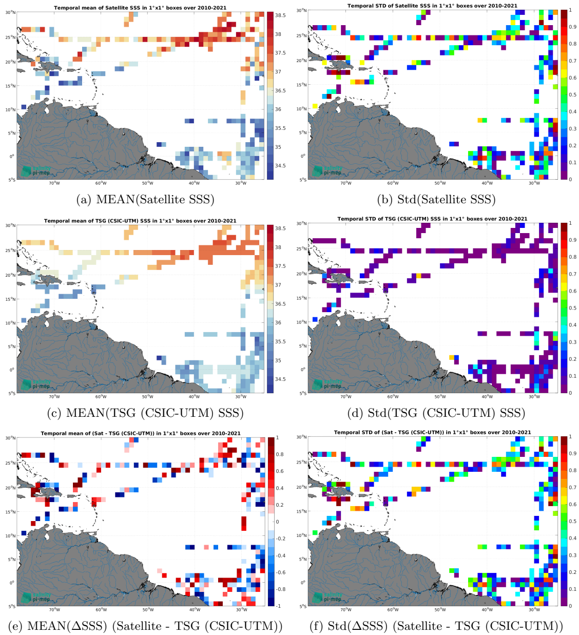
Figure 7: Temporal mean (left) and Std (right) of SSS from SMOS SSS L2Q v331 - With FLAG (CMEMS-CATDS-CPDC) (top), TSG (CSIC-UTM) (middle), and of \Delta SSS (Satellite - TSG (CSIC-UTM)). Only match-up pairs are used to generate these maps.
