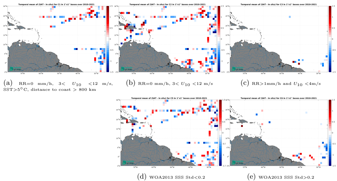
Figure 14: Temporal mean gridded over spatial boxes of size 1^\circ \times 1^\circ of \Delta SSS (SMOS SSS L2Q v331 - With FLAG (CMEMS-CATDS-CPDC) - TSG (CSIC-UTM)) for 5 different subdatasets corresponding to:RR=0 mm/h, 3 < U_{10} < 12 m/s, SST >5^\circ\text{C} , distance to coast > 800 km (a), RR=0 mm/h, 3 < U_{10} < 12 m/s (b), RR >1 mm/h and U_{10} < 4 m/s (c), WOA2013 SSS Std <0.2 (d), WOA2013 SSS Std >0.2 (e).
