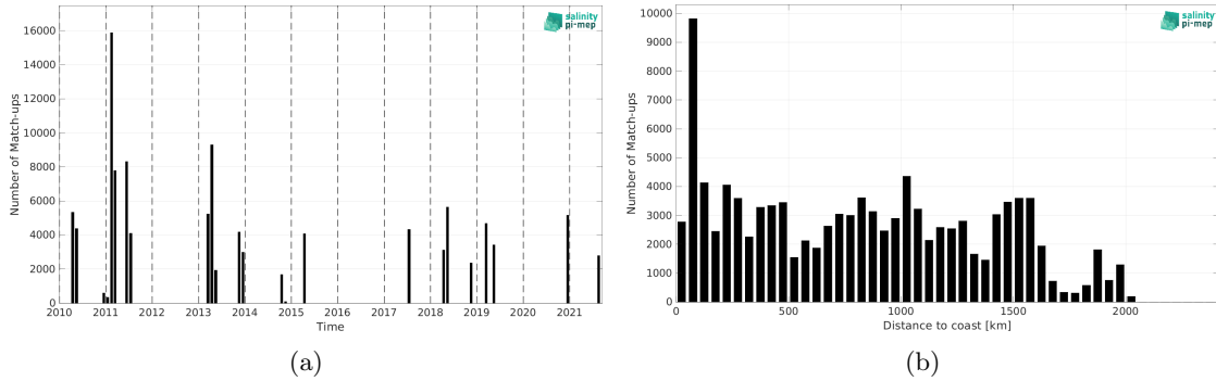
Figure 2: Number of match-ups between TSG (CSIC-UTM) and SMOS SSS L2Q v331 - With FLAG (CMEMS-CATDS-CPDC) SSS as a function of time (a) and as function of the distance to coast (b) over the Amazon and Orinoco river plumes Pi-MEP region and for the full satellite product period.
