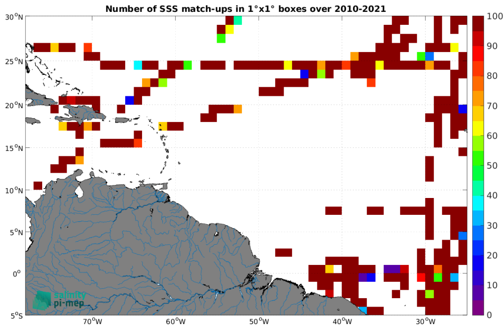
Figure 5: Number of SSS match-ups between TSG (CSIC-UTM) SSS and the SMOS SSS L2Q v331 - With FLAG (CMEMS-CATDS-CPDC) SSS product for the Amazon and Orinoco river plumes Pi-MEP region over 1^\circ \times 1^\circ boxes and for the full satellite product period.
