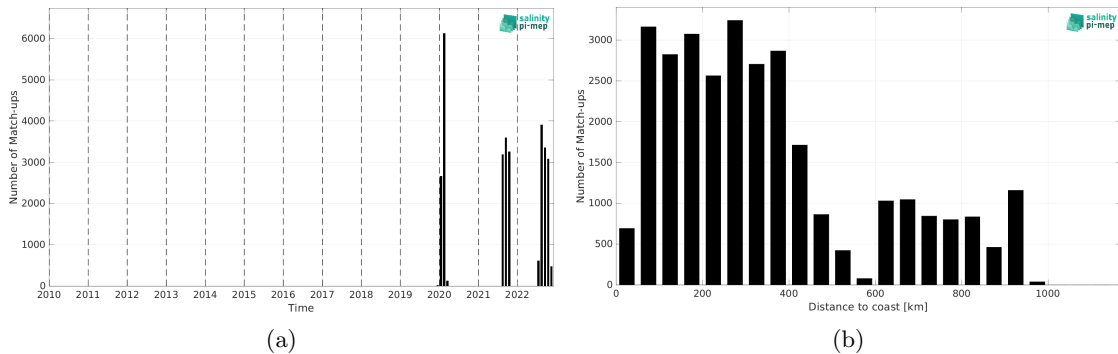
Figure 2: Number of match-ups between Saildrone and SMOS SSS L2Q v331 - With FLAG (CMEMS-CATDS-CPDC) SSS as a function of time (a) and as function of the distance to coast (b) over the Amazon and Orinoco river plumes Pi-MEP region and for the full satellite product period.
