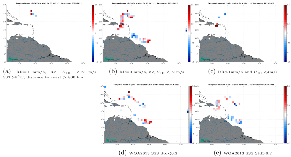
Figure 14: Temporal mean gridded over spatial boxes of size 1^\circ \times 1^\circ of \Delta SSS (SMOS SSS L2Q v331 - With FLAG (CMEMS-CATDS-CPDC) - Saildrone) for 5 different subdatasets corresponding to:RR=0 mm/h, 3 < U_{10} < 12 m/s, SST >5^\circ\text{C} , distance to coast > 800 km (a), RR=0 mm/h, 3 < U_{10} < 12 m/s (b), RR >1 mm/h and U_{10} < 4 m/s (c), WOA2013 SSS Std <0.2 (d), WOA2013 SSS Std >0.2 (e).
