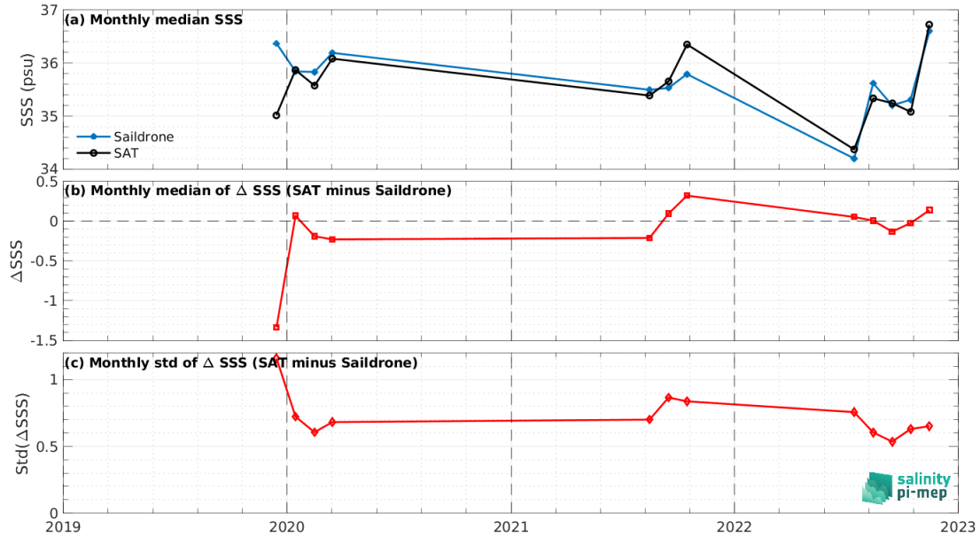
Figure 8: Time series of the monthly median SSS (top), median of \Delta SSS (Satellite - Sailldrone) and Std of \Delta SSS (Satellite - Sailldrone) over the Amazon and Orinoco river plumes Pi-MEP region considering all match-ups collected by the Pi-MEP.
