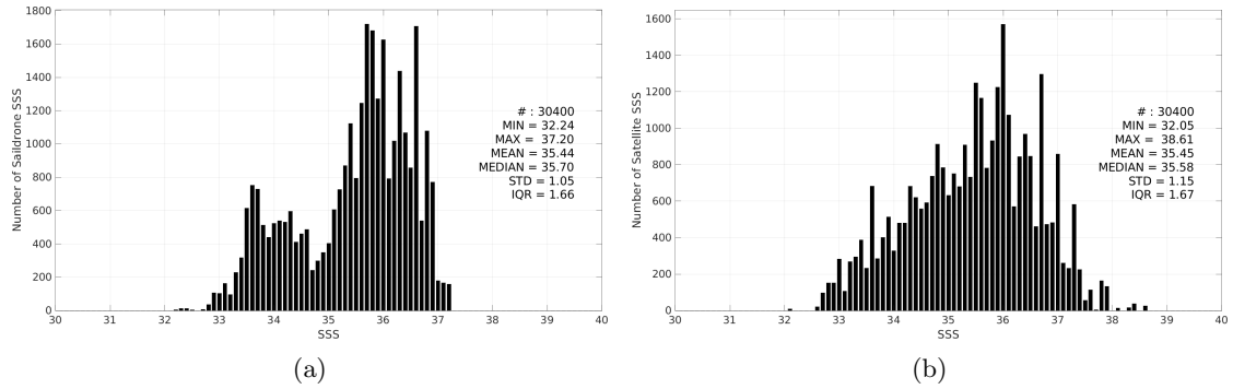
Figure 3: Histograms of SSS from Saildrone (a) and SMOS SSS L2Q v331 - With FLAG (CMEMS-CATDS-CPDC) (b) considering all match-up pairs per bins of 0.1 over the Amazon and Orinoco river plumes Pi-MEP region and for the full satellite product period.
