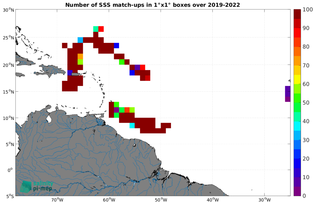
Figure 5: Number of SSS match-ups between Saildrone SSS and the SMOS SSS L2Q v331 - With FLAG (CMEMS-CATDS-CPDC) SSS product for the Amazon and Orinoco river plumes Pi-MEP region over 1^\circ \times 1^\circ boxes and for the full satellite product period.
