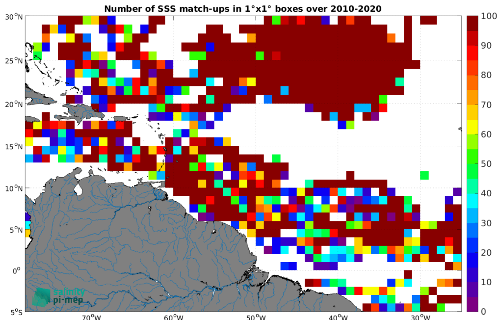
Figure 4: Number of SSS match-ups between Surface drifters SSS and the SMOS SSS L2Q v331 - With FLAG (CMEMS-CATDS-CPDC) SSS product for the Amazon and Orinoco river plumes Pi-MEP region over 1^\circ \times 1^\circ boxes and for the full satellite product period.
