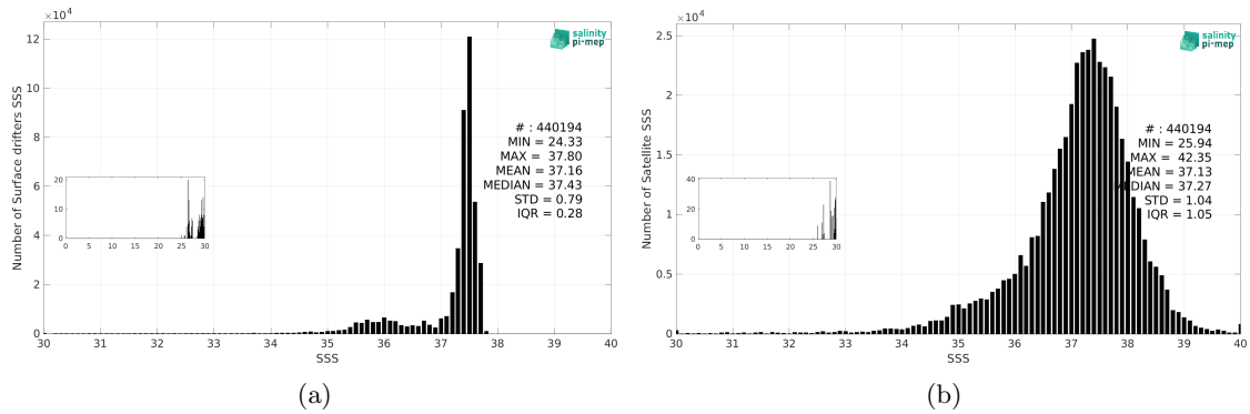
Figure 3: Histograms of SSS from Surface drifters (a) and SMOS SSS L2Q v331 - With FLAG (CMEMS-CATDS-CPDC) (b) considering all match-up pairs per bins of 0.1 over the Amazon and Orinoco river plumes Pi-MEP region and for the full satellite product period.
