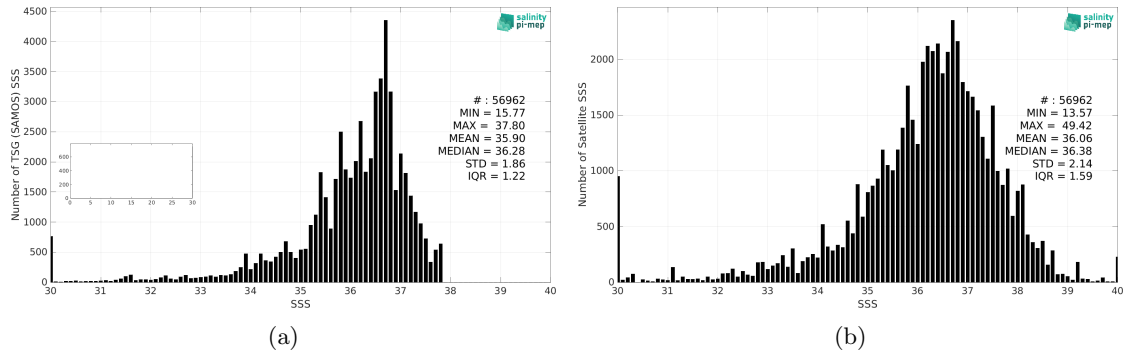
Figure 2: Histograms of SSS from TSG (SAMOS) (a) and SMOS SSS L2Q v331 - No FLAG (CMEMS-CATDS-CPDC) (b) considering all match-up pairs per bins of 0.1 over the Amazon and Orinoco river plumes Pi-MEP region and for the full satellite product period.
