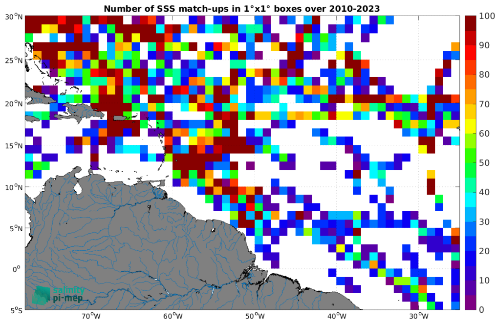
Figure 4: Number of SSS match-ups between TSG (SAMOS) SSS and the SMOS SSS L2Q v331 - No FLAG (CMEMS-CATDS-CPDC) SSS product for the Amazon and Orinoco river plumes Pi-MEP region over 1^\circ \times 1^\circ boxes and for the full satellite product period.
