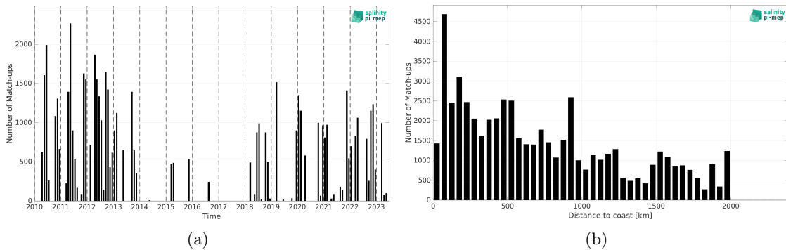
Figure 1: Number of match-ups between TSG (SAMOS) and SMOS SSS L2Q v331 - No FLAG (CMEMS-CATDS-CPDC) SSS as a function of time (a) and as function of the distance to coast (b) over the Amazon and Orinoco river plumes Pi-MEP region and for the full satellite product period.
