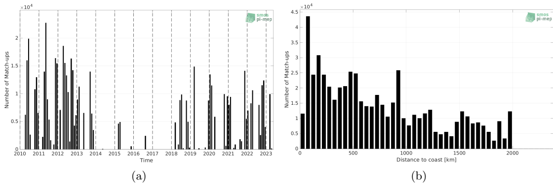
Figure 1: Number of match-ups between TSG (SAMOS) and SMOS SSS L2Q v331 - No FLAG (CMEMS-CATDS-CPDC) SSS as a function of time (a) and as function of the distance to coast (b) over the Amazon and Orinoco river plumes Pi-MEP region and for the full satellite product period.
