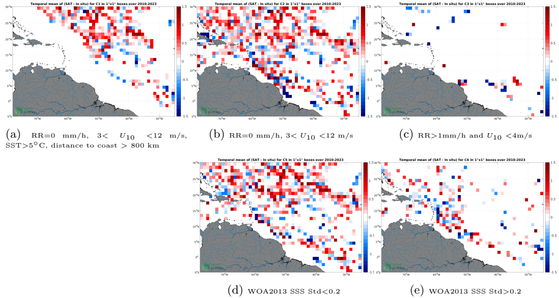
Figure 12: Temporal mean gridded over spatial boxes of size 1^{\circ}\times 1^{\circ} of \Delta\text{SSS} (SMOS SSS L2Q v331 - No FLAG (CMEMS-CATDS-CPDC) - TSG (SAMOS)) for 5 different subdatasets corresponding to:RR=0 mm/h, 3 < U_{10} < 12 m/s, SST >5^{\circ}\text{C} , distance to coast > 800 km (a), RR=0 mm/h, 3 < U_{10} < 12 m/s (b), RR >1 mm/h and U_{10} < 4 m/s (c), WOA2013 SSS Std <0.2 (d), WOA2013 SSS Std >0.2 (e).
