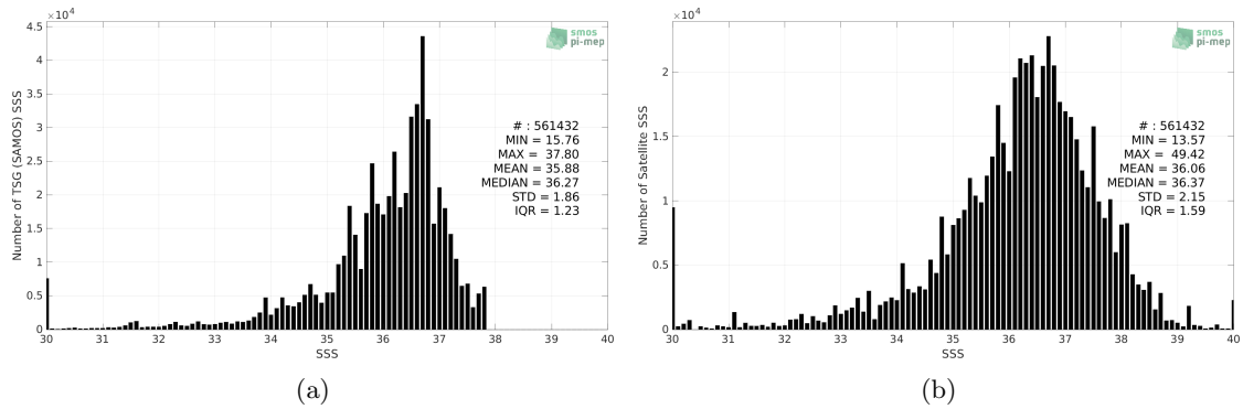
Figure 2: Histograms of SSS from TSG (SAMOS) (a) and SMOS SSS L2Q v331 - No FLAG (CMEMS-CATDS-CPDC) (b) considering all match-up pairs per bins of 0.1 over the Amazon and Orinoco river plumes Pi-MEP region and for the full satellite product period.
