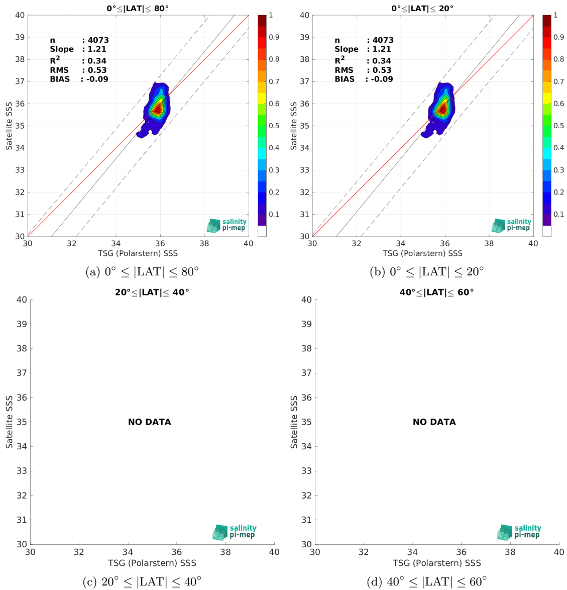
Figure 10: Contour maps of the concentration of SMOS SSS L2Q v331 - No FLAG (CMEMS-CATDS-CPDC) SSS (y-axis) versus TSG (Polarstern) SSS (x-axis) at match-up pairs for different latitude bands. For each plot, the red line shows x=y . The black thin and dashed lines indicate a linear fit through the data cloud and the \pm 95\% confidence levels, respectively. The number match-up pairs n , the slope and R^2 coefficient of the linear fit, the root mean square (RMS) and the mean bias between satellite and in situ data are indicated for each latitude band in each plots.
