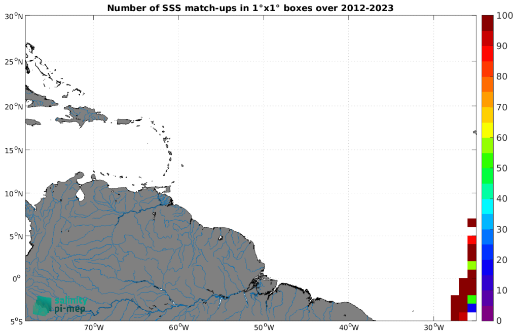
Figure 5: Number of SSS match-ups between TSG (Polarstern) SSS and the SMOS SSS L2Q v331 - No FLAG (CMEMS-CATDS-CPDC) SSS product for the Amazon and Orinoco river plumes Pi-MEP region over 1^\circ \times 1^\circ boxes and for the full satellite product period.
