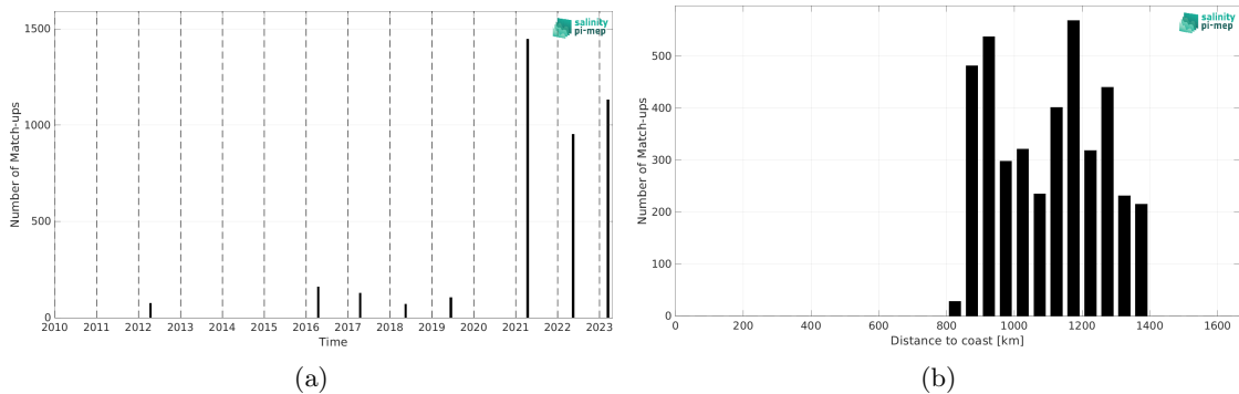
Figure 2: Number of match-ups between TSG (Polarstern) and SMOS SSS L2Q v331 - No FLAG (CMEMS-CATDS-CPDC) SSS as a function of time (a) and as function of the distance to coast (b) over the Amazon and Orinoco river plumes Pi-MEP region and for the full satellite product period.
