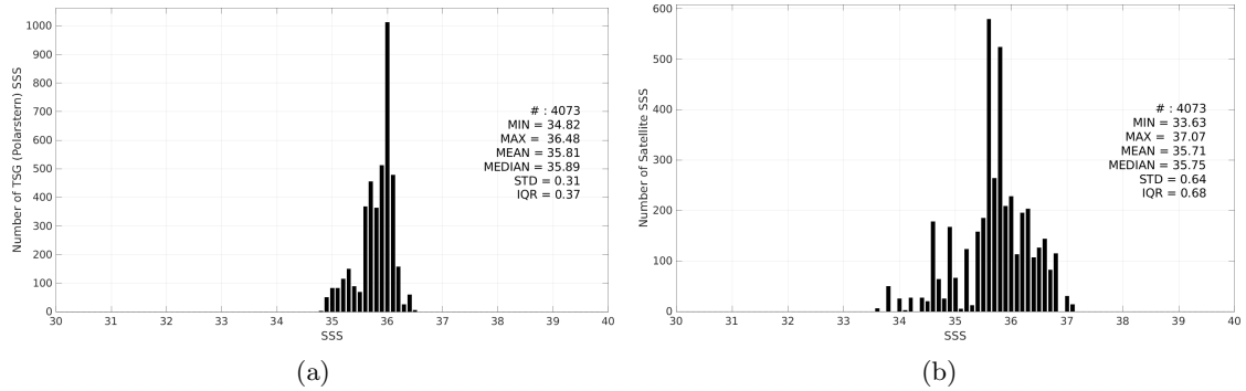
Figure 3: Histograms of SSS from TSG (Polarstern) (a) and SMOS SSS L2Q v331 - No FLAG (CMEMS-CATDS-CPDC) (b) considering all match-up pairs per bins of 0.1 over the Amazon and Orinoco river plumes Pi-MEP region and for the full satellite product period.
