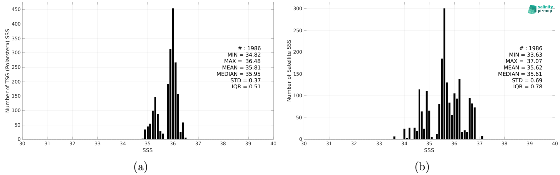
Figure 2: Histograms of SSS from TSG (Polarstern) (a) and SMOS SSS L2Q v331 - No FLAG (CMEMS-CATDS-CPDC) (b) considering all match-up pairs per bins of 0.1 over the Amazon and Orinoco river plumes Pi-MEP region and for the full satellite product period.
