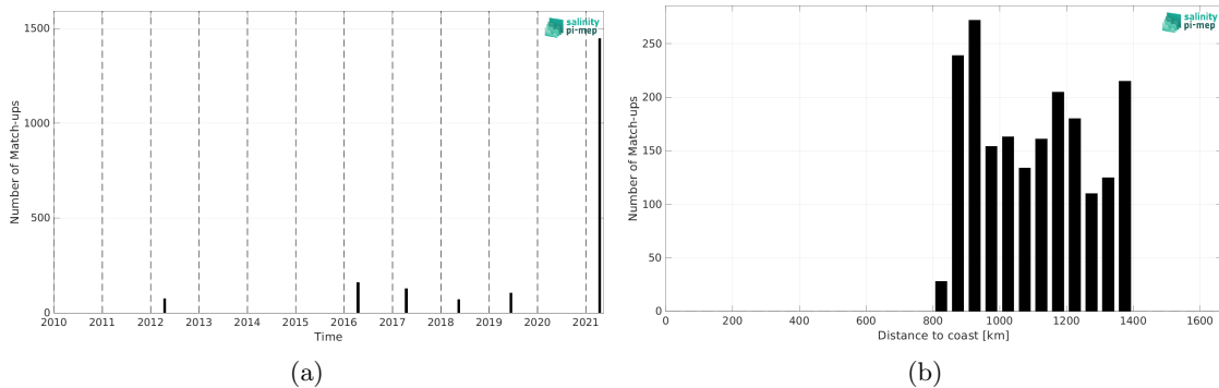
Figure 1: Number of match-ups between TSG (Polarstern) and SMOS SSS L2Q v331 - No FLAG (CMEMS-CATDS-CPDC) SSS as a function of time (a) and as function of the distance to coast (b) over the Amazon and Orinoco river plumes Pi-MEP region and for the full satellite product period.
