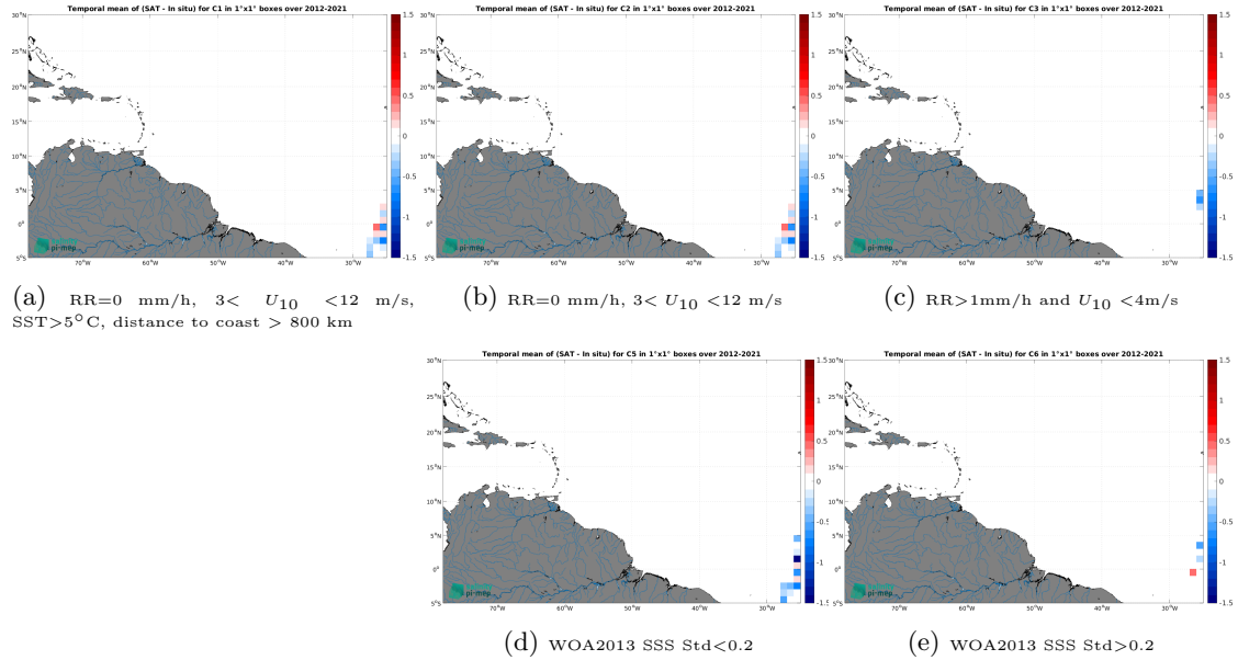
Figure 12: Temporal mean gridded over spatial boxes of size 1^{\circ}\times 1^{\circ} of \Delta\text{SSS} (SMOS SSS L2Q v331 - No FLAG (CMEMS-CATDS-CPDC) - TSG (Polarstern)) for 5 different subdatasets corresponding to:RR=0 mm/h, 3 < U_{10} < 12 m/s, SST >5^{\circ}\text{C} , distance to coast > 800 km (a), RR=0 mm/h, 3 < U_{10} < 12 m/s (b), RR >1 mm/h and U_{10} < 4 m/s (c), WOA2013 SSS Std <0.2 (d), WOA2013 SSS Std >0.2 (e).
