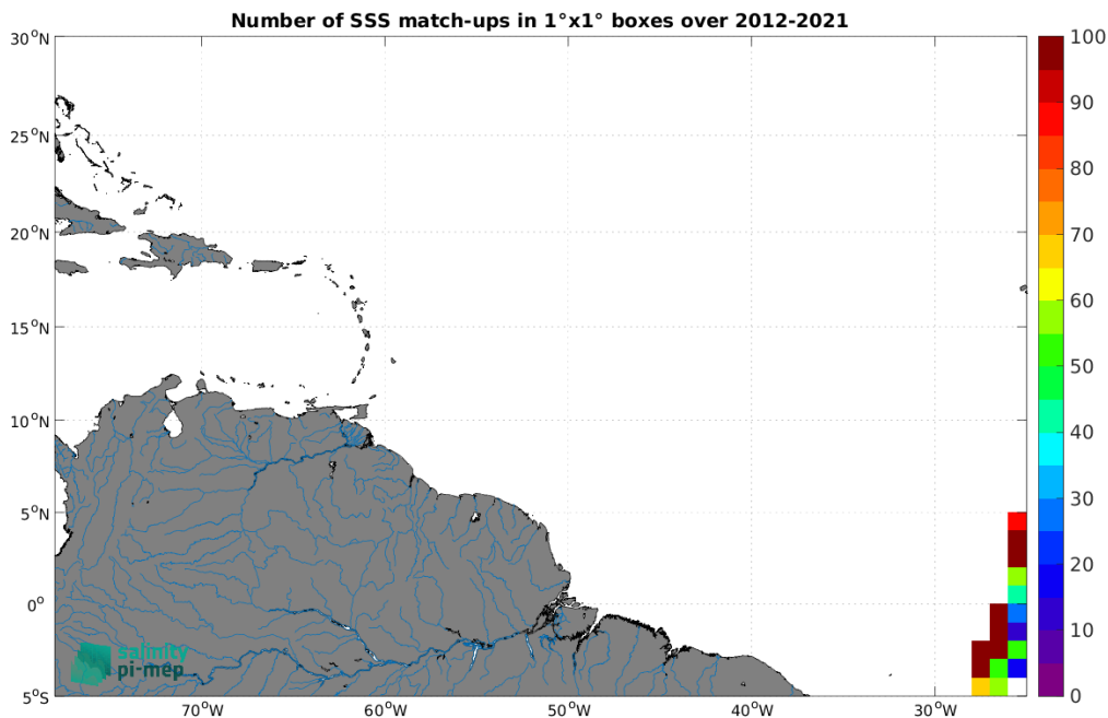
Figure 4: Number of SSS match-ups between TSG (Polarstern) SSS and the SMOS SSS L2Q v331 - No FLAG (CMEMS-CATDS-CPDC) SSS product for the Amazon and Orinoco river plumes Pi-MEP region over 1^\circ \times 1^\circ boxes and for the full satellite product period.
