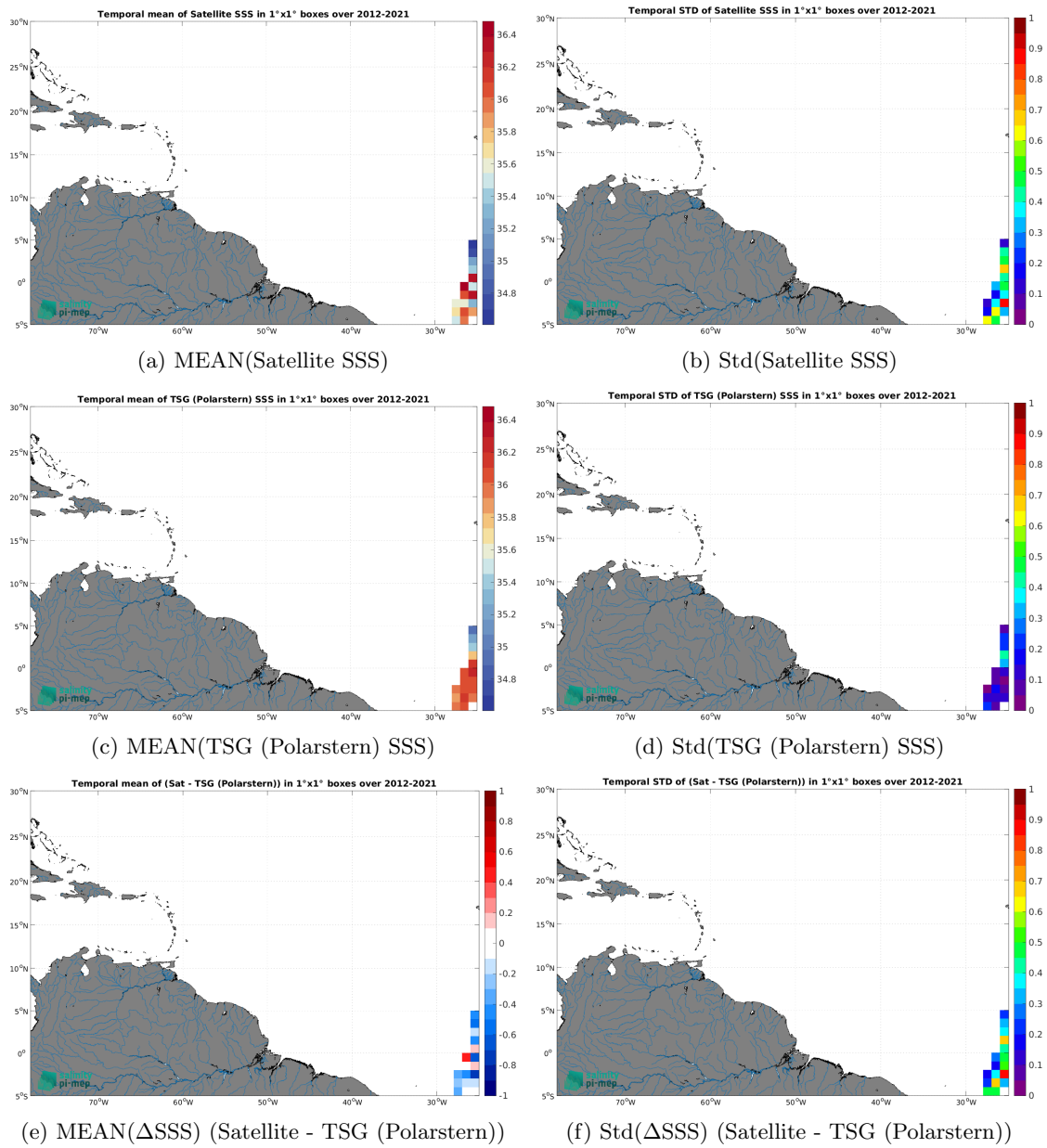
Figure 6: Temporal mean (left) and Std (right) of SSS from SMOS SSS L2Q v331 - No FLAG (CMEMS-CATDS-CPDC) (top), TSG (Polarstern) (middle), and of \Delta SSS (Satellite - TSG (Polarstern)). Only match-up pairs are used to generate these maps.
