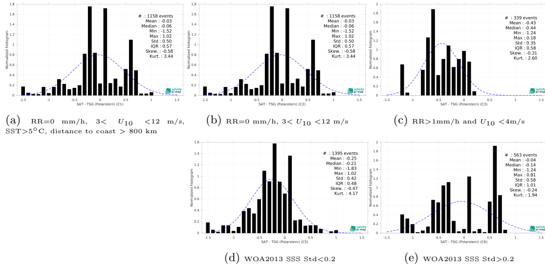
Figure 13: Normalized histogram of \Delta SSS (SMOS SSS L2Q v331 - No FLAG (CMEMS-CATDS-CPDC) - TSG (Polarstern)) for 5 different subdatasets corresponding to: RR=0 mm/h, 3 < U_{10} < 12 m/s, SST>5°C, distance to coast > 800 km (a), RR=0 mm/h, 3 < U_{10} < 12 m/s (b), RR>1mm/h and U_{10} < 4 m/s (c), WOA2013 SSS Std<0.2 (d), WOA2013 SSS Std>0.2 (e).
