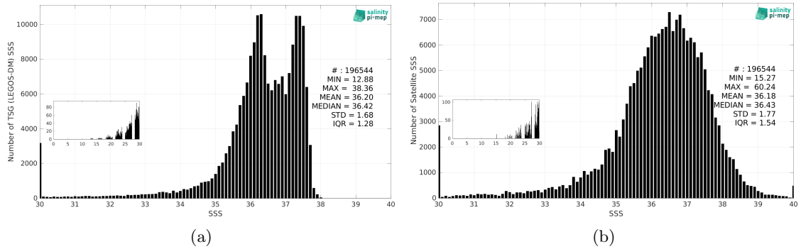
Figure 3: Histograms of SSS from TSG (LEGOS-DM) (a) and SMOS SSS L2Q v331 - No FLAG (CMEMS-CATDS-CPDC) (b) considering all match-up pairs per bins of 0.1 over the Amazon and Orinoco river plumes Pi-MEP region and for the full satellite product period.
