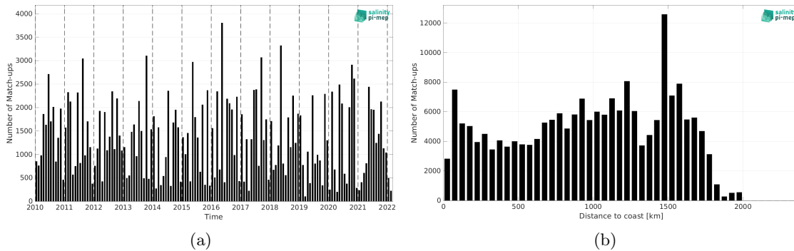
Figure 2: Number of match-ups between TSG (LEGOS-DM) and SMOS SSS L2Q v331 - No FLAG (CMEMS-CATDS-CPDC) SSS as a function of time (a) and as function of the distance to coast (b) over the Amazon and Orinoco river plumes Pi-MEP region and for the full satellite product period.
