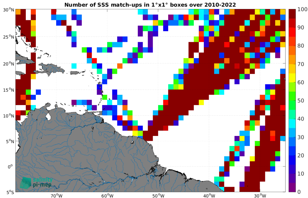
Figure 5: Number of SSS match-ups between TSG (LEGOS-DM) SSS and the SMOS SSS L2Q v331 - No FLAG (CMEMS-CATDS-CPDC) SSS product for the Amazon and Orinoco river plumes Pi-MEP region over 1^\circ \times 1^\circ boxes and for the full satellite product period.
