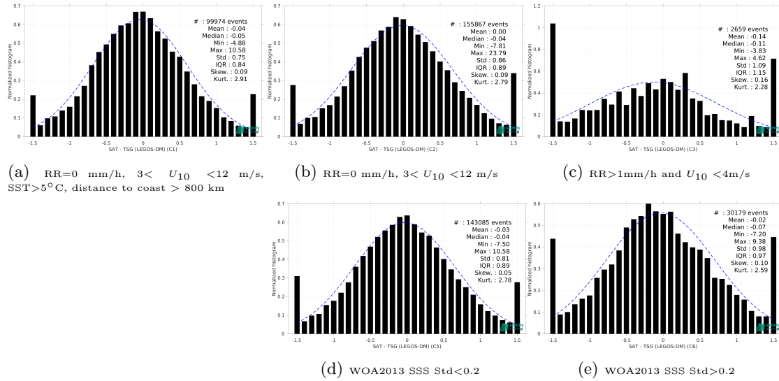
Figure 13: Normalized histogram of \Delta\text{SSS} (SMOS SSS L2Q v331 - No FLAG (CMEMS-CATDS-CPDC) - TSG (LEGOS-DM)) for 5 different subdatasets corresponding to: RR=0 mm/h, 3 < U_{10} < 12 m/s, SST > 5^\circ\text{C} , distance to coast > 800 km (a), RR=0 mm/h, 3 < U_{10} < 12 m/s (b), RR > 1 mm/h and U_{10} < 4 m/s (c), WOA2013 SSS Std < 0.2 (d), WOA2013 SSS Std > 0.2 (e).
