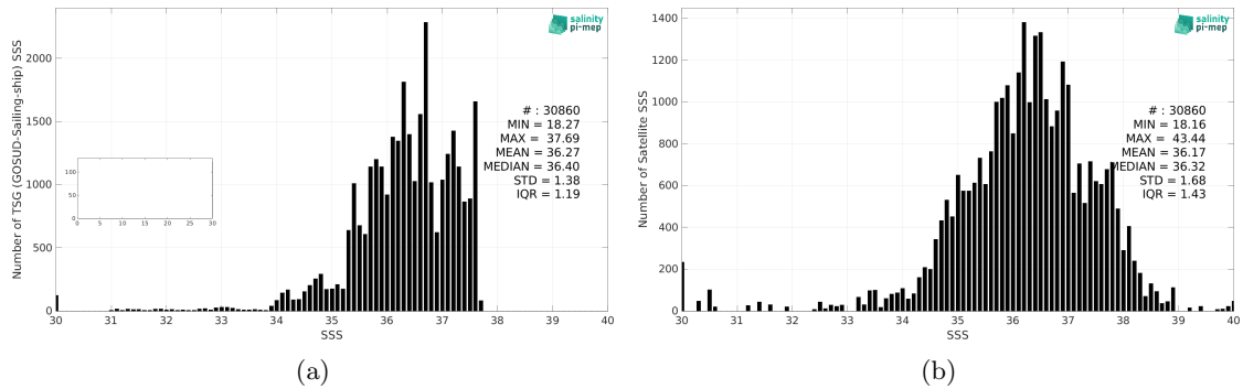
Figure 2: Histograms of SSS from TSG (GOSUD-Sailing-ship) (a) and SMOS SSS L2Q v331 - No FLAG (CMEMS-CATDS-CPDC) (b) considering all match-up pairs per bins of 0.1 over the Amazon and Orinoco river plumes Pi-MEP region and for the full satellite product period.
