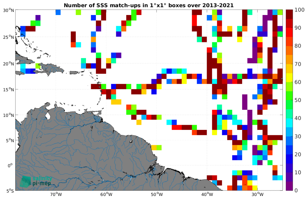
Figure 4: Number of SSS match-ups between TSG (GOSUD-Sailing-ship) SSS and the SMOS SSS L2Q v331 - No FLAG (CMEMS-CATDS-CPDC) SSS product for the Amazon and Orinoco river plumes Pi-MEP region over 1^\circ \times 1^\circ boxes and for the full satellite product period.
