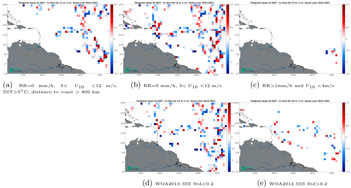
Figure 12: Temporal mean gridded over spatial boxes of size 1^{\circ}\times 1^{\circ} of \Delta SSS (SMOS SSS L2Q v331 - No FLAG (CMEMS-CATDS-CPDC) - TSG (GOSUD-Sailing-ship)) for 5 different sub-datasets corresponding to:RR=0 mm/h, 3 < U_{10} < 12 m/s, SST >5^{\circ}\text{C} , distance to coast > 800 km (a), RR=0 mm/h, 3 < U_{10} < 12 m/s (b), RR >1 mm/h and U_{10} < 4 m/s (c), WOA2013 SSS Std <0.2 (d), WOA2013 SSS Std >0.2 (e).
