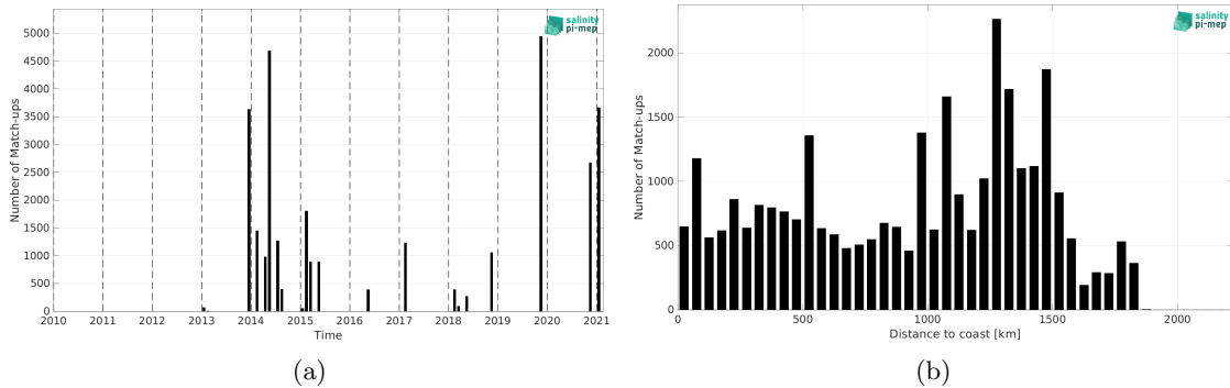
Figure 1: Number of match-ups between TSG (GOSUD-Sailing-ship) and SMOS SSS L2Q v331 - No FLAG (CMEMS-CATDS-CPDC) SSS as a function of time (a) and as function of the distance to coast (b) over the Amazon and Orinoco river plumes Pi-MEP region and for the full satellite product period.
