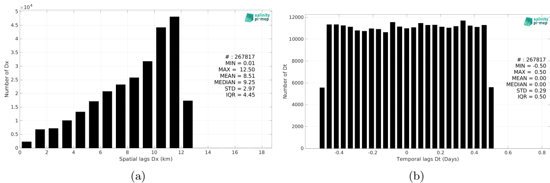
Figure 6: Histograms of the spatial (a) and temporal (b) lags between the location/time of the TSG (GOSUD-Research-vessel) measurement and the date of the corresponding SMOS SSS L2Q v331 - No FLAG (CMEMS-CATDS-CPDC) SSS pixel.
