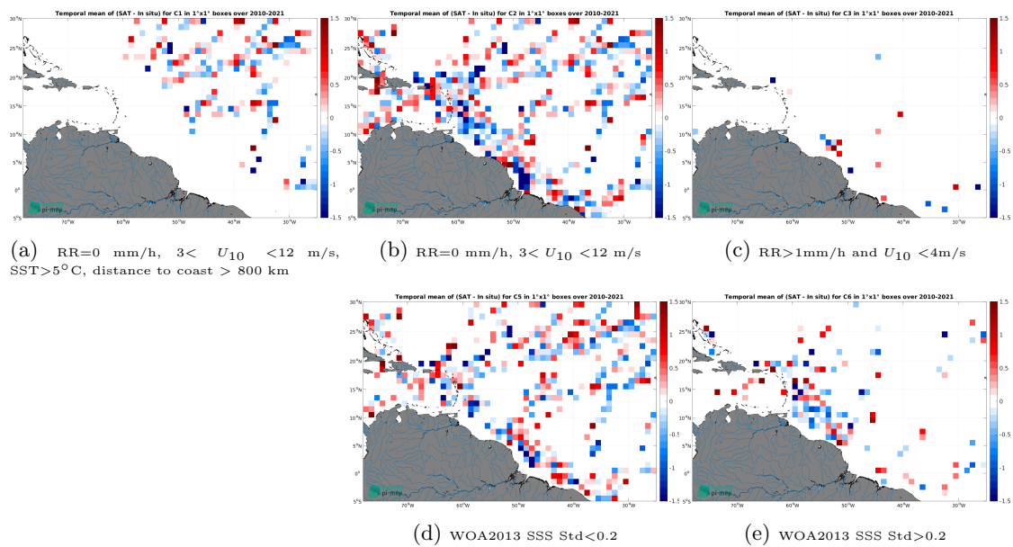
Figure 14: Temporal mean gridded over spatial boxes of size 1^\circ \times 1^\circ of \Delta SSS (SMOS SSS L2Q v331 - No FLAG (CMEMS-CATDS-CPDC) - TSG (GOSUD-Research-vessel)) for 5 different subdatasets corresponding to:RR=0 mm/h, 3 < U_{10} < 12 m/s, SST >5^\circ C, distance to coast > 800 km (a), RR=0 mm/h, 3 < U_{10} < 12 m/s (b), RR >1 mm/h and U_{10} < 4 m/s (c), WOA2013 SSS Std <0.2 (d), WOA2013 SSS Std >0.2 (e).
