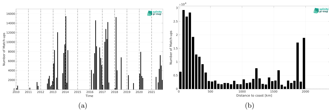
Figure 2: Number of match-ups between TSG (GOSUD-Research-vessel) and SMOS SSS L2Q v331 - No FLAG (CMEMS-CATDS-CPDC) SSS as a function of time (a) and as function of the distance to coast (b) over the Amazon and Orinoco river plumes Pi-MEP region and for the full satellite product period.
