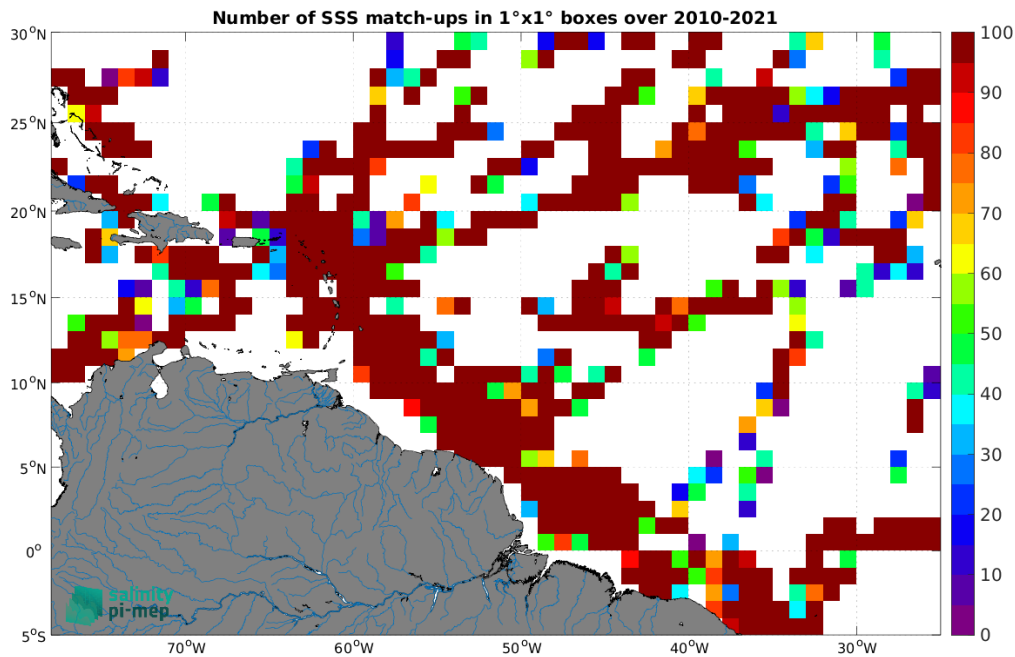
Figure 5: Number of SSS match-ups between TSG (GOSUD-Research-vessel) SSS and the SMOS SSS L2Q v331 - No FLAG (CMEMS-CATDS-CPDC) SSS product for the Amazon and Orinoco river plumes Pi-MEP region over 1^{\circ} \times 1^{\circ} boxes and for the full satellite product period.
