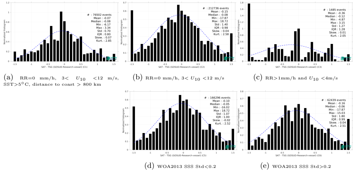
Figure 15: Normalized histogram of \Delta SSS (SMOS SSS L2Q v331 - No FLAG (CMEMS-CATDS-CPDC) - TSG (GOSUD-Research-vessel)) for 5 different subdatasets corresponding to: RR=0 mm/h, 3 < U_{10} < 12 m/s, SST > 5°C, distance to coast > 800 km (a), RR=0 mm/h, 3 < U_{10} < 12 m/s (b), RR > 1mm/h and U_{10} < 4 m/s (c), WOA2013 SSS Std < 0.2 (d), WOA2013 SSS Std > 0.2 (e).
