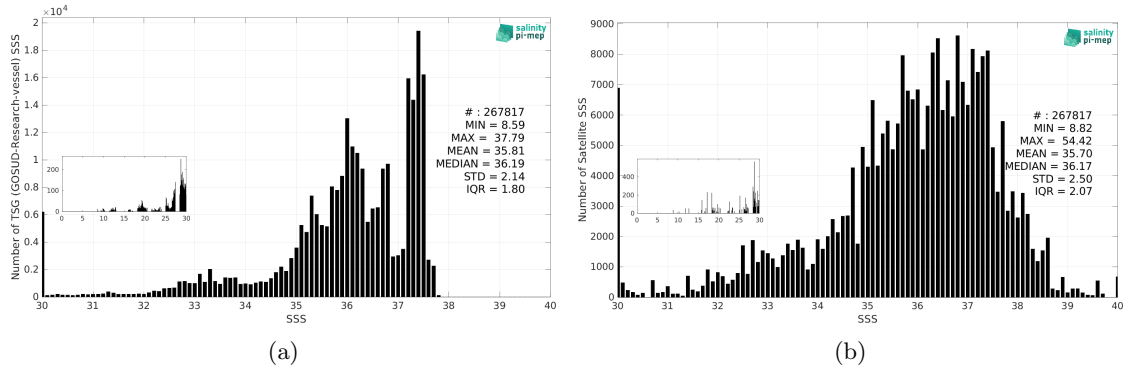
Figure 3: Histograms of SSS from TSG (GOSUD-Research-vessel) (a) and SMOS SSS L2Q v331 - No FLAG (CMEMS-CATDS-CPDC) (b) considering all match-up pairs per bins of 0.1 over the Amazon and Orinoco river plumes Pi-MEP region and for the full satellite product period.
