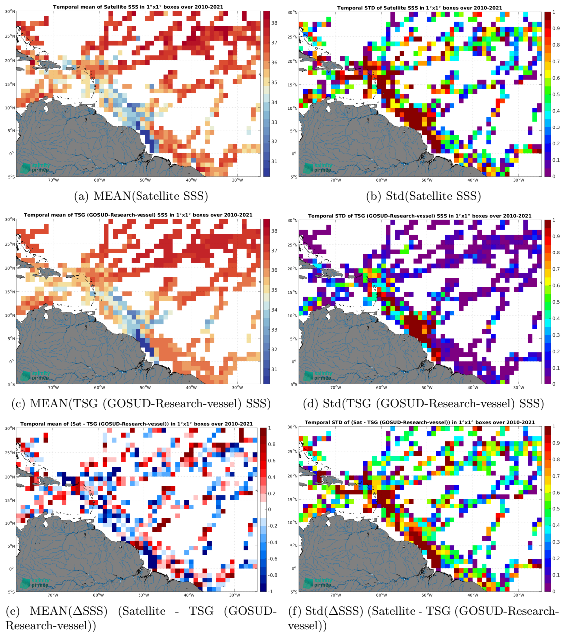
Figure 7: Temporal mean (left) and Std (right) of SSS from SMOS SSS L2Q v331 - No FLAG (CMEMS-CATDS-CPDC) (top), TSG (GOSUD-Research-vessel) (middle), and of \Delta SSS (Satellite - TSG (GOSUD-Research-vessel)). Only match-up pairs are used to generate these maps.
