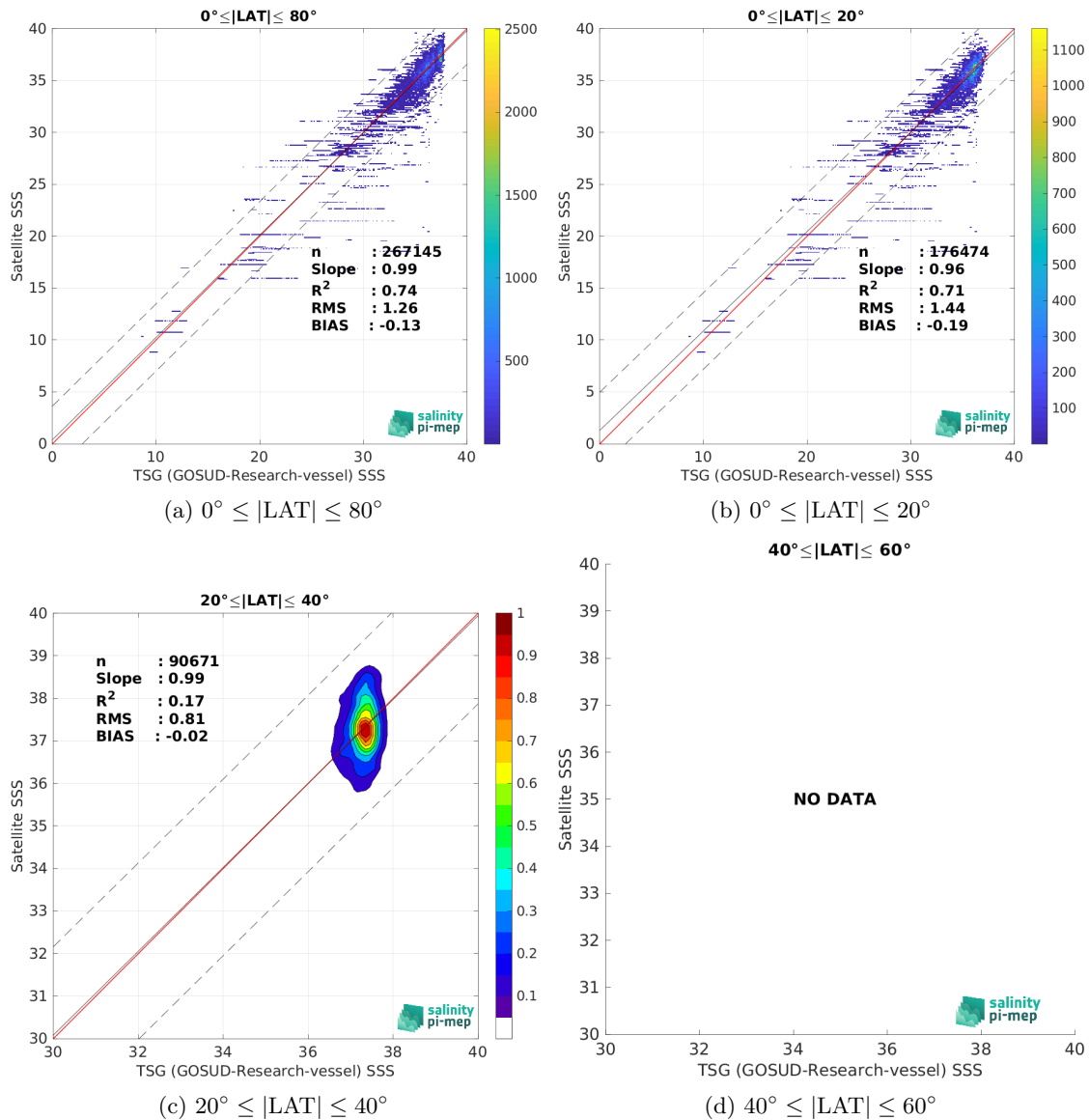
Figure 10: Contour maps of the concentration of SMOS SSS L2Q v331 - No FLAG (CMEMS-CATDS-CPDC) SSS (y-axis) versus TSG (GOSUD-Research-vessel) SSS (x-axis) at match-up pairs for different latitude bands. For each plot, the red line shows x=y . The black thin and dashed lines indicate a linear fit through the data cloud and the \pm 95\% confidence levels, respectively. The number match-up pairs n , the slope and R^2 coefficient of the linear fit, the root mean square (RMS) and the mean bias between satellite and in situ data are indicated for each latitude band in each plots.
