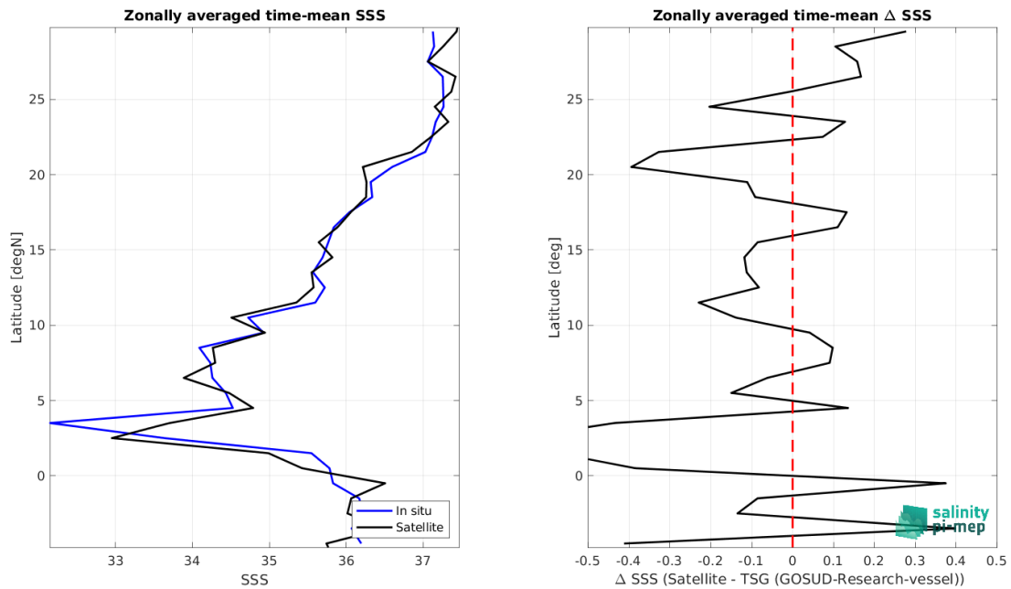
Figure 9: Left panel: Zonal mean SSS from SMOS SSS L2Q v331 - No FLAG (CMEMS-CATDS-CPDC) satellite product (black) and from TSG (GOSUD-Research-vessel) (blue). Right panel: Zonal mean of \Delta SSS (Satellite - TSG (GOSUD-Research-vessel)) for all the collected Pi-MEP match-up pairs estimated over the full satellite product period.
