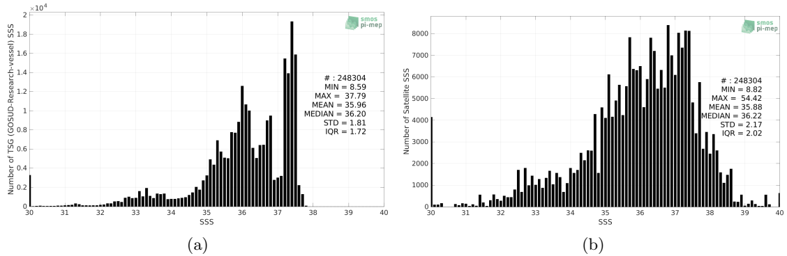
Figure 2: Histograms of SSS from TSG (GOSUD-Research-vessel) (a) and SMOS SSS L2Q v331 - No FLAG (CMEMS-CATDS-CPDC) (b) considering all match-up pairs per bins of 0.1 over the Amazon and Orinoco river plumes Pi-MEP region and for the full satellite product period.
