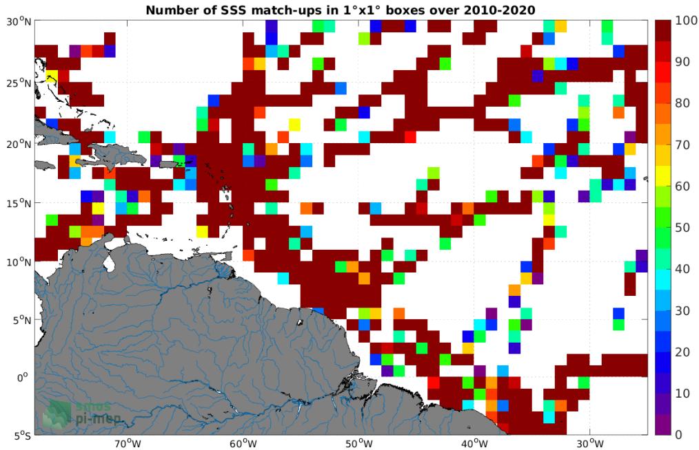
Figure 4: Number of SSS match-ups between TSG (GOSUD-Research-vessel) SSS and the SMOS SSS L2Q v331 - No FLAG (CMEMS-CATDS-CPDC) SSS product for the Amazon and Orinoco river plumes Pi-MEP region over 1^\circ \times 1^\circ boxes and for the full satellite product period.
