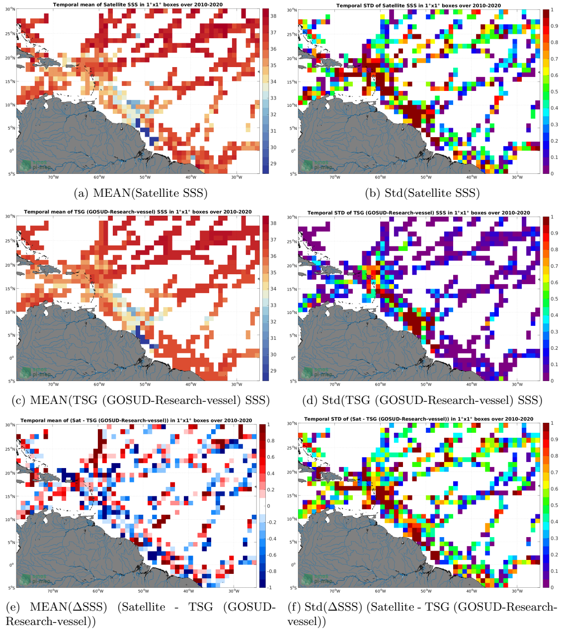
Figure 6: Temporal mean (left) and Std (right) of SSS from SMOS SSS L2Q v331 - No FLAG (CMEMS-CATDS-CPDC) (top), TSG (GOSUD-Research-vessel) (middle), and of \Delta SSS (Satellite - TSG (GOSUD-Research-vessel)). Only match-up pairs are used to generate these maps.
