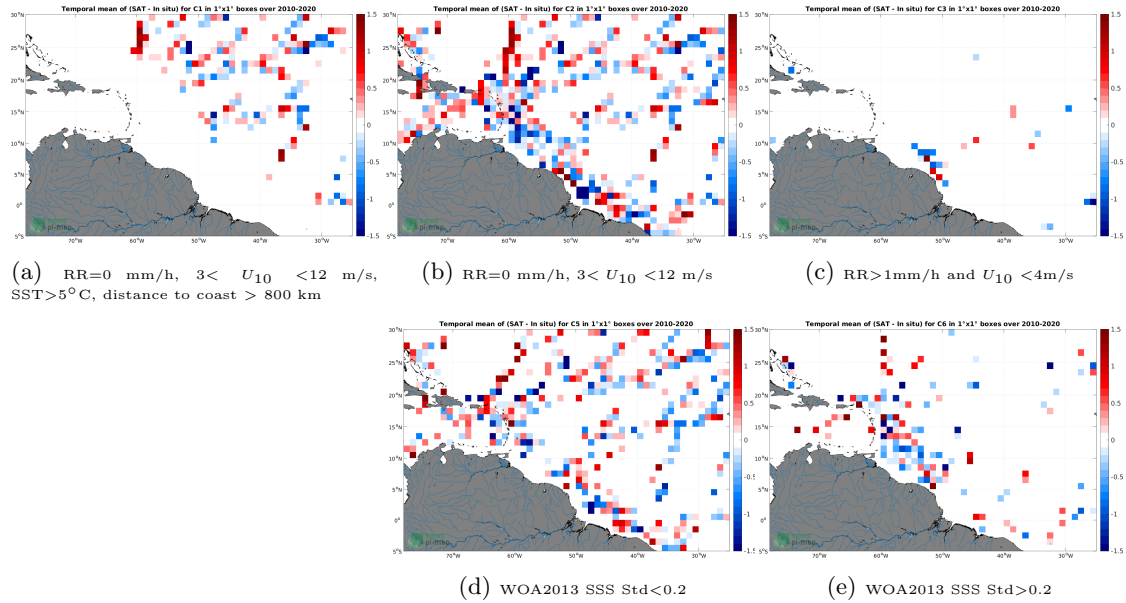
Figure 12: Temporal mean gridded over spatial boxes of size 1^{\circ}\times 1^{\circ} of \Delta SSS (SMOS SSS L2Q v331 - No FLAG (CMEMS-CATDS-CPDC) - TSG (GOSUD-Research-vessel)) for 5 different subdatasets corresponding to:RR=0 mm/h, 3 < U_{10} < 12 m/s, SST >5^{\circ}\text{C} , distance to coast > 800 km (a), RR=0 mm/h, 3 < U_{10} < 12 m/s (b), RR >1 mm/h and U_{10} < 4 m/s (c), WOA2013 SSS Std <0.2 (d), WOA2013 SSS Std >0.2 (e).
