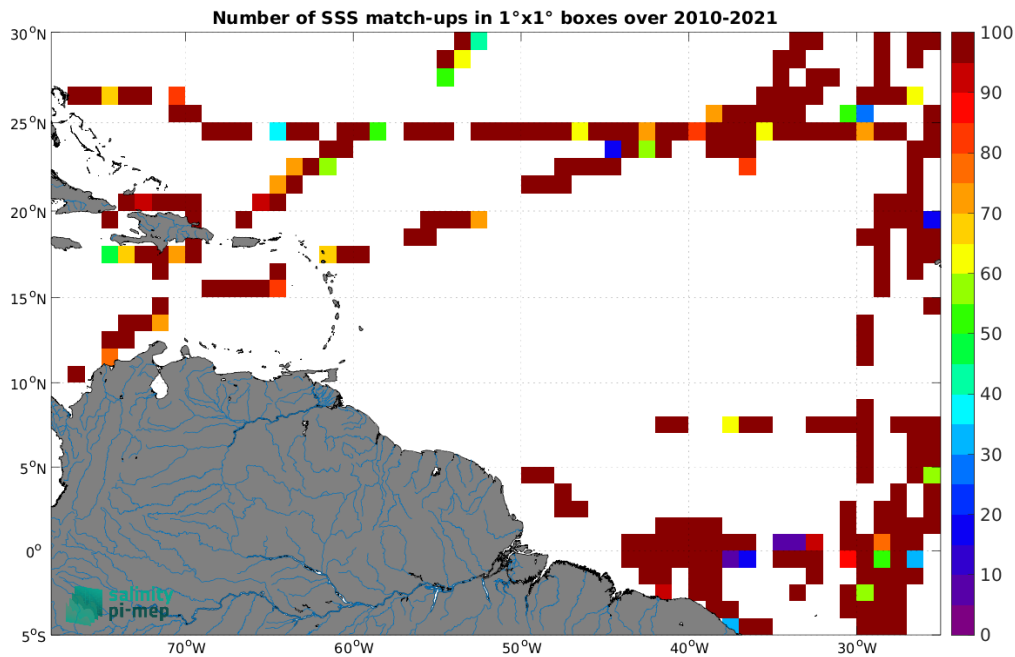
Figure 5: Number of SSS match-ups between TSG (CSIC-UTM) SSS and the SMOS SSS L2Q v331 - No FLAG (CMEMS-CATDS-CPDC) SSS product for the Amazon and Orinoco river plumes Pi-MEP region over 1^\circ \times 1^\circ boxes and for the full satellite product period.
