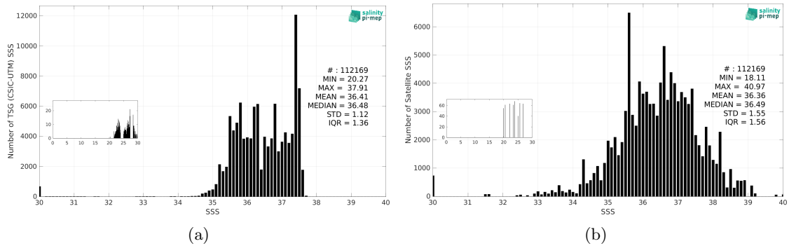
Figure 3: Histograms of SSS from TSG (CSIC-UTM) (a) and SMOS SSS L2Q v331 - No FLAG (CMEMS-CATDS-CPDC) (b) considering all match-up pairs per bins of 0.1 over the Amazon and Orinoco river plumes Pi-MEP region and for the full satellite product period.
