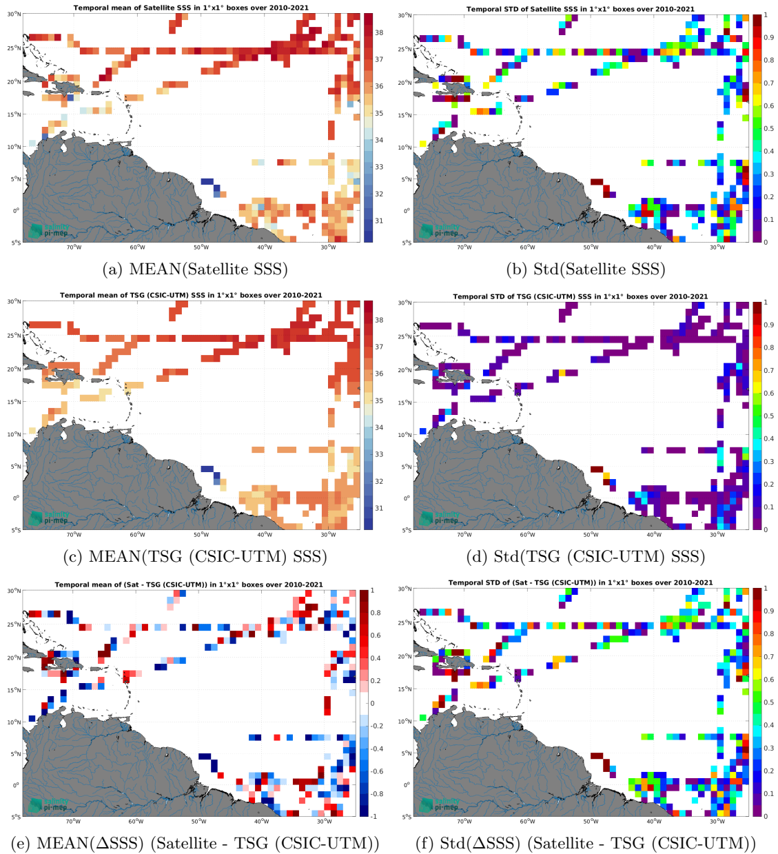
Figure 7: Temporal mean (left) and Std (right) of SSS from SMOS SSS L2Q v331 - No FLAG (CMEMS-CATDS-CPDC) (top), TSG (CSIC-UTM) (middle), and of \Delta SSS (Satellite - TSG (CSIC-UTM)). Only match-up pairs are used to generate these maps.
