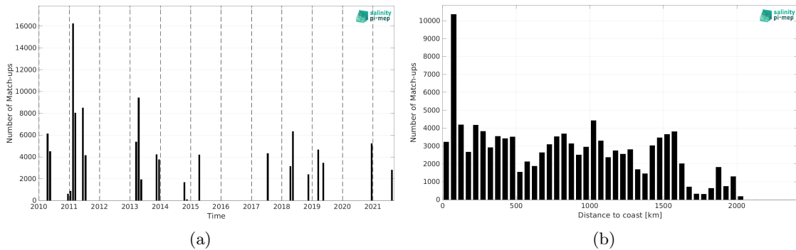
Figure 2: Number of match-ups between TSG (CSIC-UTM) and SMOS SSS L2Q v331 - No FLAG (CMEMS-CATDS-CPDC) SSS as a function of time (a) and as function of the distance to coast (b) over the Amazon and Orinoco river plumes Pi-MEP region and for the full satellite product period.
