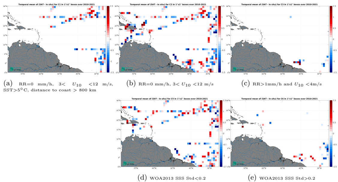
Figure 14: Temporal mean gridded over spatial boxes of size 1^\circ \times 1^\circ of \Delta SSS (SMOS SSS L2Q v331 - No FLAG (CMEMS-CATDS-CPDC) - TSG (CSIC-UTM)) for 5 different subdatasets corresponding to:RR=0 mm/h, 3 < U_{10} < 12 m/s, SST >5^\circ\text{C} , distance to coast > 800 km (a), RR=0 mm/h, 3 < U_{10} < 12 m/s (b), RR >1 mm/h and U_{10} < 4 m/s (c), WOA2013 SSS Std <0.2 (d), WOA2013 SSS Std >0.2 (e).
