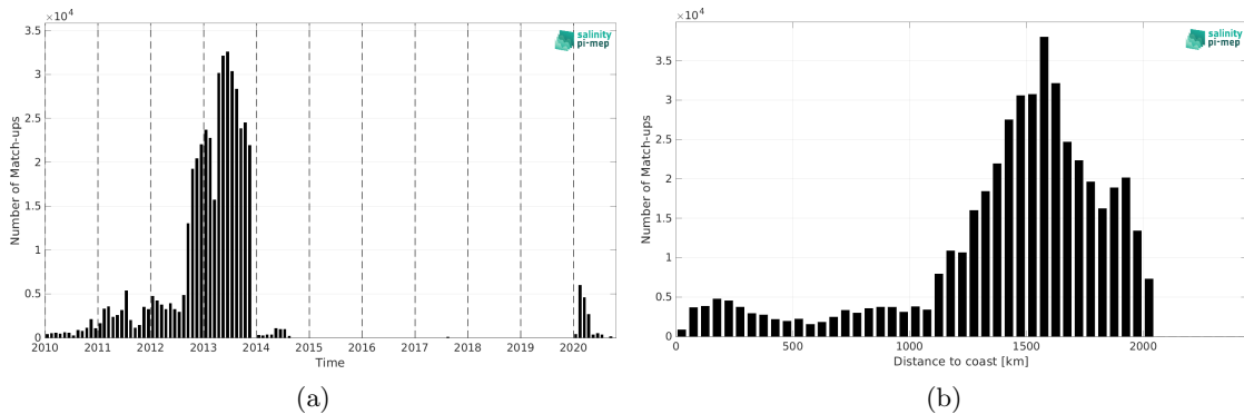
Figure 2: Number of match-ups between Surface drifters and SMOS SSS L2Q v331 - No FLAG (CMEMS-CATDS-CPDC) SSS as a function of time (a) and as function of the distance to coast (b) over the Amazon and Orinoco river plumes Pi-MEP region and for the full satellite product period.
