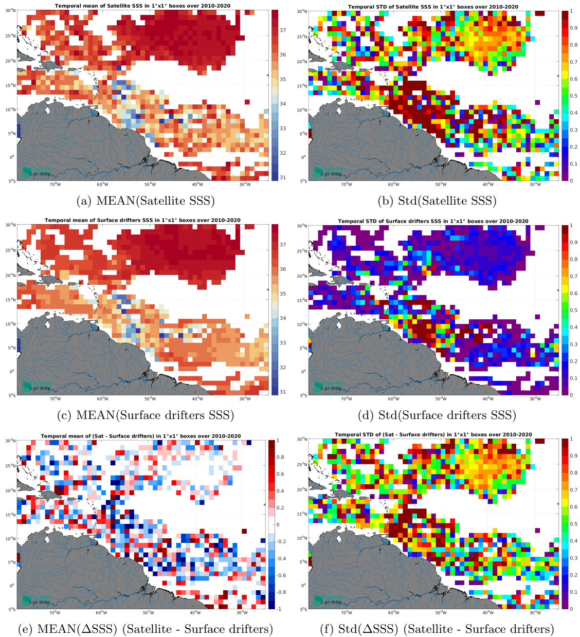
Figure 6: Temporal mean (left) and Std (right) of SSS from SMOS SSS L2Q v331 - No FLAG (CMEMS-CATDS-CPDC) (top), Surface drifters (middle), and of \Delta SSS (Satellite - Surface drifters). Only match-up pairs are used to generate these maps.
