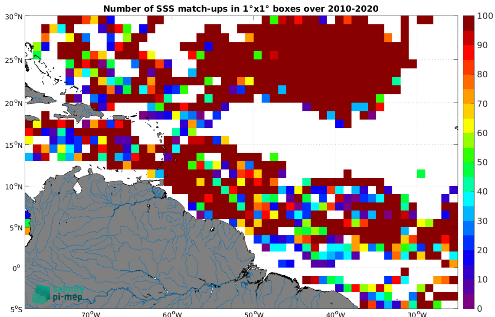
Figure 4: Number of SSS match-ups between Surface drifters SSS and the SMOS SSS L2Q v331 - No FLAG (CMEMS-CATDS-CPDC) SSS product for the Amazon and Orinoco river plumes Pi-MEP region over 1^\circ \times 1^\circ boxes and for the full satellite product period.
