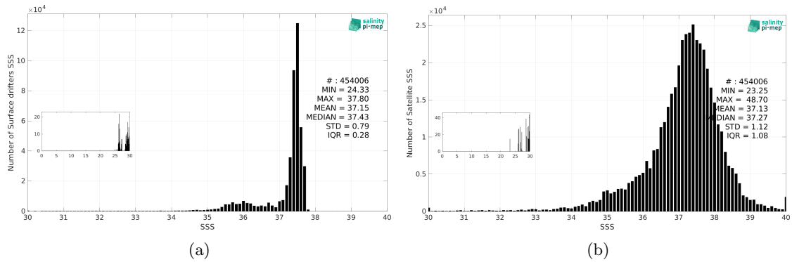
Figure 3: Histograms of SSS from Surface drifters (a) and SMOS SSS L2Q v331 - No FLAG (CMEMS-CATDS-CPDC) (b) considering all match-up pairs per bins of 0.1 over the Amazon and Orinoco river plumes Pi-MEP region and for the full satellite product period.
