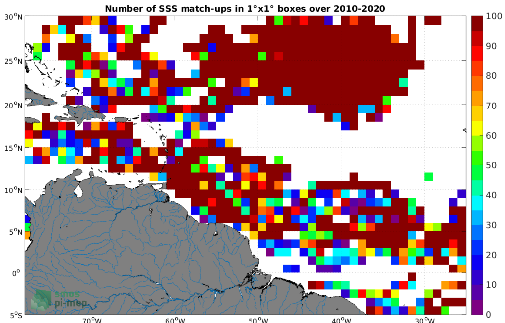
Figure 3: Number of SSS match-ups between Surface drifters SSS and the SMOS SSS L2Q v331 - No FLAG (CMEMS-CATDS-CPDC) SSS product for the Amazon and Orinoco river plumes Pi-MEP region over 1^\circ \times 1^\circ boxes and for the full satellite product period.
