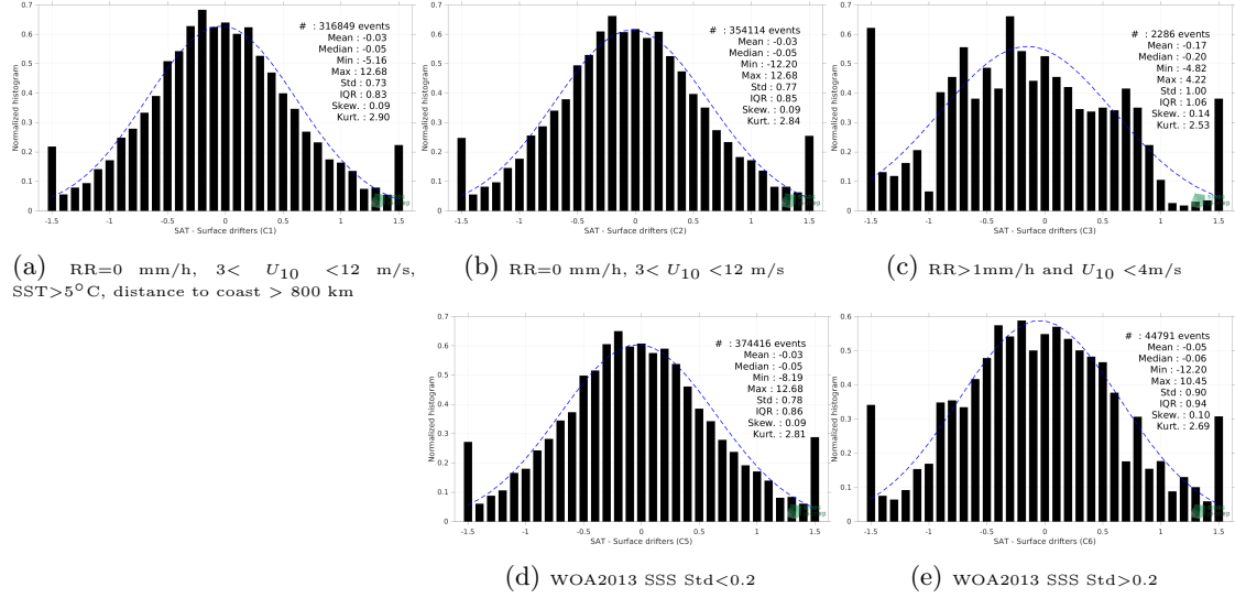
Figure 12: Normalized histogram of \Delta SSS (SMOS SSS L2Q v331 - No FLAG (CMEMS-CATDS-CPDC) - Surface drifters) for 5 different subdatasets corresponding to: RR=0 mm/h, 3 < U_{10} < 12 m/s, SST > 5°C, distance to coast > 800 km (a), RR=0 mm/h, 3 < U_{10} < 12 m/s (b), RR > 1mm/h and U_{10} < 4 m/s (c), WOA2013 SSS Std < 0.2 (d), WOA2013 SSS Std > 0.2 (e).
