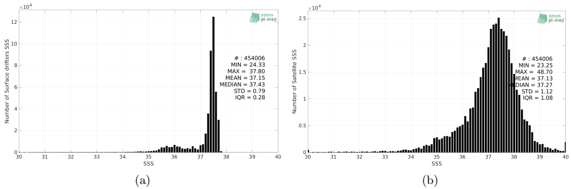
Figure 2: Histograms of SSS from Surface drifters (a) and SMOS SSS L2Q v331 - No FLAG (CMEMS-CATDS-CPDC) (b) considering all match-up pairs per bins of 0.1 over the Amazon and Orinoco river plumes Pi-MEP region and for the full satellite product period.
