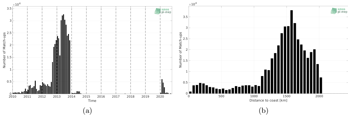
Figure 1: Number of match-ups between Surface drifters and SMOS SSS L2Q v331 - No FLAG (CMEMS-CATDS-CPDC) SSS as a function of time (a) and as function of the distance to coast (b) over the Amazon and Orinoco river plumes Pi-MEP region and for the full satellite product period.
