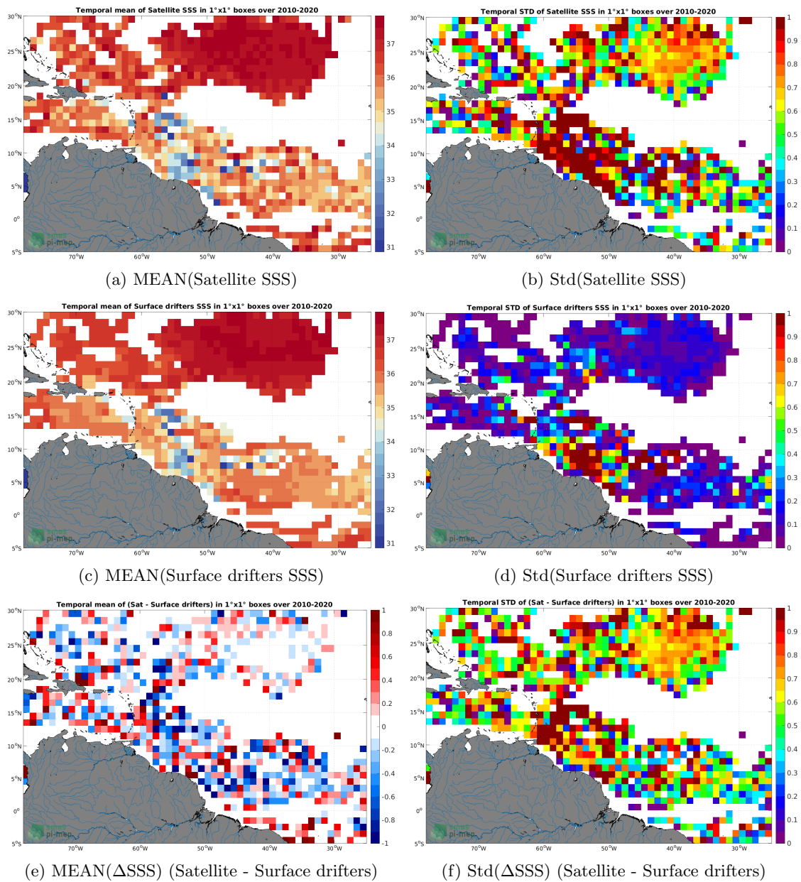
Figure 5: Temporal mean (left) and Std (right) of SSS from SMOS SSS L2Q v331 - No FLAG (CMEMS-CATDS-CPDC) (top), Surface drifters (middle), and of \Delta SSS (Satellite - Surface drifters). Only match-up pairs are used to generate these maps.
