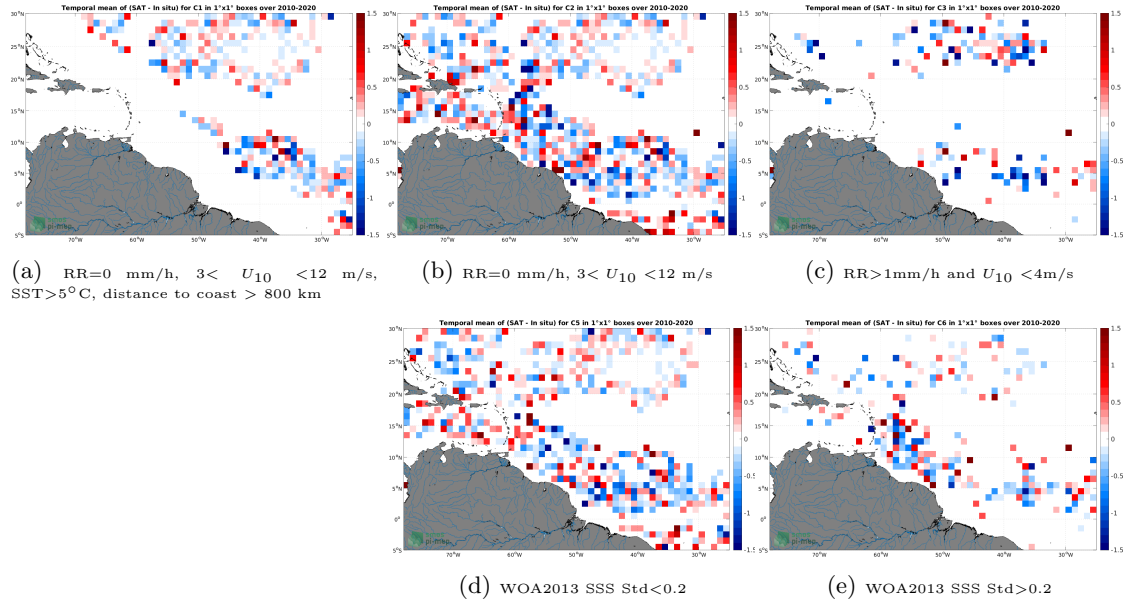
Figure 11: Temporal mean gridded over spatial boxes of size 1^{\circ}\times 1^{\circ} of \Delta\text{SSS} (SMOS SSS L2Q v331 - No FLAG (CMEMS-CATDS-CPDC) - Surface drifters) for 5 different subdatasets corresponding to:RR=0 mm/h, 3 < U_{10} < 12 m/s, SST >5^{\circ}\text{C} , distance to coast > 800 km (a), RR=0 mm/h, 3 < U_{10} < 12 m/s (b), RR >1 mm/h and U_{10} < 4 m/s (c), WOA2013 SSS Std <0.2 (d), WOA2013 SSS Std >0.2 (e).
