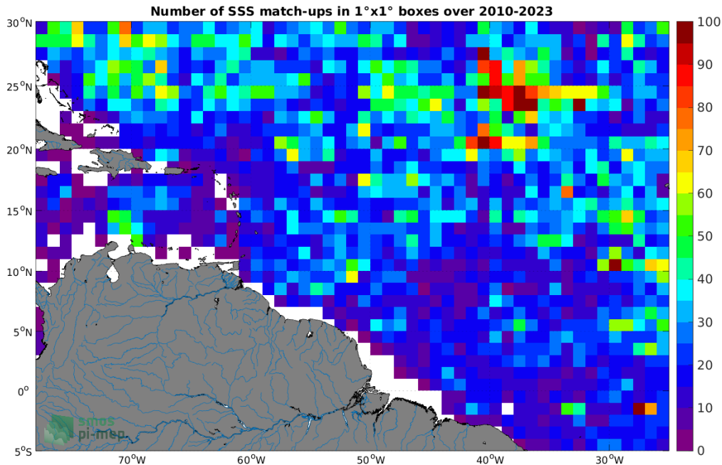
Figure 4: Number of SSS match-ups between Argo SSS and the SMOS SSS L2Q v331 - No FLAG (CMEMS-CATDS-CPDC) SSS product for the Amazon and Orinoco river plumes Pi-MEP region over 1^\circ \times 1^\circ boxes and for the full satellite product period.
