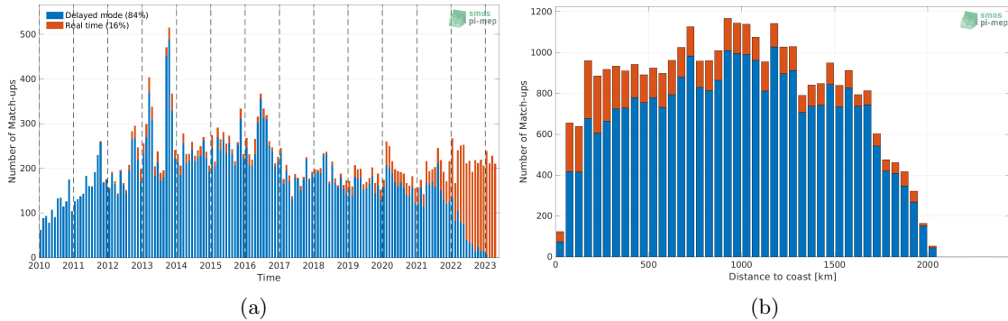
Figure 1: Number of match-ups between Argo and SMOS SSS L2Q v331 - No FLAG (CMEMS-CATDS-CPDC) SSS as a function of time (a) and as function of the distance to coast (b) over the Amazon and Orinoco river plumes Pi-MEP region and for the full satellite product period.
