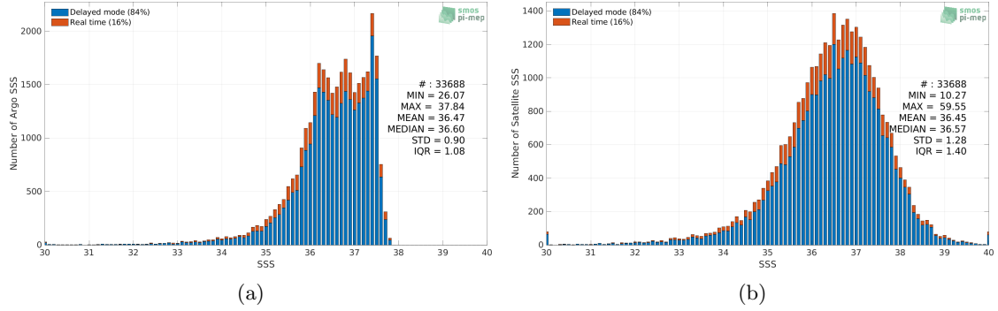
Figure 2: Histograms of SSS from Argo (a) and SMOS SSS L2Q v331 - No FLAG (CMEMS-CATDS-CPDC) (b) considering all match-up pairs per bins of 0.1 over the Amazon and Orinoco river plumes Pi-MEP region and for the full satellite product period.
