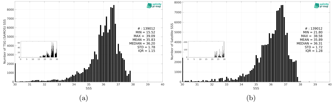
Figure 3: Histograms of SSS from TSG (SAMOS) (a) and SMOS SSS L3 v9 - 9 Days (CATDS-CEC-LOCEAN) (b) considering all match-up pairs per bins of 0.1 over the Amazon and Orinoco river plumes Pi-MEP region and for the full satellite product period.
