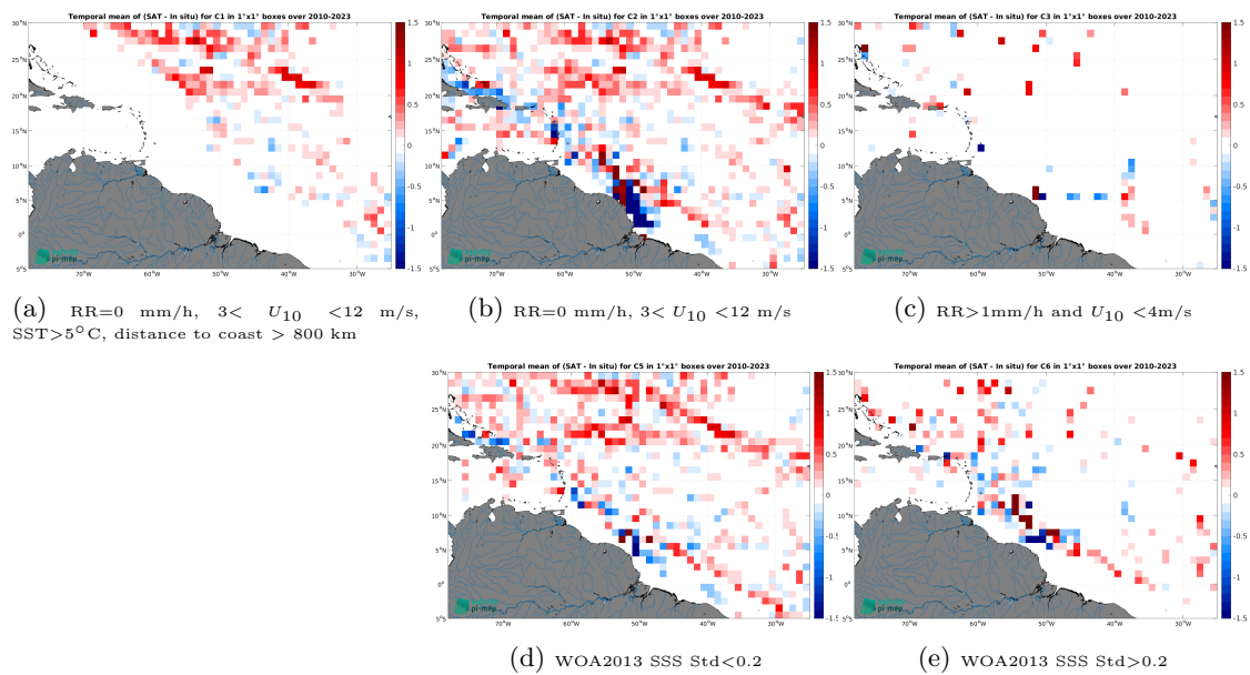
Figure 14: Temporal mean gridded over spatial boxes of size 1^\circ \times 1^\circ of \Delta\text{SSS} (SMOS SSS L3 v9 - 9 Days (CATDS-CEC-LOCEAN) - TSG (SAMOS)) for 5 different subdatasets corresponding to:RR=0 mm/h, 3 < U_{10} < 12 m/s, SST >5^\circ\text{C} , distance to coast > 800 km (a), RR=0 mm/h, 3 < U_{10} < 12 m/s (b), RR >1 mm/h and U_{10} < 4 m/s (c), WOA2013 SSS Std <0.2 (d), WOA2013 SSS Std >0.2 (e).
