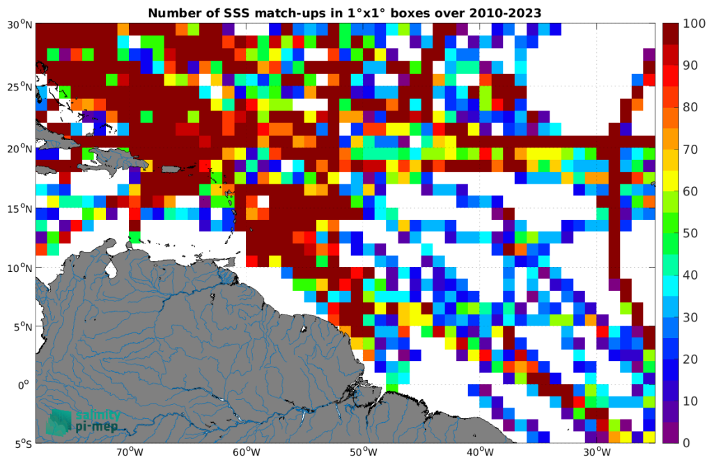
Figure 5: Number of SSS match-ups between TSG (SAMOS) SSS and the SMOS SSS L3 v9 - 9 Days (CATDS-CEC-LOCEAN) SSS product for the Amazon and Orinoco river plumes Pi-MEP region over 1^\circ \times 1^\circ boxes and for the full satellite product period.
