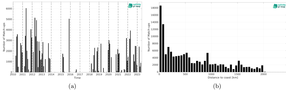
Figure 2: Number of match-ups between TSG (SAMOS) and SMOS SSS L3 v9 - 9 Days (CATDS-CEC-LOCEAN) SSS as a function of time (a) and as function of the distance to coast (b) over the Amazon and Orinoco river plumes Pi-MEP region and for the full satellite product period.
