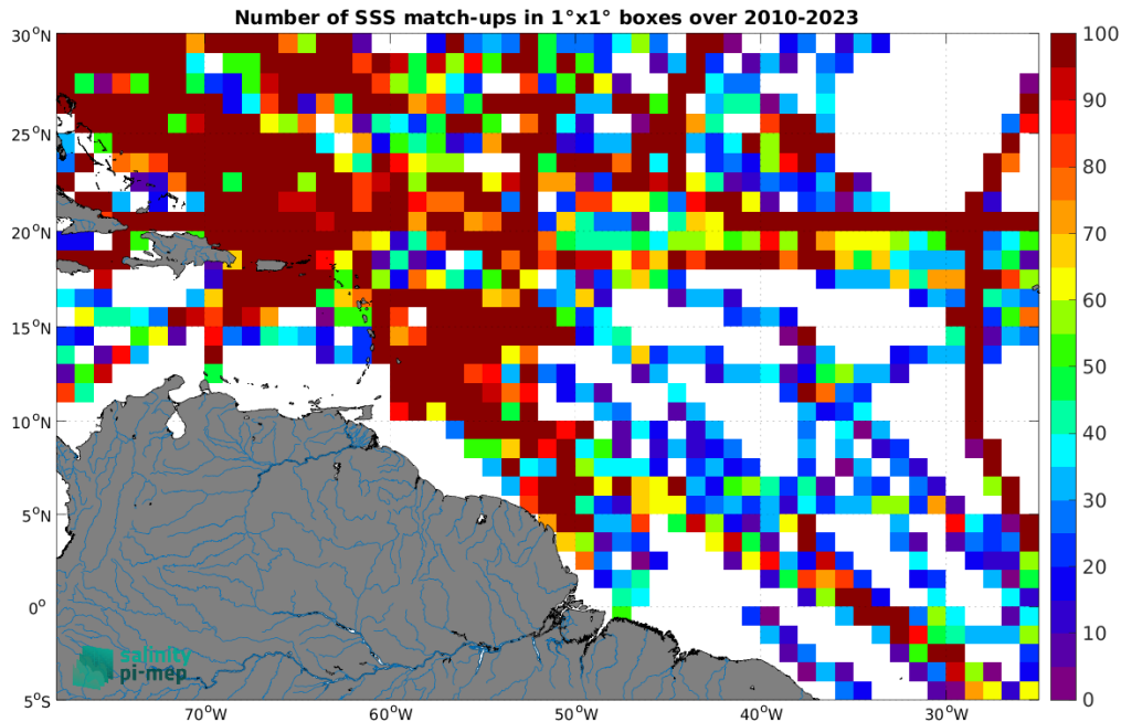
Figure 4: Number of SSS match-ups between TSG (SAMOS) SSS and the SMOS SSS L3 v9 - 9 Days (CATDS-CEC-LOCEAN) SSS product for the Amazon and Orinoco river plumes Pi-MEP region over 1^\circ \times 1^\circ boxes and for the full satellite product period.
