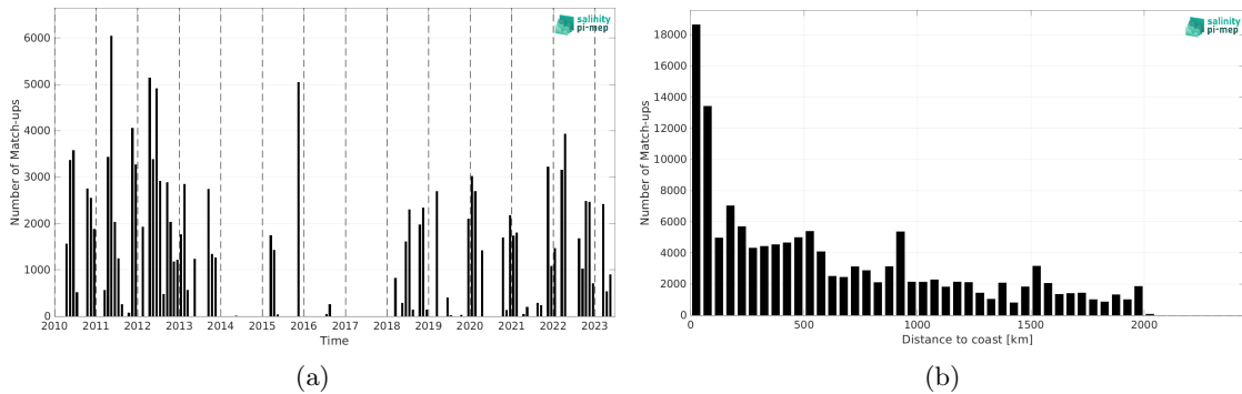
Figure 1: Number of match-ups between TSG (SAMOS) and SMOS SSS L3 v9 - 9 Days (CATDS-CEC-LOCEAN) SSS as a function of time (a) and as function of the distance to coast (b) over the Amazon and Orinoco river plumes Pi-MEP region and for the full satellite product period.
