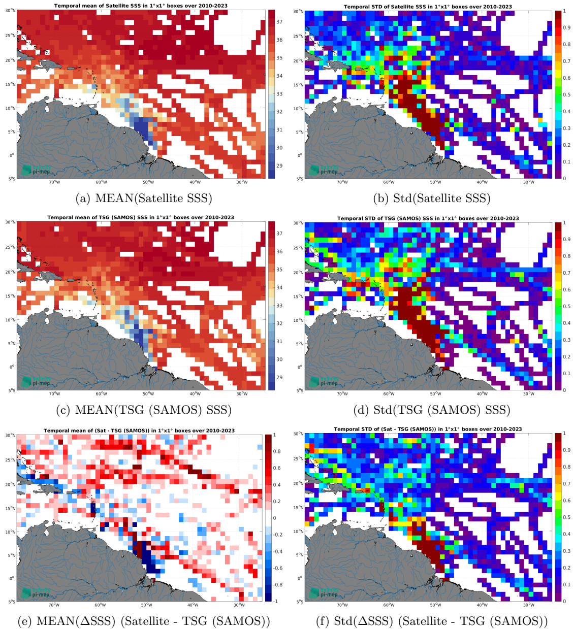
Figure 6: Temporal mean (left) and Std (right) of SSS from SMOS SSS L3 v9 - 9 Days (CATDS-CEC-LOCEAN) (top), TSG (SAMOS) (middle), and of \Delta SSS (Satellite - TSG (SAMOS)). Only match-up pairs are used to generate these maps.
