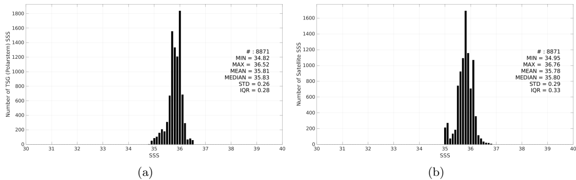
Figure 3: Histograms of SSS from TSG (Polarstern) (a) and SMOS SSS L3 v9 - 9 Days (CATDS-CEC-LOCEAN) (b) considering all match-up pairs per bins of 0.1 over the Amazon and Orinoco river plumes Pi-MEP region and for the full satellite product period.
