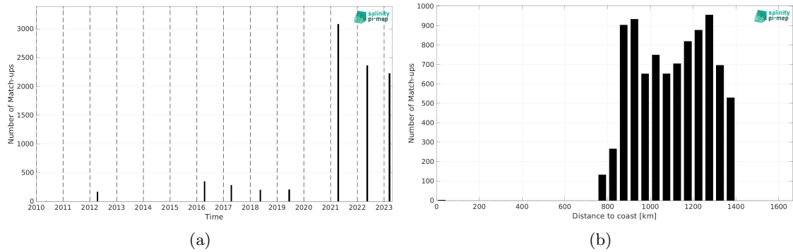
Figure 2: Number of match-ups between TSG (Polarstern) and SMOS SSS L3 v9 - 9 Days (CATDS-CEC-LOCEAN) SSS as a function of time (a) and as function of the distance to coast (b) over the Amazon and Orinoco river plumes Pi-MEP region and for the full satellite product period.
