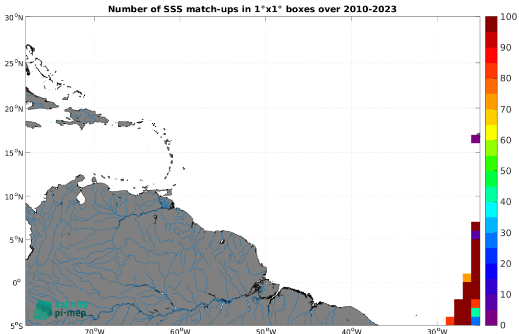
Figure 5: Number of SSS match-ups between TSG (Polarstern) SSS and the SMOS SSS L3 v9 - 9 Days (CATDS-CEC-LOCEAN) SSS product for the Amazon and Orinoco river plumes Pi-MEP region over 1^\circ \times 1^\circ boxes and for the full satellite product period.
