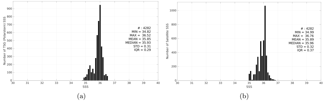
Figure 2: Histograms of SSS from TSG (Polarstern) (a) and SMOS SSS L3 v9 - 9 Days (CATDS-CEC-LOCEAN) (b) considering all match-up pairs per bins of 0.1 over the Amazon and Orinoco river plumes Pi-MEP region and for the full satellite product period.
