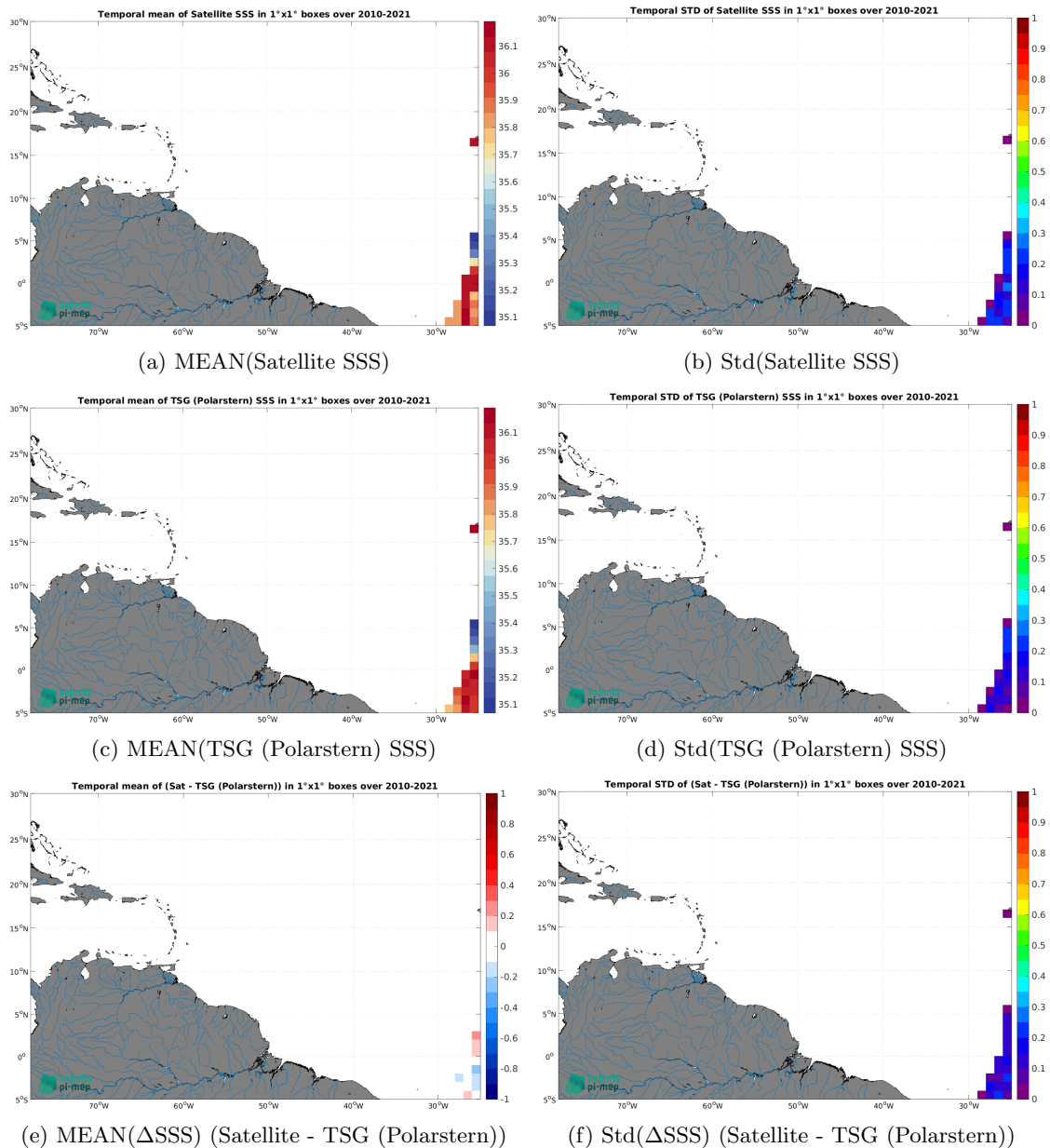
Figure 6: Temporal mean (left) and Std (right) of SSS from SMOS SSS L3 v9 - 9 Days (CATDS-CEC-LOCEAN) (top), TSG (Polarstern) (middle), and of \Delta SSS (Satellite - TSG (Polarstern)). Only match-up pairs are used to generate these maps.
