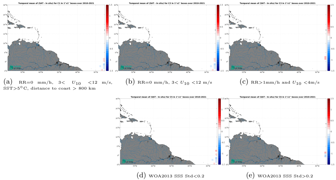
Figure 12: Temporal mean gridded over spatial boxes of size 1^{\circ}\times 1^{\circ} of \Delta\text{SSS} (SMOS SSS L3 v9 - 9 Days (CATDS-CEC-LOCEAN) - TSG (Polarstern)) for 5 different subdatasets corresponding to:RR=0 mm/h, 3 < U_{10} < 12 m/s, SST >5^{\circ}\text{C} , distance to coast > 800 km (a), RR=0 mm/h, 3 < U_{10} < 12 m/s (b), RR >1 mm/h and U_{10} < 4 m/s (c), WOA2013 SSS Std <0.2 (d), WOA2013 SSS Std >0.2 (e).
