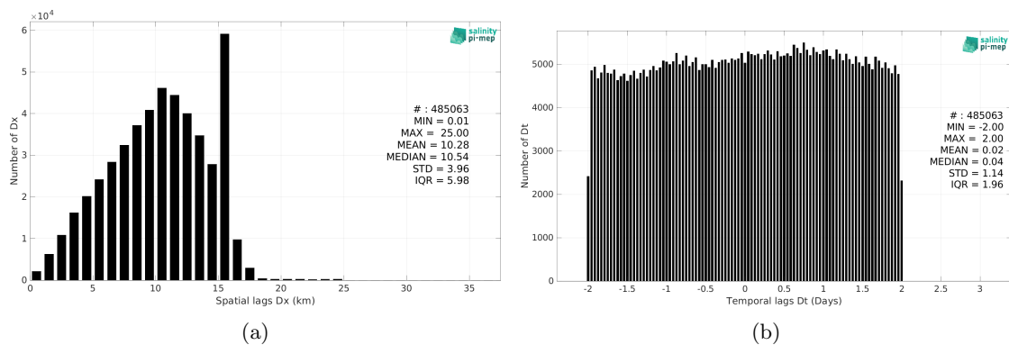
Figure 5: Histograms of the spatial (a) and temporal (b) lags between the location/time of the TSG (LEGOS-DM) measurement and the date of the corresponding SMOS SSS L3 v9 - 9 Days (CATDS-CEC-LOCEAN) SSS pixel.
