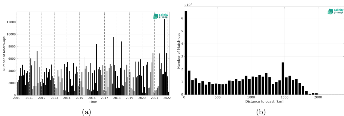
Figure 1: Number of match-ups between TSG (LEGOS-DM) and SMOS SSS L3 v9 - 9 Days (CATDS-CEC-LOCEAN) SSS as a function of time (a) and as function of the distance to coast (b) over the Amazon and Orinoco river plumes Pi-MEP region and for the full satellite product period.
