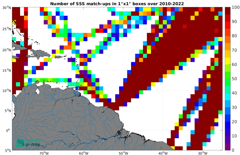
Figure 4: Number of SSS match-ups between TSG (LEGOS-DM) SSS and the SMOS SSS L3 v9 - 9 Days (CATDS-CEC-LOCEAN) SSS product for the Amazon and Orinoco river plumes Pi-MEP region over 1^\circ \times 1^\circ boxes and for the full satellite product period.
