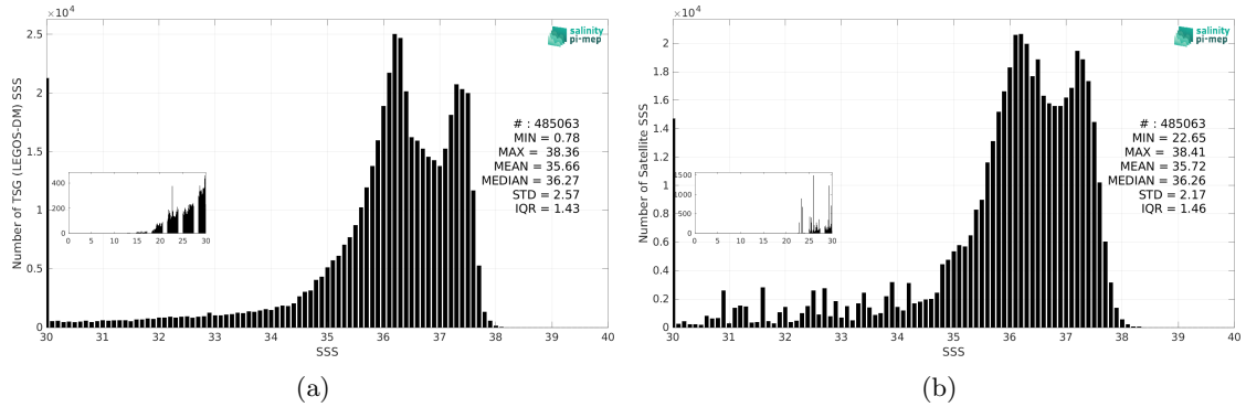
Figure 2: Histograms of SSS from TSG (LEGOS-DM) (a) and SMOS SSS L3 v9 - 9 Days (CATDS-CEC-LOCEAN) (b) considering all match-up pairs per bins of 0.1 over the Amazon and Orinoco river plumes Pi-MEP region and for the full satellite product period.
