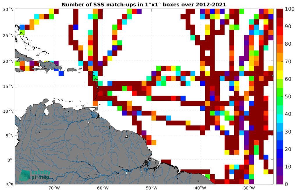
Figure 5: Number of SSS match-ups between TSG (GOSUD-Sailing-ship) SSS and the SMOS SSS L3 v9 - 9 Days (CATDS-CEC-LOCEAN) SSS product for the Amazon and Orinoco river plumes Pi-MEP region over 1^\circ \times 1^\circ boxes and for the full satellite product period.
