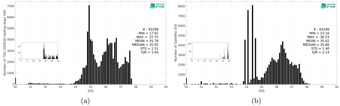
Figure 3: Histograms of SSS from TSG (GOSUD-Sailing-ship) (a) and SMOS SSS L3 v9 - 9 Days (CATDS-CEC-LOCEAN) (b) considering all match-up pairs per bins of 0.1 over the Amazon and Orinoco river plumes Pi-MEP region and for the full satellite product period.
