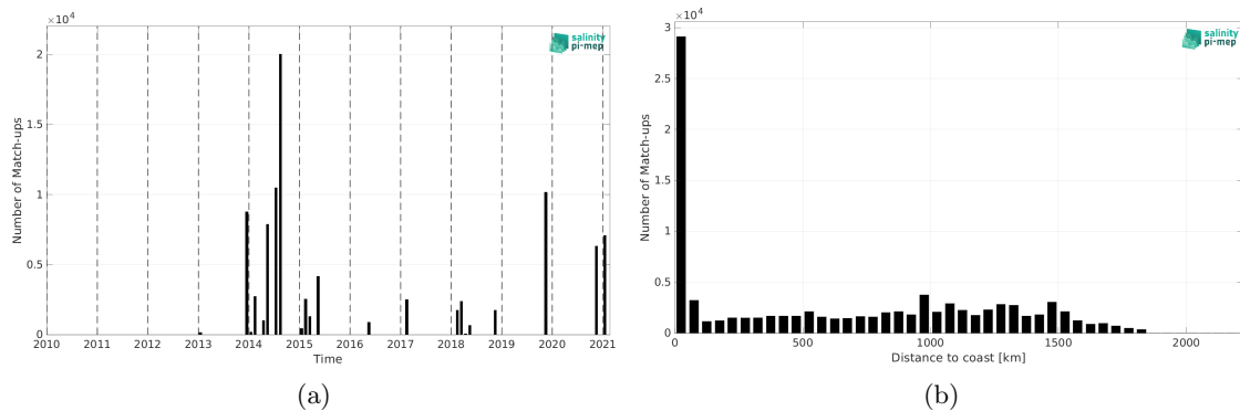
Figure 1: Number of match-ups between TSG (GOSUD-Sailing-ship) and SMOS SSS L3 v9 - 9 Days (CATDS-CEC-LOCEAN) SSS as a function of time (a) and as function of the distance to coast (b) over the Amazon and Orinoco river plumes Pi-MEP region and for the full satellite product period.
