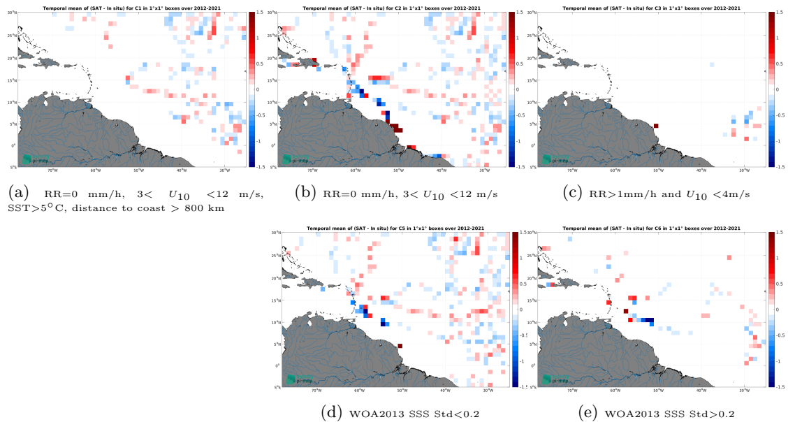
Figure 12: Temporal mean gridded over spatial boxes of size 1^{\circ}\times 1^{\circ} of \Delta SSS (SMOS SSS L3 v9 - 9 Days (CATDS-CEC-LOCEAN) - TSG (GOSUD-Sailing-ship)) for 5 different subdatasets corresponding to:RR=0 mm/h, 3 < U_{10} < 12 m/s, SST >5^{\circ}\text{C} , distance to coast > 800 km (a), RR=0 mm/h, 3 < U_{10} < 12 m/s (b), RR >1 mm/h and U_{10} < 4 m/s (c), WOA2013 SSS Std <0.2 (d), WOA2013 SSS Std >0.2 (e).
