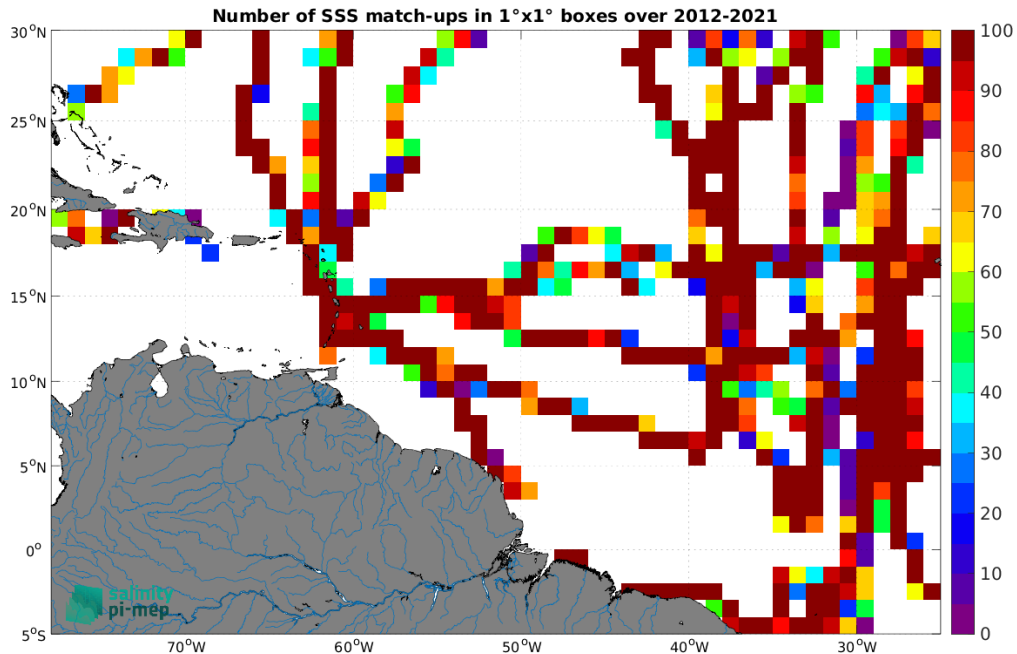
Figure 4: Number of SSS match-ups between TSG (GOSUD-Sailing-ship) SSS and the SMOS SSS L3 v9 - 9 Days (CATDS-CEC-LOCEAN) SSS product for the Amazon and Orinoco river plumes Pi-MEP region over 1^\circ \times 1^\circ boxes and for the full satellite product period.
