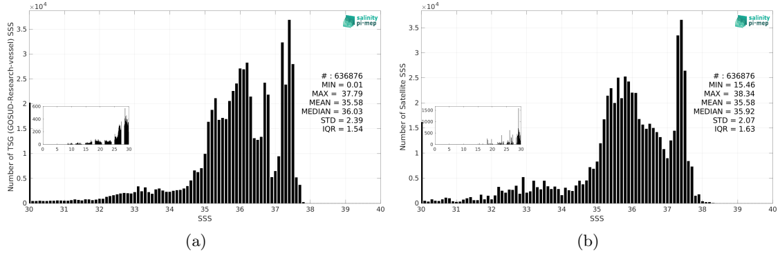
Figure 2: Histograms of SSS from TSG (GOSUD-Research-vessel) (a) and SMOS SSS L3 v9 - 9 Days (CATDS-CEC-LOCEAN) (b) considering all match-up pairs per bins of 0.1 over the Amazon and Orinoco river plumes Pi-MEP region and for the full satellite product period.
