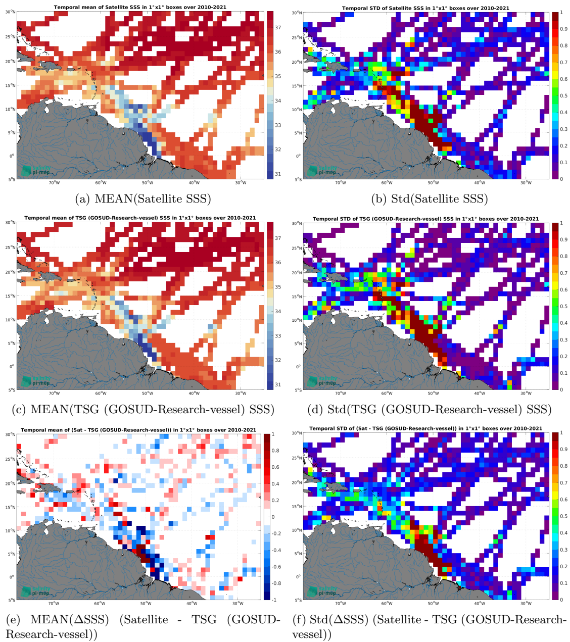
Figure 6: Temporal mean (left) and Std (right) of SSS from SMOS SSS L3 v9 - 9 Days (CATDS-CEC-LOCEAN) (top), TSG (GOSUD-Research-vessel) (middle), and of \Delta SSS (Satellite - TSG (GOSUD-Research-vessel)). Only match-up pairs are used to generate these maps.
