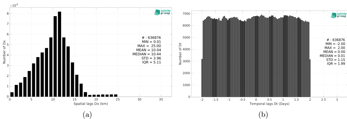
Figure 5: Histograms of the spatial (a) and temporal (b) lags between the location/time of the TSG (GOSUD-Research-vessel) measurement and the date of the corresponding SMOS SSS L3 v9 - 9 Days (CATDS-CEC-LOCEAN) SSS pixel.
