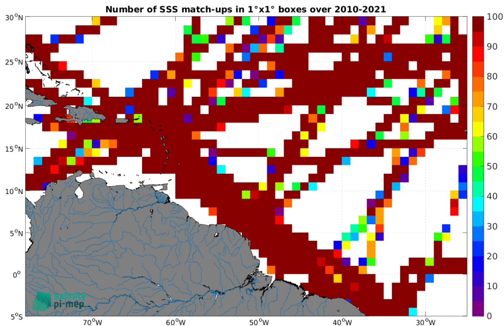
Figure 4: Number of SSS match-ups between TSG (GOSUD-Research-vessel) SSS and the SMOS SSS L3 v9 - 9 Days (CATDS-CEC-LOCEAN) SSS product for the Amazon and Orinoco river plumes Pi-MEP region over 1^\circ \times 1^\circ boxes and for the full satellite product period.
