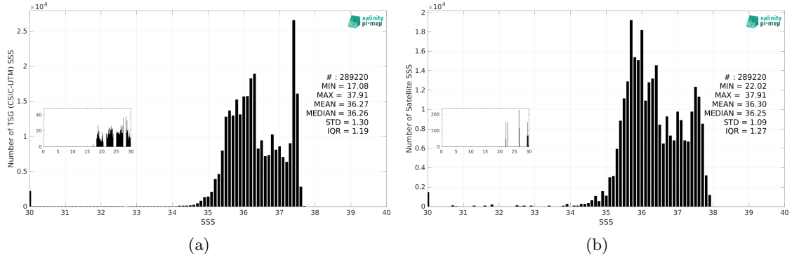
Figure 2: Histograms of SSS from TSG (CSIC-UTM) (a) and SMOS SSS L3 v9 - 9 Days (CATDS-CEC-LOCEAN) (b) considering all match-up pairs per bins of 0.1 over the Amazon and Orinoco river plumes Pi-MEP region and for the full satellite product period.
