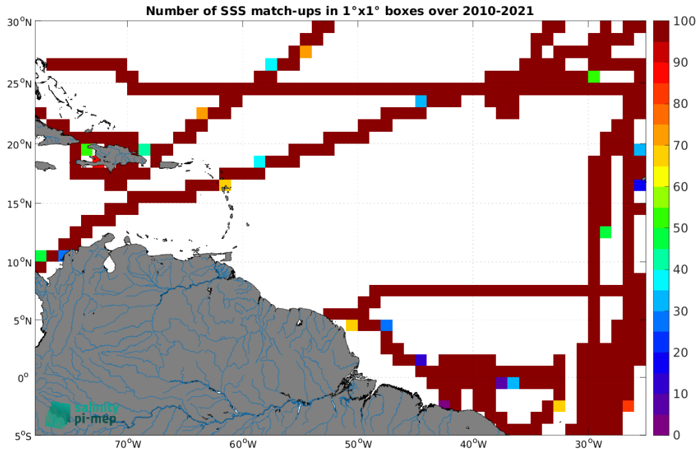
Figure 4: Number of SSS match-ups between TSG (CSIC-UTM) SSS and the SMOS SSS L3 v9 - 9 Days (CATDS-CEC-LOCEAN) SSS product for the Amazon and Orinoco river plumes Pi-MEP region over 1^\circ \times 1^\circ boxes and for the full satellite product period.
