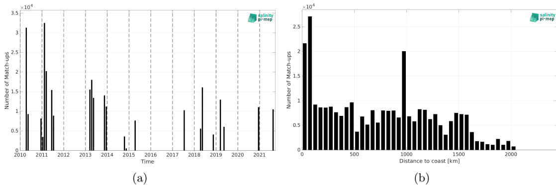
Figure 1: Number of match-ups between TSG (CSIC-UTM) and SMOS SSS L3 v9 - 9 Days (CATDS-CEC-LOCEAN) SSS as a function of time (a) and as function of the distance to coast (b) over the Amazon and Orinoco river plumes Pi-MEP region and for the full satellite product period.
