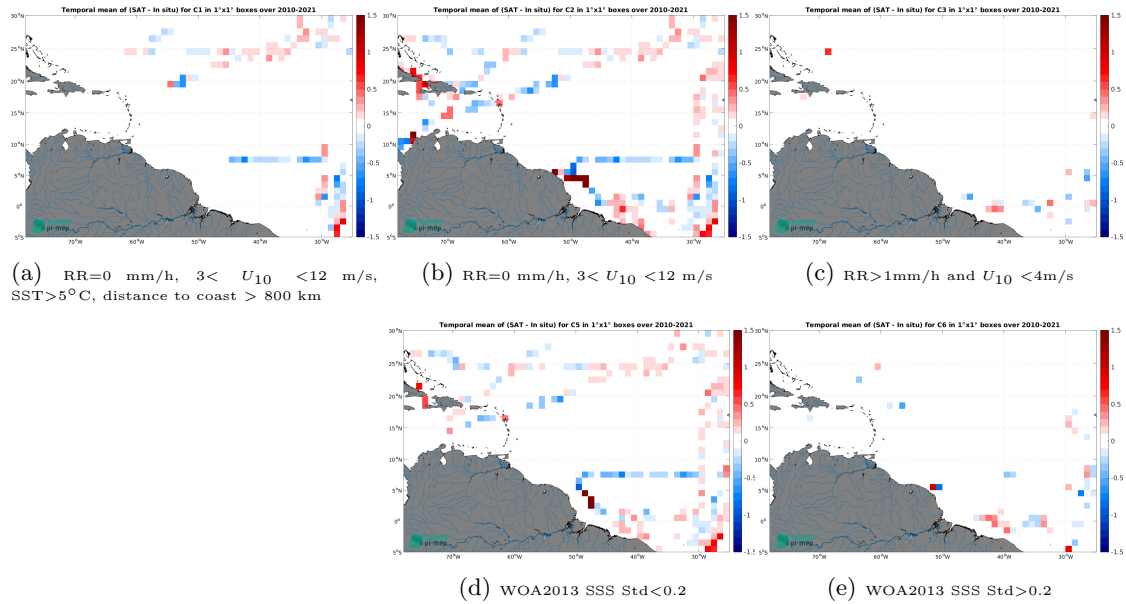
Figure 12: Temporal mean gridded over spatial boxes of size 1^\circ \times 1^\circ of \Delta SSS (SMOS SSS L3 v9 - 9 Days (CATDS-CEC-LOCEAN) - TSG (CSIC-UTM)) for 5 different subdatasets corresponding to:RR=0 mm/h, 3 < U_{10} < 12 m/s, SST >5^\circ\text{C} , distance to coast > 800 km (a), RR=0 mm/h, 3 < U_{10} < 12 m/s (b), RR >1 mm/h and U_{10} < 4 m/s (c), WOA2013 SSS Std <0.2 (d), WOA2013 SSS Std >0.2 (e).
