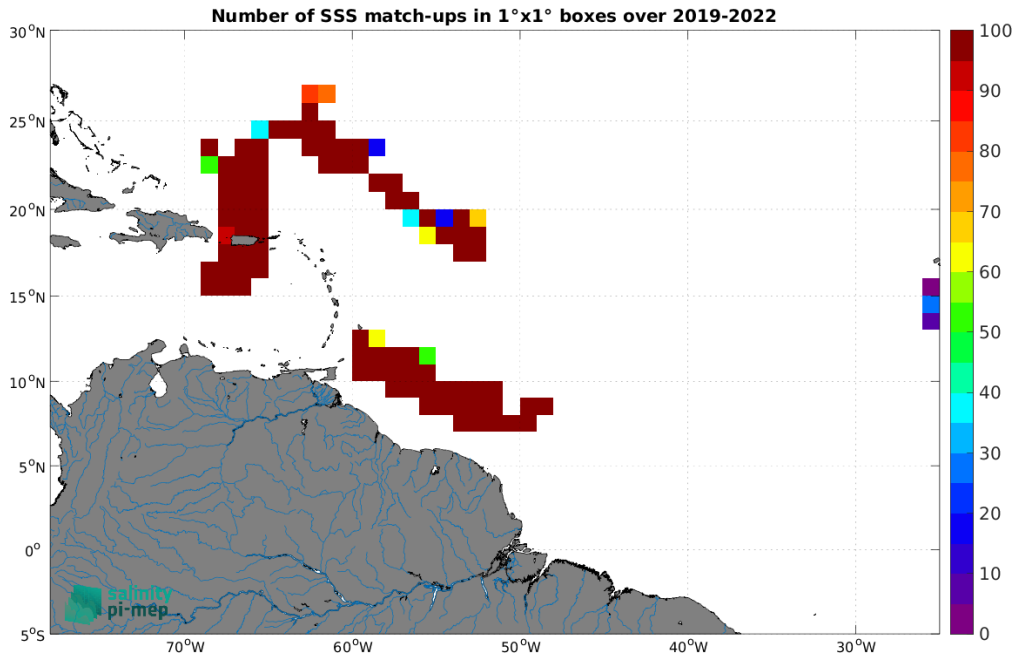
Figure 5: Number of SSS match-ups between Saildrone SSS and the SMOS SSS L3 v9 - 9 Days (CATDS-CEC-LOCEAN) SSS product for the Amazon and Orinoco river plumes Pi-MEP region over 1^\circ \times 1^\circ boxes and for the full satellite product period.
