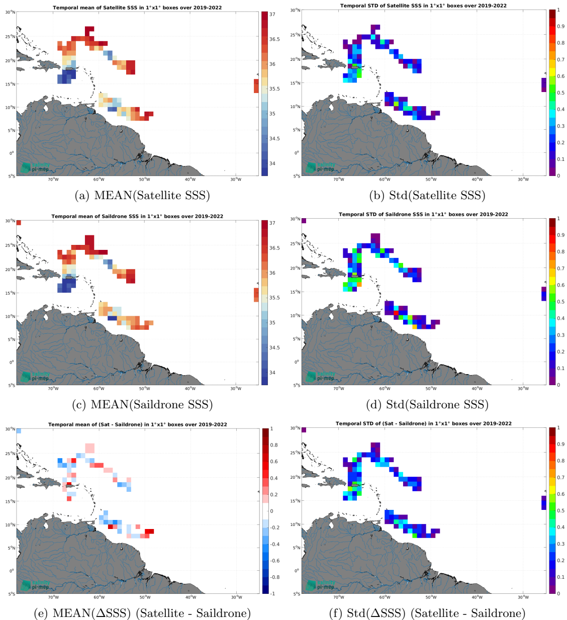
Figure 6: Temporal mean (left) and Std (right) of SSS from SMOS SSS L3 v9 - 9 Days (CATDS-CEC-LOCEAN) (top), Saildrone (middle), and of \Delta SSS (Satellite - Saildrone). Only match-up pairs are used to generate these maps.
