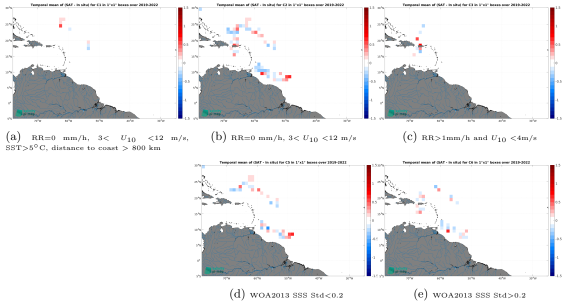
Figure 12: Temporal mean gridded over spatial boxes of size 1^\circ \times 1^\circ of \Delta SSS (SMOS SSS L3 v9 - 9 Days (CATDS-CEC-LOCEAN) - Saildrone) for 5 different subdatasets corresponding to:RR=0 mm/h, 3 < U_{10} < 12 m/s, SST >5^\circ\text{C} , distance to coast > 800 km (a), RR=0 mm/h, 3 < U_{10} < 12 m/s (b), RR >1 mm/h and U_{10} < 4 m/s (c), WOA2013 SSS Std <0.2 (d), WOA2013 SSS Std >0.2 (e).
