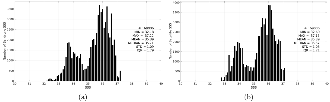
Figure 2: Histograms of SSS from Saildrone (a) and SMOS SSS L3 v9 - 9 Days (CATDS-CEC-LOCEAN) (b) considering all match-up pairs per bins of 0.1 over the Amazon and Orinoco river plumes Pi-MEP region and for the full satellite product period.
