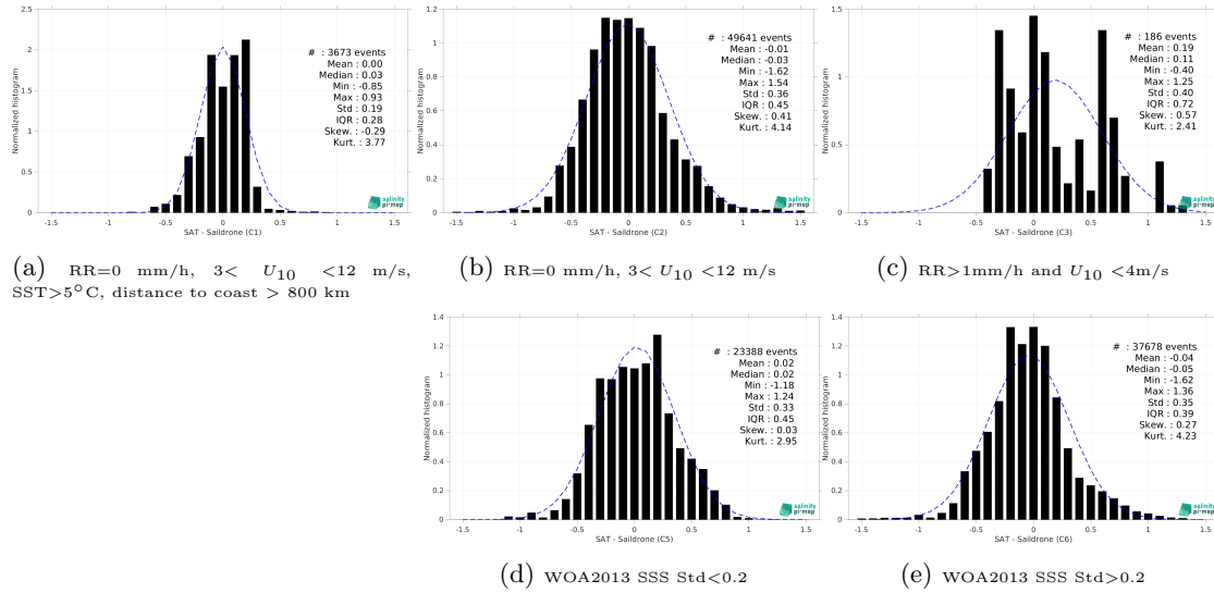
Figure 13: Normalized histogram of \Delta SSS (SMOS SSS L3 v9 - 9 Days (CATDS-CEC-LOCEAN) - Sairdron) for 5 different subdatasets corresponding to: RR=0 mm/h, 3 < U_{10} < 12 m/s, SST>5°C, distance to coast > 800 km (a), RR=0 mm/h, 3 < U_{10} < 12 m/s (b), RR>1mm/h and U_{10} < 4 m/s (c), WOA2013 SSS Std<0.2 (d), WOA2013 SSS Std>0.2 (e).
