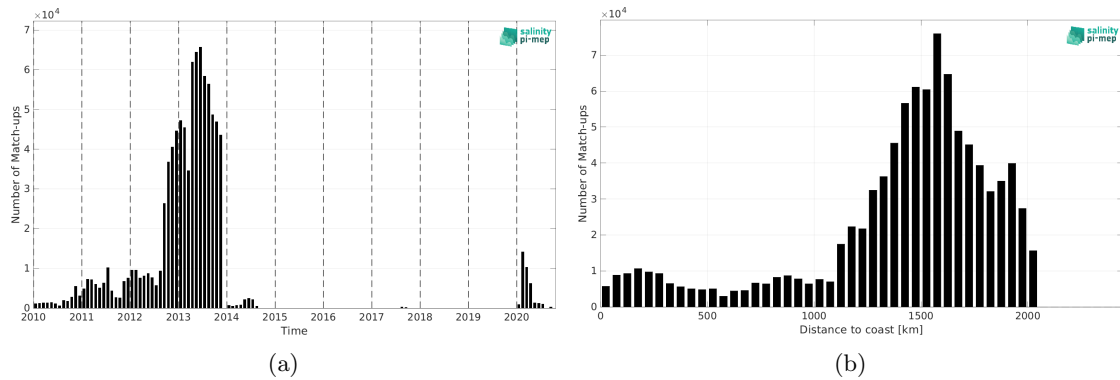
Figure 2: Number of match-ups between Surface drifters and SMOS SSS L3 v9 - 9 Days (CATDS-CEC-LOCEAN) SSS as a function of time (a) and as function of the distance to coast (b) over the Amazon and Orinoco river plumes Pi-MEP region and for the full satellite product period.
