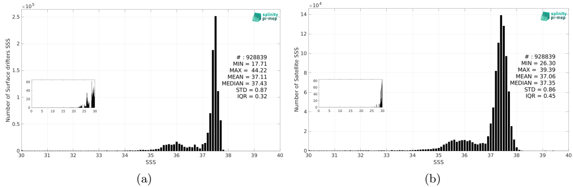
Figure 3: Histograms of SSS from Surface drifters (a) and SMOS SSS L3 v9 - 9 Days (CATDS-CEC-LOCEAN) (b) considering all match-up pairs per bins of 0.1 over the Amazon and Orinoco river plumes Pi-MEP region and for the full satellite product period.
