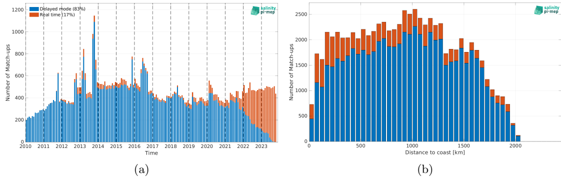
Figure 1: Number of match-ups between Argo and SMOS SSS L3 v9 - 9 Days (CATDS-CEC-LOCEAN) SSS as a function of time (a) and as function of the distance to coast (b) over the Amazon and Orinoco river plumes Pi-MEP region and for the full satellite product period.
