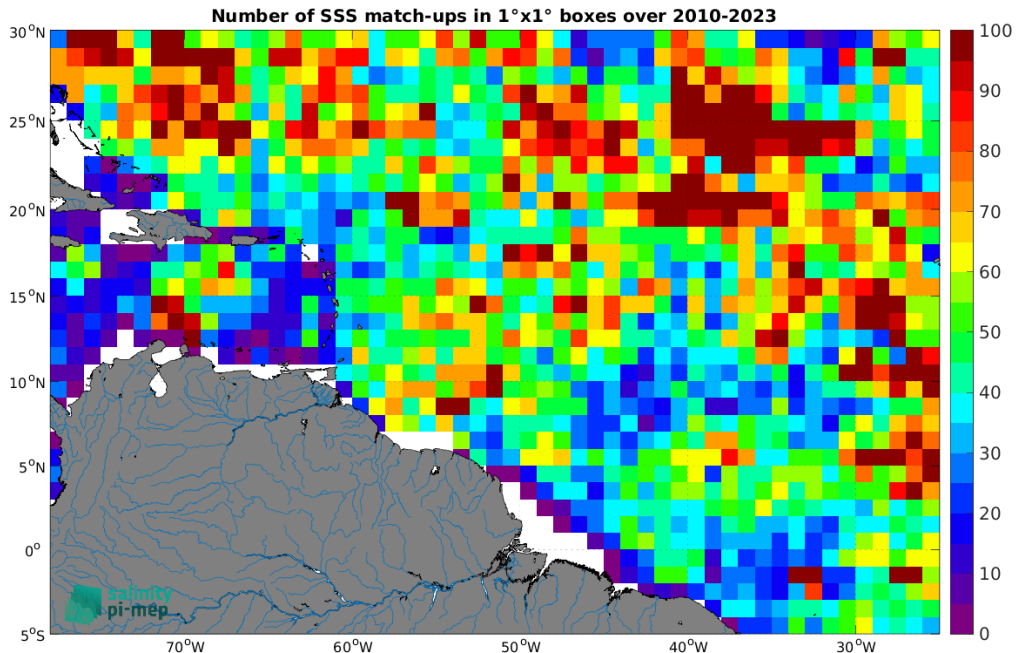
Figure 4: Number of SSS match-ups between Argo SSS and the SMOS SSS L3 v9 - 9 Days (CATDS-CEC-LOCEAN) SSS product for the Amazon and Orinoco river plumes Pi-MEP region over 1^\circ \times 1^\circ boxes and for the full satellite product period.
