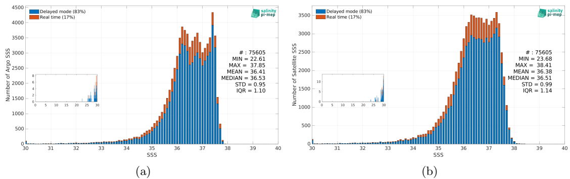
Figure 2: Histograms of SSS from Argo (a) and SMOS SSS L3 v9 - 9 Days (CATDS-CEC-LOCEAN) (b) considering all match-up pairs per bins of 0.1 over the Amazon and Orinoco river plumes Pi-MEP region and for the full satellite product period.
