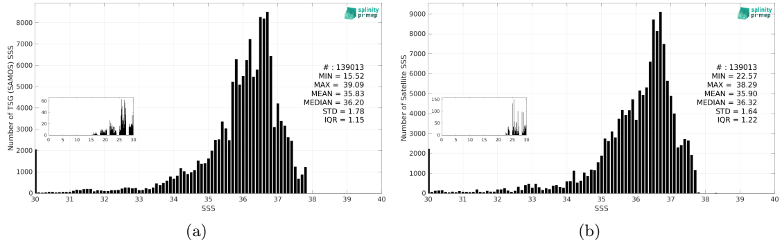
Figure 2: Histograms of SSS from TSG (SAMOS) (a) and SMOS SSS L3 v9 - 18 Days (CATDS-CEC-LOCEAN) (b) considering all match-up pairs per bins of 0.1 over the Amazon and Orinoco river plumes Pi-MEP region and for the full satellite product period.
