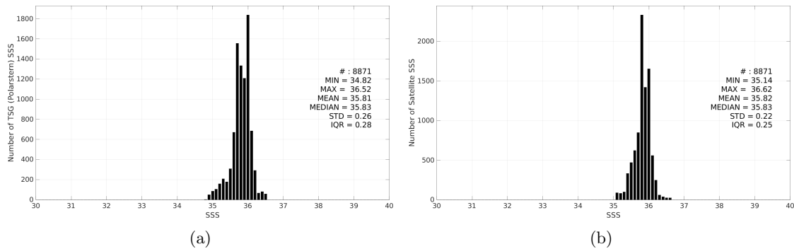
Figure 3: Histograms of SSS from TSG (Polarstern) (a) and SMOS SSS L3 v9 - 18 Days (CATDS-CEC-LOCEAN) (b) considering all match-up pairs per bins of 0.1 over the Amazon and Orinoco river plumes Pi-MEP region and for the full satellite product period.
