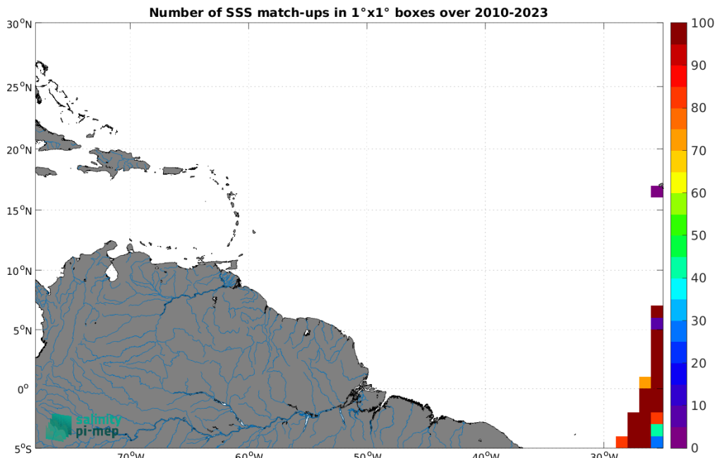
Figure 5: Number of SSS match-ups between TSG (Polarstern) SSS and the SMOS SSS L3 v9 - 18 Days (CATDS-CEC-LOCEAN) SSS product for the Amazon and Orinoco river plumes Pi-MEP region over 1^\circ \times 1^\circ boxes and for the full satellite product period.
