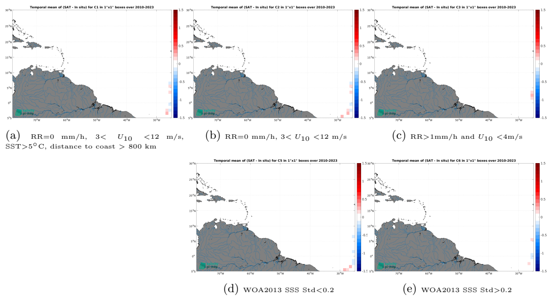
Figure 14: Temporal mean gridded over spatial boxes of size 1^\circ \times 1^\circ of \Delta SSS (SMOS SSS L3 v9 - 18 Days (CATDS-CEC-LOCEAN) - TSG (Polarstern)) for 5 different subdatasets corresponding to:RR=0 mm/h, 3 < U_{10} < 12 m/s, SST >5^\circ\text{C} , distance to coast > 800 km (a), RR=0 mm/h, 3 < U_{10} < 12 m/s (b), RR >1 mm/h and U_{10} < 4 m/s (c), WOA2013 SSS Std <0.2 (d), WOA2013 SSS Std >0.2 (e).
