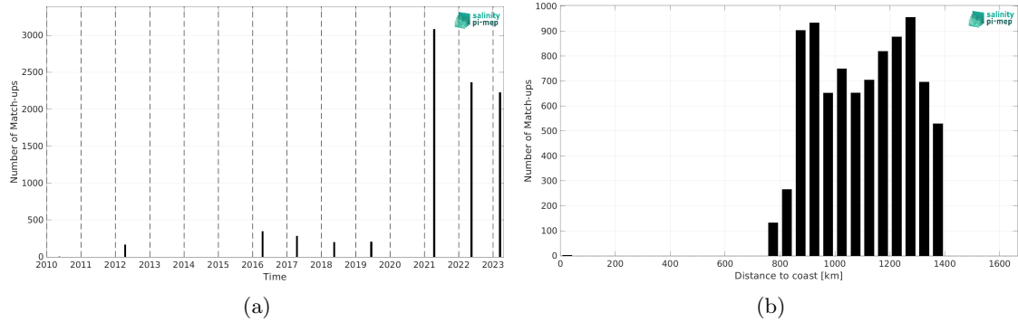
Figure 2: Number of match-ups between TSG (Polarstern) and SMOS SSS L3 v9 - 18 Days (CATDS-CEC-LOCEAN) SSS as a function of time (a) and as function of the distance to coast (b) over the Amazon and Orinoco river plumes Pi-MEP region and for the full satellite product period.
