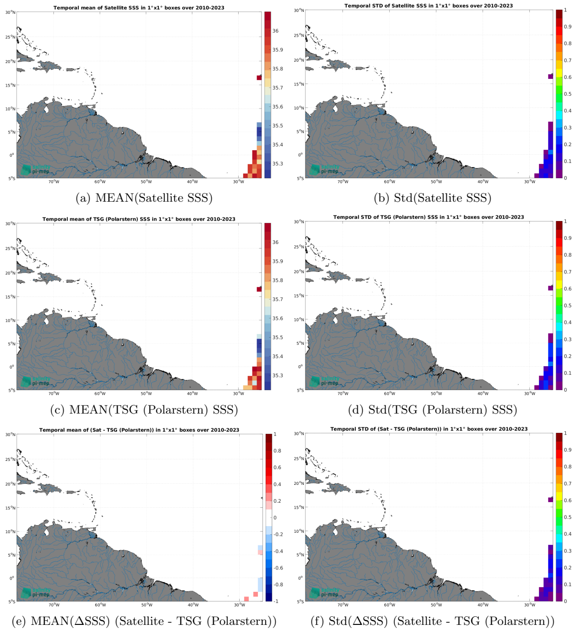
Figure 7: Temporal mean (left) and Std (right) of SSS from SMOS SSS L3 v9 - 18 Days (CATDS-CEC-LOCEAN) (top), TSG (Polarstern) (middle), and of \Delta SSS (Satellite - TSG (Polarstern)). Only match-up pairs are used to generate these maps.
