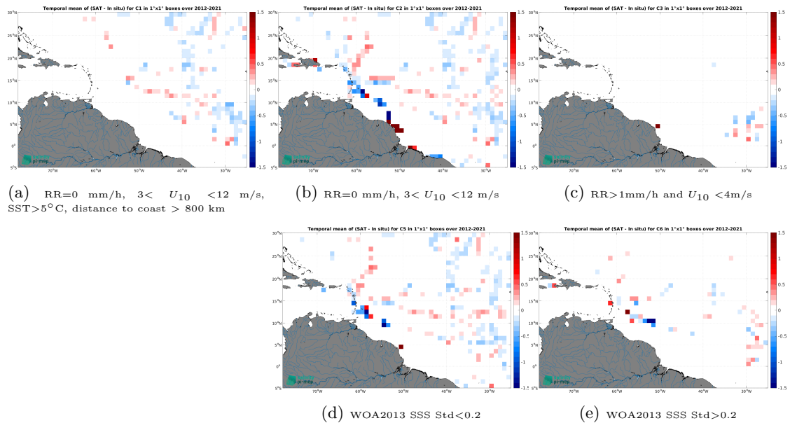
Figure 12: Temporal mean gridded over spatial boxes of size 1^{\circ}\times 1^{\circ} of \Delta SSS (SMOS SSS L3 v9 - 18 Days (CATDS-CEC-LOCEAN) - TSG (GOSUD-Sailing-ship)) for 5 different subdatasets corresponding to:RR=0 mm/h, 3 < U_{10} < 12 m/s, SST > 5^{\circ}\text{C} , distance to coast > 800 km (a), RR=0 mm/h, 3 < U_{10} < 12 m/s (b), RR > 1 mm/h and U_{10} < 4 m/s (c), WOA2013 SSS Std < 0.2 (d), WOA2013 SSS Std > 0.2 (e).
