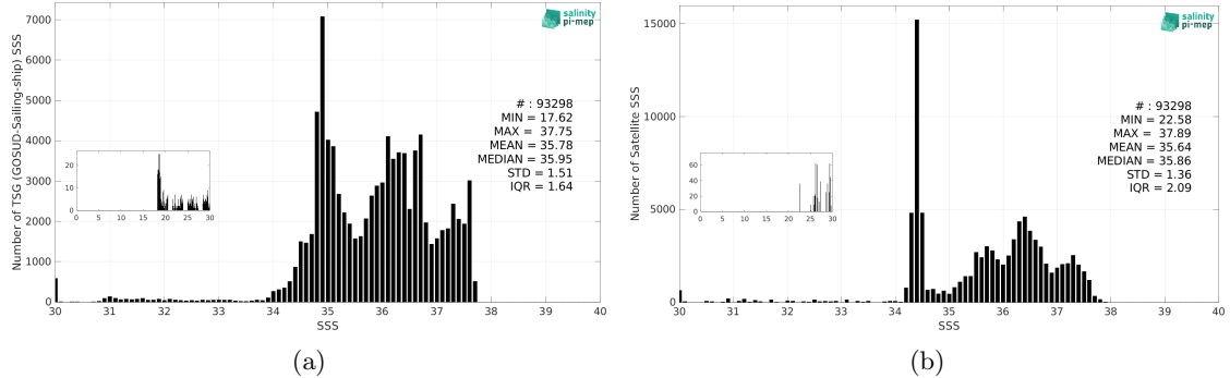
Figure 2: Histograms of SSS from TSG (GOSUD-Sailing-ship) (a) and SMOS SSS L3 v9 - 18 Days (CATDS-CEC-LOCEAN) (b) considering all match-up pairs per bins of 0.1 over the Amazon and Orinoco river plumes Pi-MEP region and for the full satellite product period.
