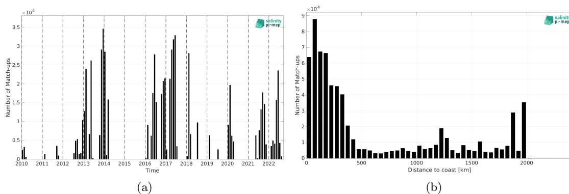
Figure 2: Number of match-ups between TSG (GOSUD-Research-vessel) and SMOS SSS L3 v9 - 18 Days (CATDS-CEC-LOCEAN) SSS as a function of time (a) and as function of the distance to coast (b) over the Amazon and Orinoco river plumes Pi-MEP region and for the full satellite product period.
