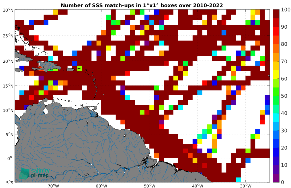
Figure 5: Number of SSS match-ups between TSG (GOSUD-Research-vessel) SSS and the SMOS SSS L3 v9 - 18 Days (CATDS-CEC-LOCEAN) SSS product for the Amazon and Orinoco river plumes Pi-MEP region over 1^\circ \times 1^\circ boxes and for the full satellite product period.
