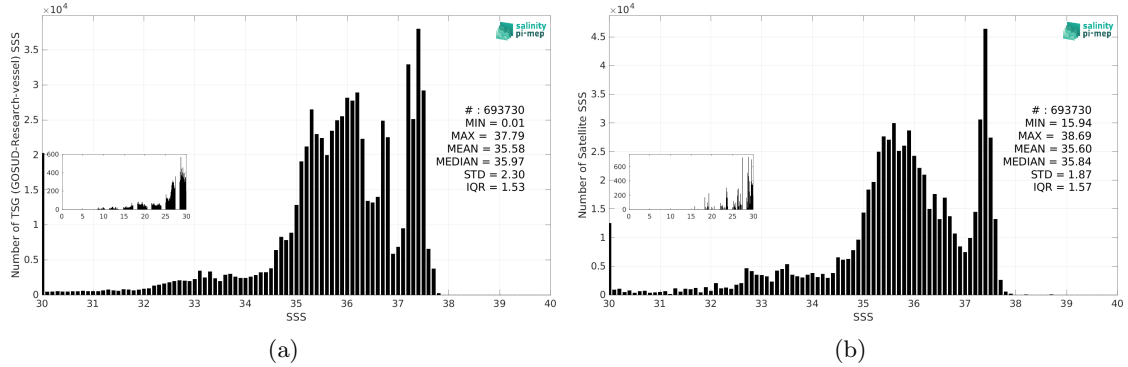
Figure 3: Histograms of SSS from TSG (GOSUD-Research-vessel) (a) and SMOS SSS L3 v9 - 18 Days (CATDS-CEC-LOCEAN) (b) considering all match-up pairs per bins of 0.1 over the Amazon and Orinoco river plumes Pi-MEP region and for the full satellite product period.
