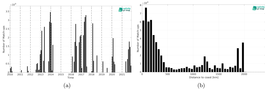
Figure 2: Number of match-ups between TSG (GOSUD-Research-vessel) and SMOS SSS L3 v9 - 18 Days (CATDS-CEC-LOCEAN) SSS as a function of time (a) and as function of the distance to coast (b) over the Amazon and Orinoco river plumes Pi-MEP region and for the full satellite product period.
