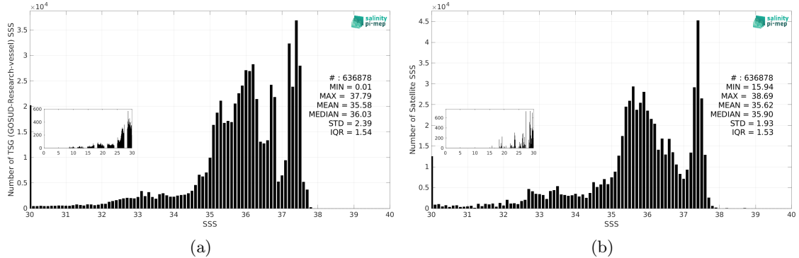
Figure 3: Histograms of SSS from TSG (GOSUD-Research-vessel) (a) and SMOS SSS L3 v9 - 18 Days (CATDS-CEC-LOCEAN) (b) considering all match-up pairs per bins of 0.1 over the Amazon and Orinoco river plumes Pi-MEP region and for the full satellite product period.
