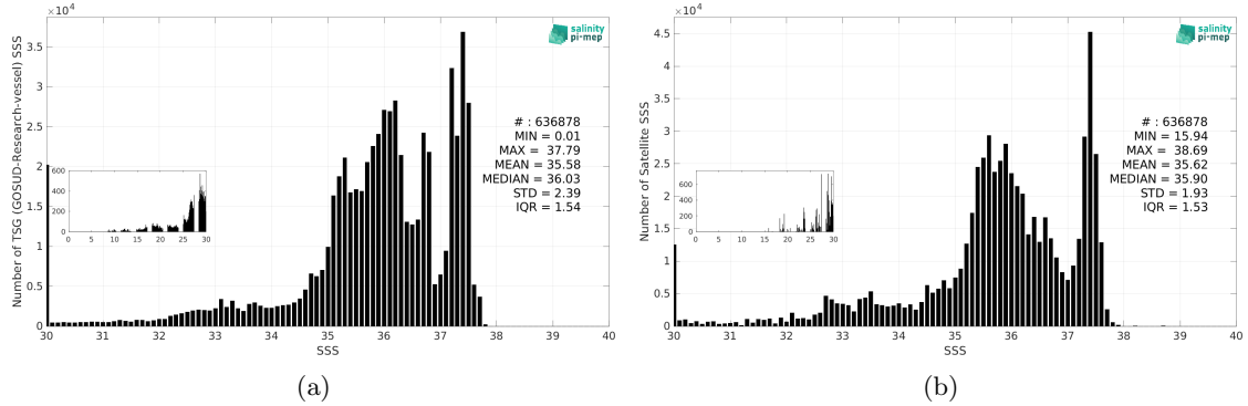
Figure 2: Histograms of SSS from TSG (GOSUD-Research-vessel) (a) and SMOS SSS L3 v9 - 18 Days (CATDS-CEC-LOCEAN) (b) considering all match-up pairs per bins of 0.1 over the Amazon and Orinoco river plumes Pi-MEP region and for the full satellite product period.
