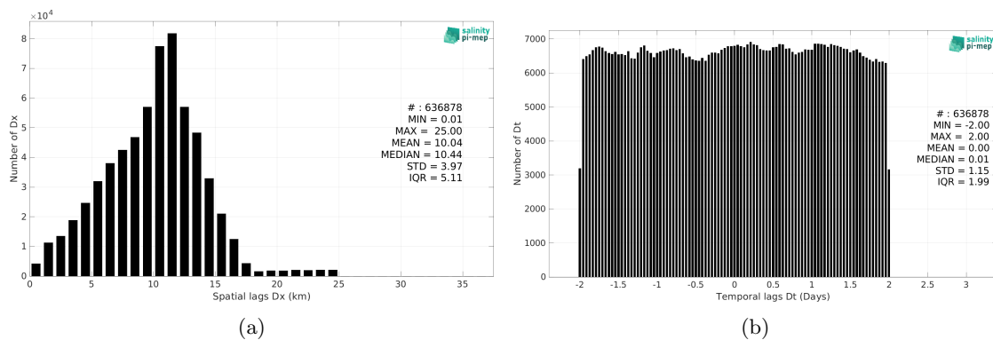
Figure 5: Histograms of the spatial (a) and temporal (b) lags between the location/time of the TSG (GOSUD-Research-vessel) measurement and the date of the corresponding SMOS SSS L3 v9 - 18 Days (CATDS-CEC-LOCEAN) SSS pixel.
