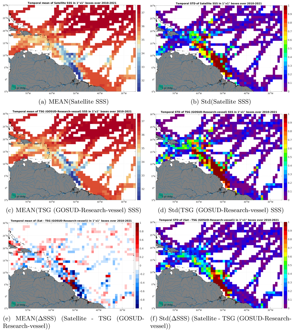
Figure 6: Temporal mean (left) and Std (right) of SSS from SMOS SSS L3 v9 - 18 Days (CATDS-CEC-LOCEAN) (top), TSG (GOSUD-Research-vessel) (middle), and of \Delta SSS (Satellite - TSG (GOSUD-Research-vessel)). Only match-up pairs are used to generate these maps.
