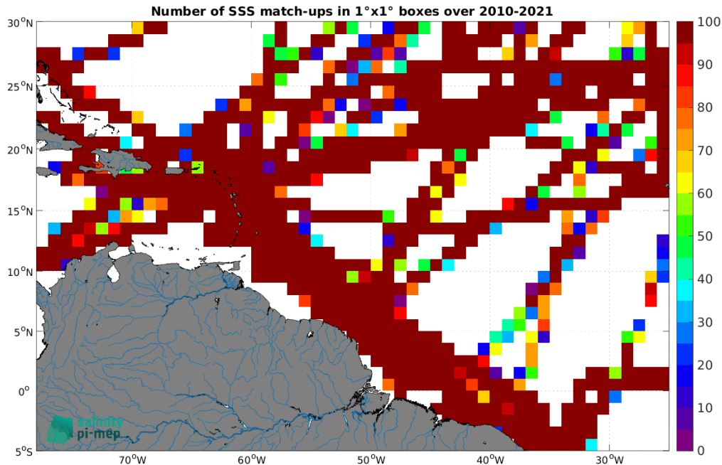
Figure 4: Number of SSS match-ups between TSG (GOSUD-Research-vessel) SSS and the SMOS SSS L3 v9 - 18 Days (CATDS-CEC-LOCEAN) SSS product for the Amazon and Orinoco river plumes Pi-MEP region over 1^\circ \times 1^\circ boxes and for the full satellite product period.
