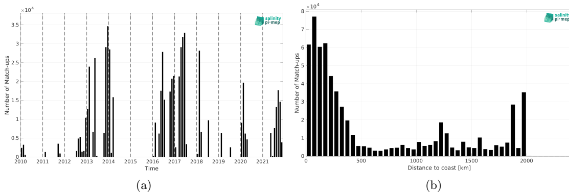
Figure 1: Number of match-ups between TSG (GOSUD-Research-vessel) and SMOS SSS L3 v9 - 18 Days (CATDS-CEC-LOCEAN) SSS as a function of time (a) and as function of the distance to coast (b) over the Amazon and Orinoco river plumes Pi-MEP region and for the full satellite product period.
