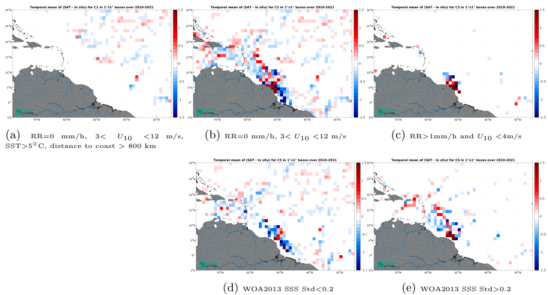
Figure 12: Temporal mean gridded over spatial boxes of size 1^\circ \times 1^\circ of \Delta SSS (SMOS SSS L3 v9 - 18 Days (CATDS-CEC-LOCEAN) - TSG (GOSUD-Research-vessel)) for 5 different subdatasets corresponding to:RR=0 mm/h, 3 < U_{10} < 12 m/s, SST >5^\circ C, distance to coast > 800 km (a), RR=0 mm/h, 3 < U_{10} < 12 m/s (b), RR >1 mm/h and U_{10} < 4 m/s (c), WOA2013 SSS Std <0.2 (d), WOA2013 SSS Std >0.2 (e).
