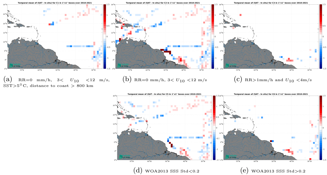
Figure 12: Temporal mean gridded over spatial boxes of size 1^\circ \times 1^\circ of \Delta SSS (SMOS SSS L3 v9 - 18 Days (CATDS-CEC-LOCEAN) - TSG (CSIC-UTM)) for 5 different subdatasets corresponding to:RR=0 mm/h, 3 < U_{10} < 12 m/s, SST >5^\circ\text{C} , distance to coast > 800 km (a), RR=0 mm/h, 3 < U_{10} < 12 m/s (b), RR >1 mm/h and U_{10} < 4 m/s (c), WOA2013 SSS Std <0.2 (d), WOA2013 SSS Std >0.2 (e).
