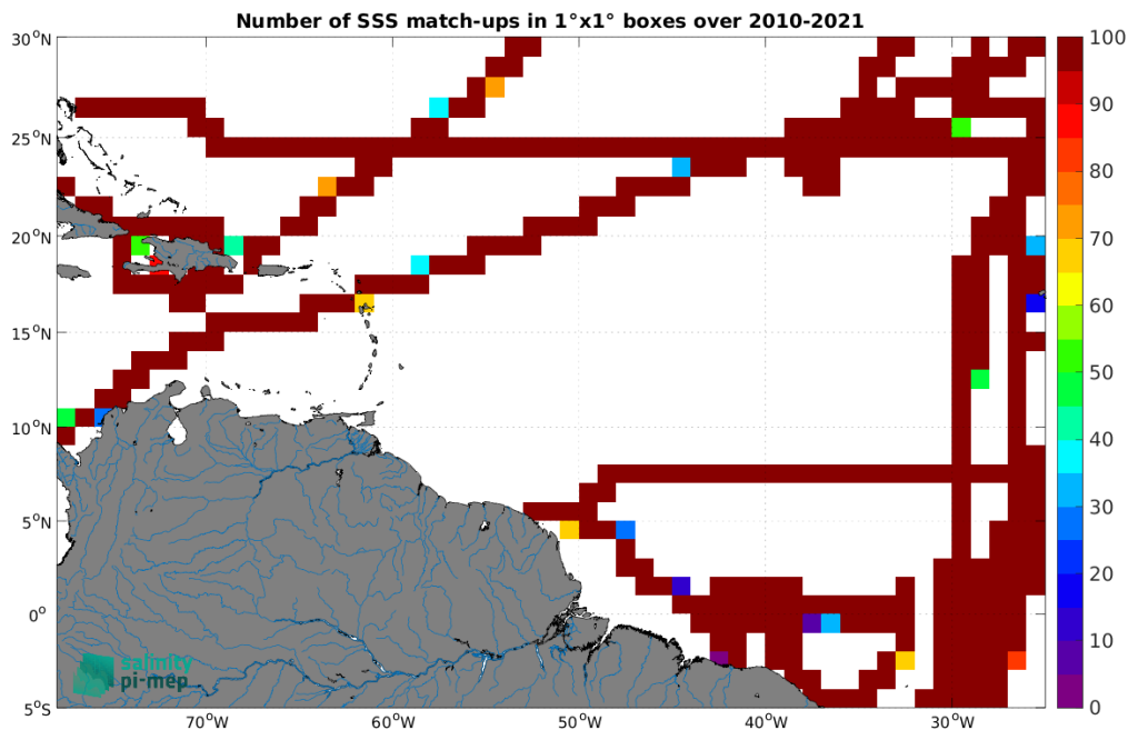
Figure 4: Number of SSS match-ups between TSG (CSIC-UTM) SSS and the SMOS SSS L3 v9 - 18 Days (CATDS-CEC-LOCEAN) SSS product for the Amazon and Orinoco river plumes Pi-MEP region over 1^\circ \times 1^\circ boxes and for the full satellite product period.
