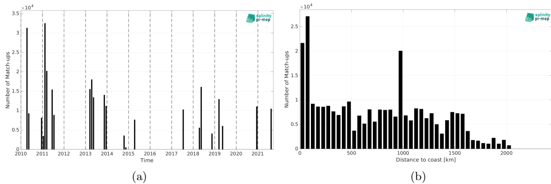
Figure 1: Number of match-ups between TSG (CSIC-UTM) and SMOS SSS L3 v9 - 18 Days (CATDS-CEC-LOCEAN) SSS as a function of time (a) and as function of the distance to coast (b) over the Amazon and Orinoco river plumes Pi-MEP region and for the full satellite product period.
