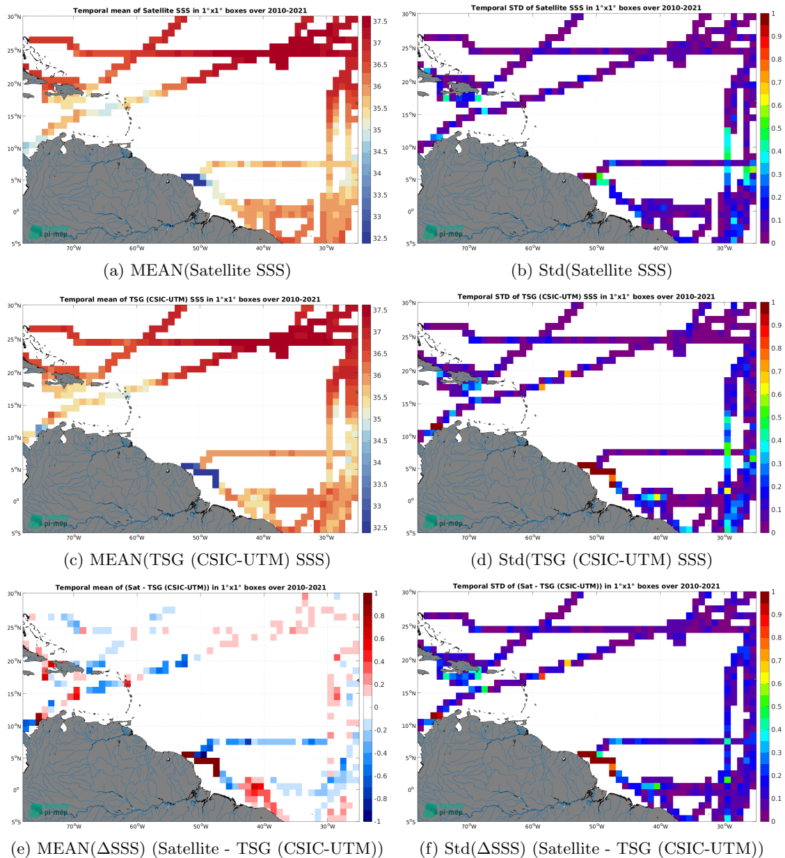
Figure 6: Temporal mean (left) and Std (right) of SSS from SMOS SSS L3 v9 - 18 Days (CATDS-CEC-LOCEAN) (top), TSG (CSIC-UTM) (middle), and of \Delta SSS (Satellite - TSG (CSIC-UTM)). Only match-up pairs are used to generate these maps.
