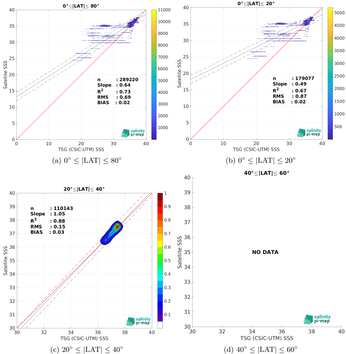
Figure 9: Contour maps of the concentration of SMOS SSS L3 v9 - 18 Days (CATDS-CEC-LOCEAN) SSS (y-axis) versus TSG (CSIC-UTM) SSS (x-axis) at match-up pairs for different latitude bands. For each plot, the red line shows x=y . The black thin and dashed lines indicate a linear fit through the data cloud and the \pm 95\% confidence levels, respectively. The number match-up pairs n , the slope and R^2 coefficient of the linear fit, the root mean square (RMS) and the mean bias between satellite and in situ data are indicated for each latitude band in each plots.
