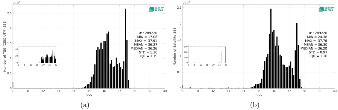
Figure 2: Histograms of SSS from TSG (CSIC-UTM) (a) and SMOS SSS L3 v9 - 18 Days (CATDS-CEC-LOCEAN) (b) considering all match-up pairs per bins of 0.1 over the Amazon and Orinoco river plumes Pi-MEP region and for the full satellite product period.
