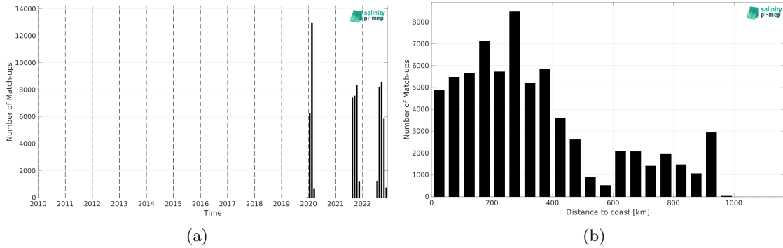
Figure 2: Number of match-ups between Saildrone and SMOS SSS L3 v9 - 18 Days (CATDS-CEC-LOCEAN) SSS as a function of time (a) and as function of the distance to coast (b) over the Amazon and Orinoco river plumes Pi-MEP region and for the full satellite product period.
