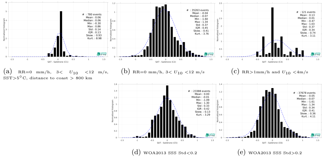
Figure 15: Normalized histogram of \Delta\text{SSS} (SMOS SSS L3 v9 - 18 Days (CATDS-CEC-LOCEAN) - Saldrone) for 5 different subdatasets corresponding to: RR=0 mm/h, 3 < U_{10} < 12 m/s, SST > 5^\circ\text{C} , distance to coast > 800 km (a), RR=0 mm/h, 3 < U_{10} < 12 m/s (b), RR > 1\text{mm/h} and U_{10} < 4\text{m/s} (c), WOA2013 SSS Std < 0.2 (d), WOA2013 SSS Std > 0.2 (e).
