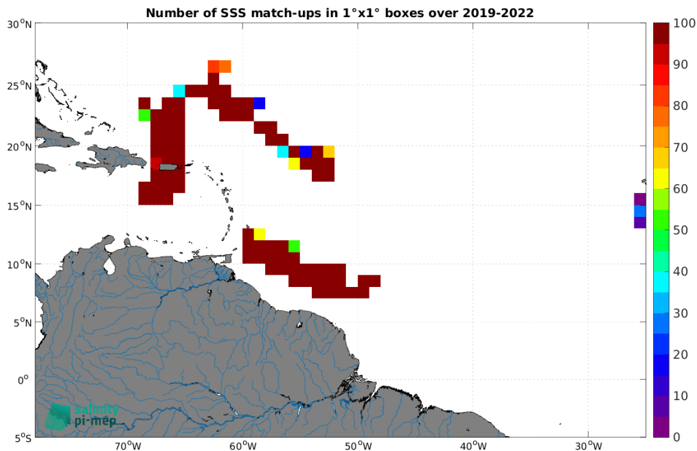
Figure 5: Number of SSS match-ups between Saildrone SSS and the SMOS SSS L3 v9 - 18 Days (CATDS-CEC-LOCEAN) SSS product for the Amazon and Orinoco river plumes Pi-MEP region over 1^\circ \times 1^\circ boxes and for the full satellite product period.
