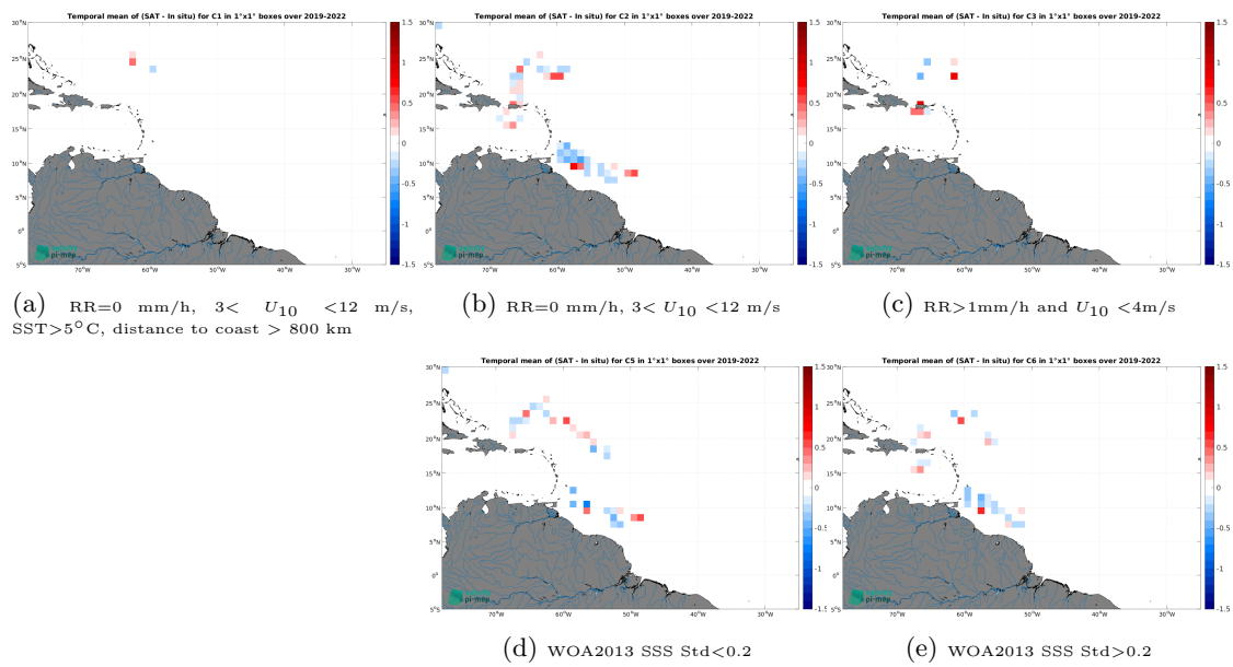
Figure 14: Temporal mean gridded over spatial boxes of size 1^\circ \times 1^\circ of \Delta SSS (SMOS SSS L3 v9 - 18 Days (CATDS-CEC-LOCEAN) - Sailydrone) for 5 different subdatasets corresponding to:RR=0 mm/h, 3 < U_{10} < 12 m/s, SST >5^\circ\text{C} , distance to coast > 800 km (a), RR=0 mm/h, 3 < U_{10} < 12 m/s (b), RR >1 mm/h and U_{10} < 4 m/s (c), WOA2013 SSS Std <0.2 (d), WOA2013 SSS Std >0.2 (e).
