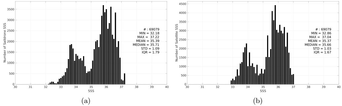
Figure 3: Histograms of SSS from Saildrone (a) and SMOS SSS L3 v9 - 18 Days (CATDS-CEC-LOCEAN) (b) considering all match-up pairs per bins of 0.1 over the Amazon and Orinoco river plumes Pi-MEP region and for the full satellite product period.
