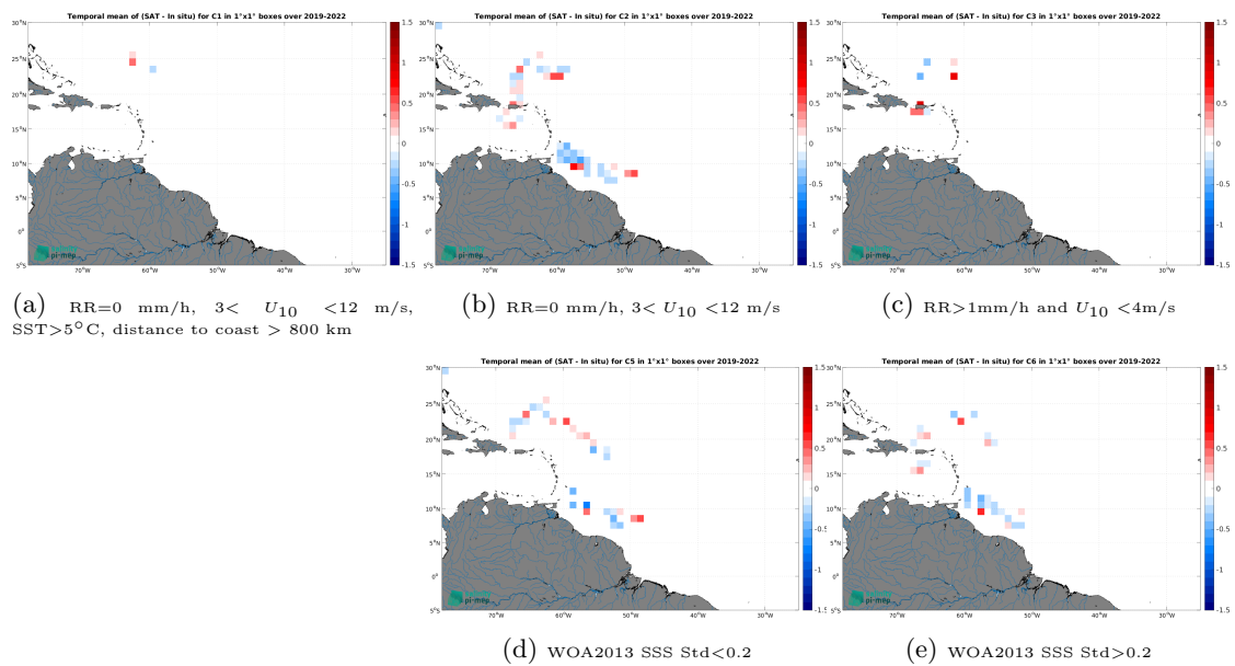
Figure 14: Temporal mean gridded over spatial boxes of size 1^\circ \times 1^\circ of \Delta SSS (SMOS SSS L3 v9 - 18 Days (CATDS-CEC-LOCEAN) - Sairdrone) for 5 different subdatasets corresponding to:RR=0 mm/h, 3 < U_{10} < 12 m/s, SST >5^\circ\text{C} , distance to coast > 800 km (a), RR=0 mm/h, 3 < U_{10} < 12 m/s (b), RR >1 mm/h and U_{10} < 4 m/s (c), WOA2013 SSS Std <0.2 (d), WOA2013 SSS Std >0.2 (e).
