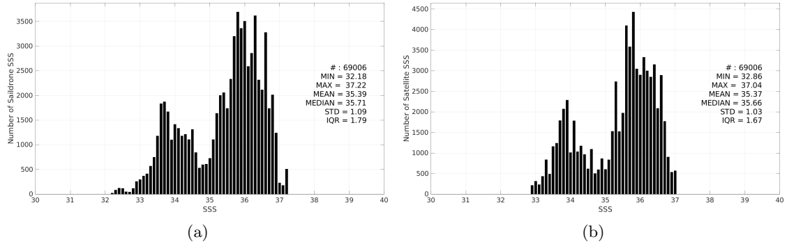
Figure 2: Histograms of SSS from Saildrone (a) and SMOS SSS L3 v9 - 18 Days (CATDS-CEC-LOCEAN) (b) considering all match-up pairs per bins of 0.1 over the Amazon and Orinoco river plumes Pi-MEP region and for the full satellite product period.
