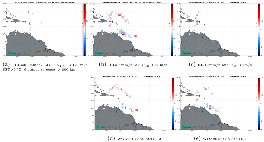
Figure 12: Temporal mean gridded over spatial boxes of size 1^\circ \times 1^\circ of \Delta SSS (SMOS SSS L3 v9 - 18 Days (CATDS-CEC-LOCEAN) - Saldrone) for 5 different subdatasets corresponding to:RR=0 mm/h, 3 < U_{10} < 12 m/s, SST >5^\circ\text{C} , distance to coast > 800 km (a), RR=0 mm/h, 3 < U_{10} < 12 m/s (b), RR >1 mm/h and U_{10} < 4 m/s (c), WOA2013 SSS Std <0.2 (d), WOA2013 SSS Std >0.2 (e).
