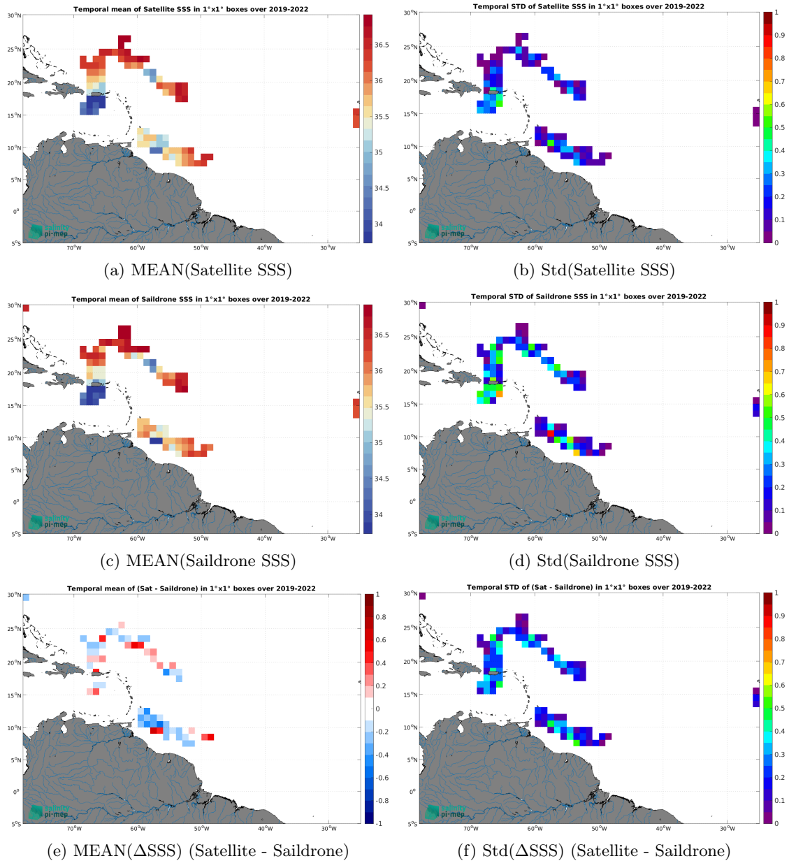
Figure 6: Temporal mean (left) and Std (right) of SSS from SMOS SSS L3 v9 - 18 Days (CATDS-CEC-LOCEAN) (top), Saildrone (middle), and of \Delta SSS (Satellite - Saildrone). Only match-up pairs are used to generate these maps.
