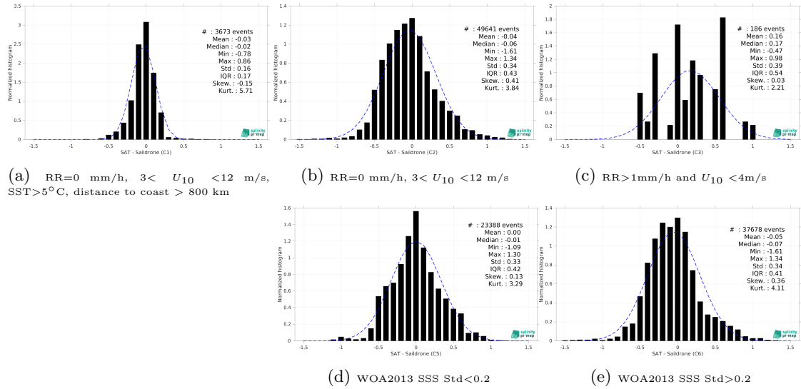
Figure 13: Normalized histogram of \Delta SSS (SMOS SSS L3 v9 - 18 Days (CATDS-CEC-LOCEAN) - Saildrone) for 5 different subdatasets corresponding to: RR=0 mm/h, 3 < U_{10} < 12 m/s, SST>5°C, distance to coast > 800 km (a), RR=0 mm/h, 3 < U_{10} < 12 m/s (b), RR>1mm/h and U_{10} < 4 m/s (c), WOA2013 SSS Std<0.2 (d), WOA2013 SSS Std>0.2 (e).
