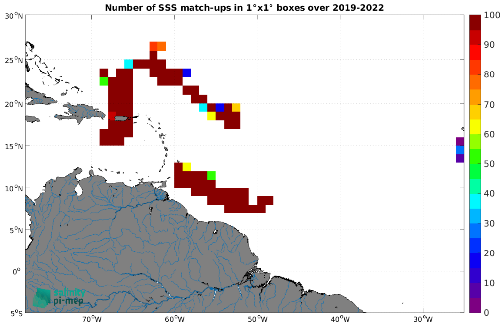
Figure 4: Number of SSS match-ups between Saildrone SSS and the SMOS SSS L3 v9 - 18 Days (CATDS-CEC-LOCEAN) SSS product for the Amazon and Orinoco river plumes Pi-MEP region over 1^\circ \times 1^\circ boxes and for the full satellite product period.
