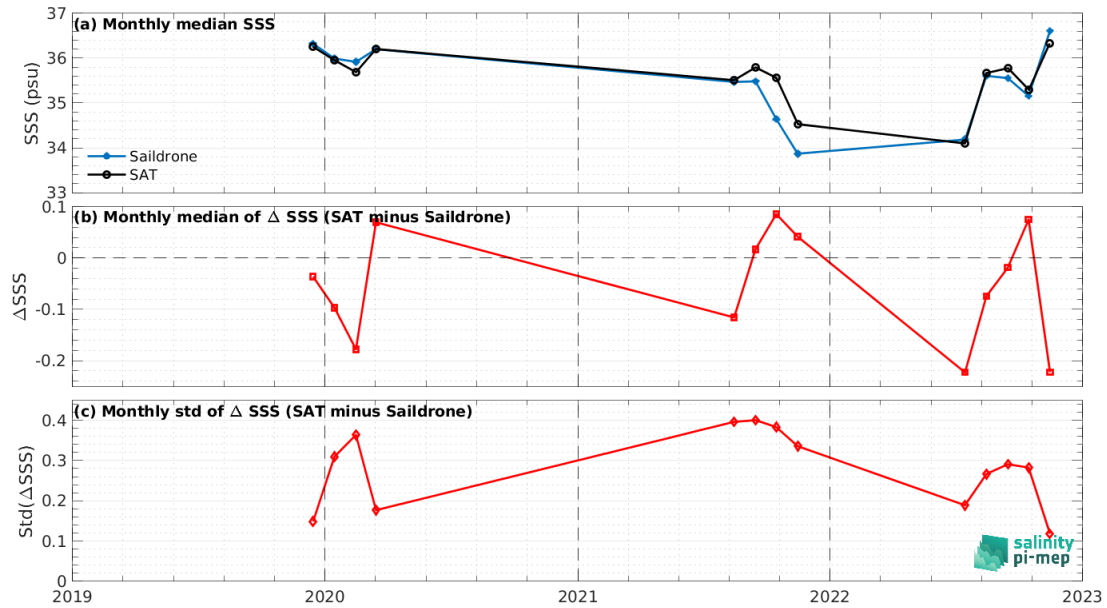
Figure 7: Time series of the monthly median SSS (top), median of \Delta\text{SSS} (Satellite - Sairdrone) and Std of \Delta\text{SSS} (Satellite - Sairdrone) over the Amazon and Orinoco river plumes Pi-MEP region considering all match-ups collected by the Pi-MEP.
