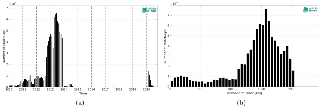
Figure 1: Number of match-ups between Surface drifters and SMOS SSS L3 v9 - 18 Days (CATDS-CEC-LOCEAN) SSS as a function of time (a) and as function of the distance to coast (b) over the Amazon and Orinoco river plumes Pi-MEP region and for the full satellite product period.
