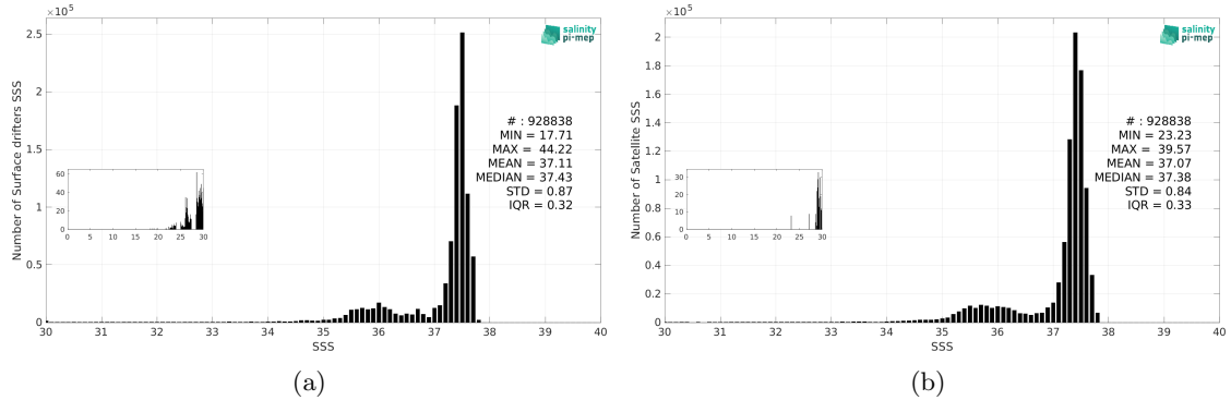
Figure 2: Histograms of SSS from Surface drifters (a) and SMOS SSS L3 v9 - 18 Days (CATDS-CEC-LOCEAN) (b) considering all match-up pairs per bins of 0.1 over the Amazon and Orinoco river plumes Pi-MEP region and for the full satellite product period.
