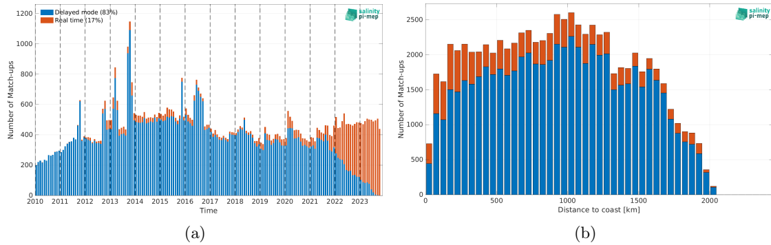
Figure 1: Number of match-ups between Argo and SMOS SSS L3 v9 - 18 Days (CATDS-CEC-LOCEAN) SSS as a function of time (a) and as function of the distance to coast (b) over the Amazon and Orinoco river plumes Pi-MEP region and for the full satellite product period.
