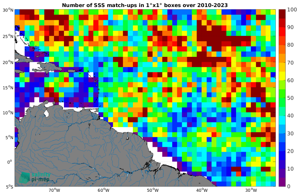
Figure 4: Number of SSS match-ups between Argo SSS and the SMOS SSS L3 v9 - 18 Days (CATDS-CEC-LOCEAN) SSS product for the Amazon and Orinoco river plumes Pi-MEP region over 1^\circ \times 1^\circ boxes and for the full satellite product period.
