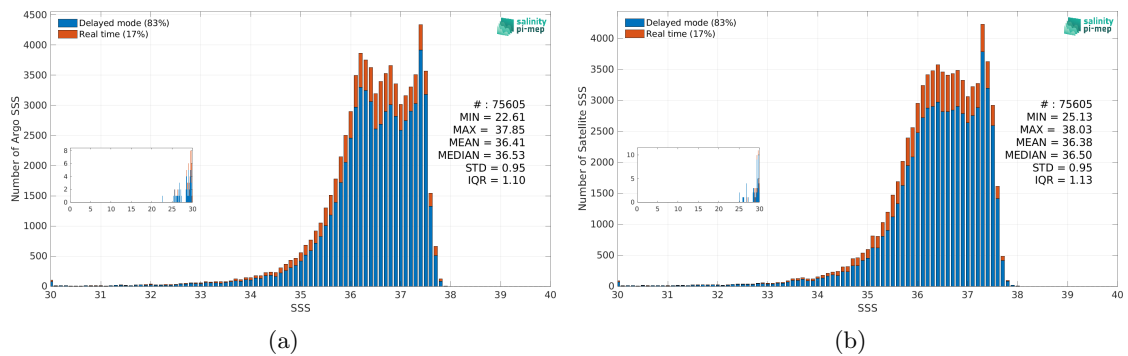
Figure 2: Histograms of SSS from Argo (a) and SMOS SSS L3 v9 - 18 Days (CATDS-CEC-LOCEAN) (b) considering all match-up pairs per bins of 0.1 over the Amazon and Orinoco river plumes Pi-MEP region and for the full satellite product period.
