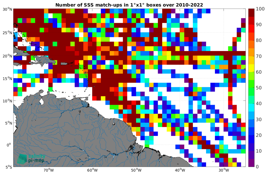
Figure 4: Number of SSS match-ups between TSG (SAMOS) SSS and the SMOS SSS L3 v8 - 9 Days (CATDS-CEC-LOCEAN) SSS product for the Amazon and Orinoco river plumes Pi-MEP region over 1^\circ \times 1^\circ boxes and for the full satellite product period.
