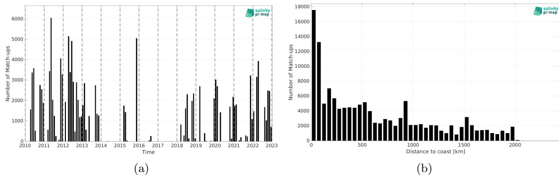
Figure 1: Number of match-ups between TSG (SAMOS) and SMOS SSS L3 v8 - 9 Days (CATDS-CEC-LOCEAN) SSS as a function of time (a) and as function of the distance to coast (b) over the Amazon and Orinoco river plumes Pi-MEP region and for the full satellite product period.
