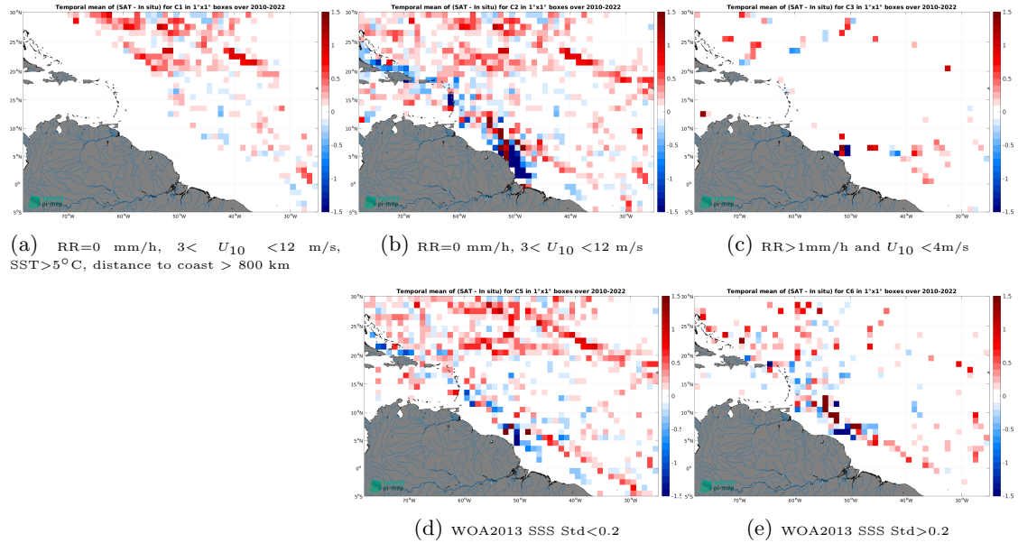
Figure 12: Temporal mean gridded over spatial boxes of size 1^{\circ}\times 1^{\circ} of \Delta\text{SSS} (SMOS SSS L3 v8 - 9 Days (CATDS-CEC-LOCEAN) - TSG (SAMOS)) for 5 different subdatasets corresponding to:RR=0 mm/h, 3 < U_{10} < 12 m/s, SST >5^{\circ}\text{C} , distance to coast > 800 km (a), RR=0 mm/h, 3 < U_{10} < 12 m/s (b), RR >1 mm/h and U_{10} < 4 m/s (c), WOA2013 SSS Std <0.2 (d), WOA2013 SSS Std >0.2 (e).
