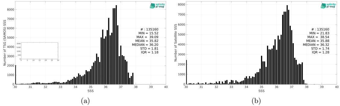
Figure 2: Histograms of SSS from TSG (SAMOS) (a) and SMOS SSS L3 v8 - 9 Days (CATDS-CEC-LOCEAN) (b) considering all match-up pairs per bins of 0.1 over the Amazon and Orinoco river plumes Pi-MEP region and for the full satellite product period.
