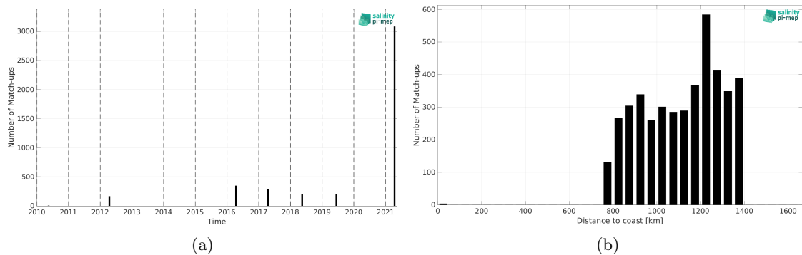
Figure 1: Number of match-ups between TSG (Polarstern) and SMOS SSS L3 v8 - 9 Days (CATDS-CEC-LOCEAN) SSS as a function of time (a) and as function of the distance to coast (b) over the Amazon and Orinoco river plumes Pi-MEP region and for the full satellite product period.
