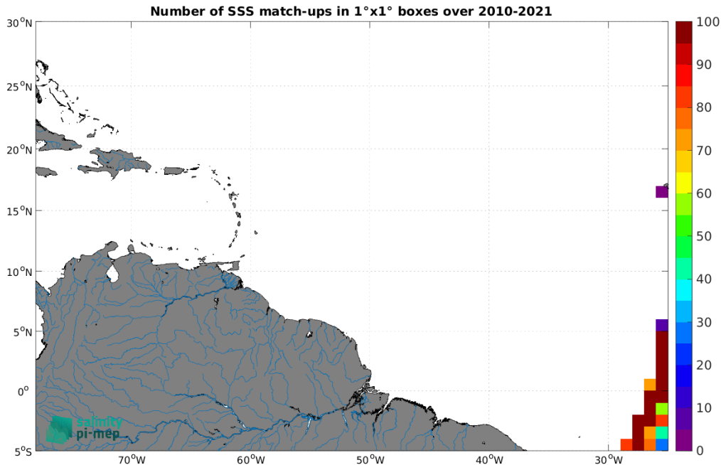
Figure 4: Number of SSS match-ups between TSG (Polarstern) SSS and the SMOS SSS L3 v8 - 9 Days (CATDS-CEC-LOCEAN) SSS product for the Amazon and Orinoco river plumes Pi-MEP region over 1^\circ \times 1^\circ boxes and for the full satellite product period.
