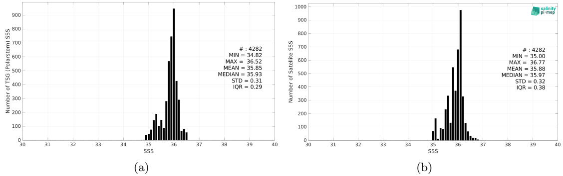
Figure 2: Histograms of SSS from TSG (Polarstern) (a) and SMOS SSS L3 v8 - 9 Days (CATDS-CEC-LOCEAN) (b) considering all match-up pairs per bins of 0.1 over the Amazon and Orinoco river plumes Pi-MEP region and for the full satellite product period.
