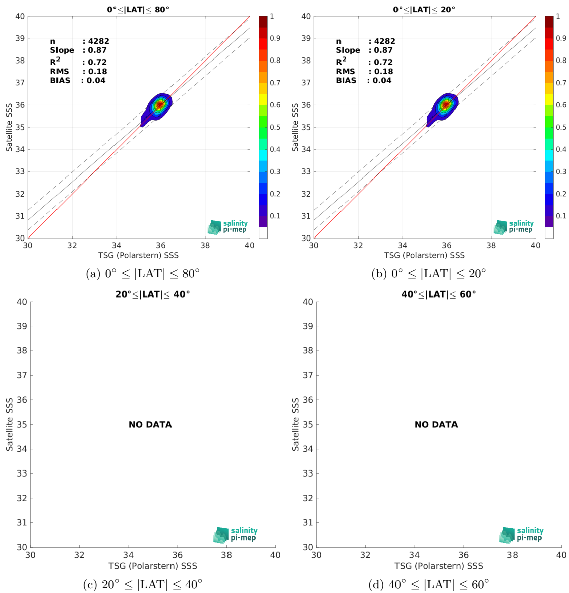
Figure 9: Contour maps of the concentration of SMOS SSS L3 v8 - 9 Days (CATDS-CEC-LOCEAN) SSS (y-axis) versus TSG (Polarstern) SSS (x-axis) at match-up pairs for different latitude bands. For each plot, the red line shows x=y . The black thin and dashed lines indicate a linear fit through the data cloud and the \pm 95\% confidence levels, respectively. The number match-up pairs n , the slope and R^2 coefficient of the linear fit, the root mean square (RMS) and the mean bias between satellite and in situ data are indicated for each latitude band in each plots.
