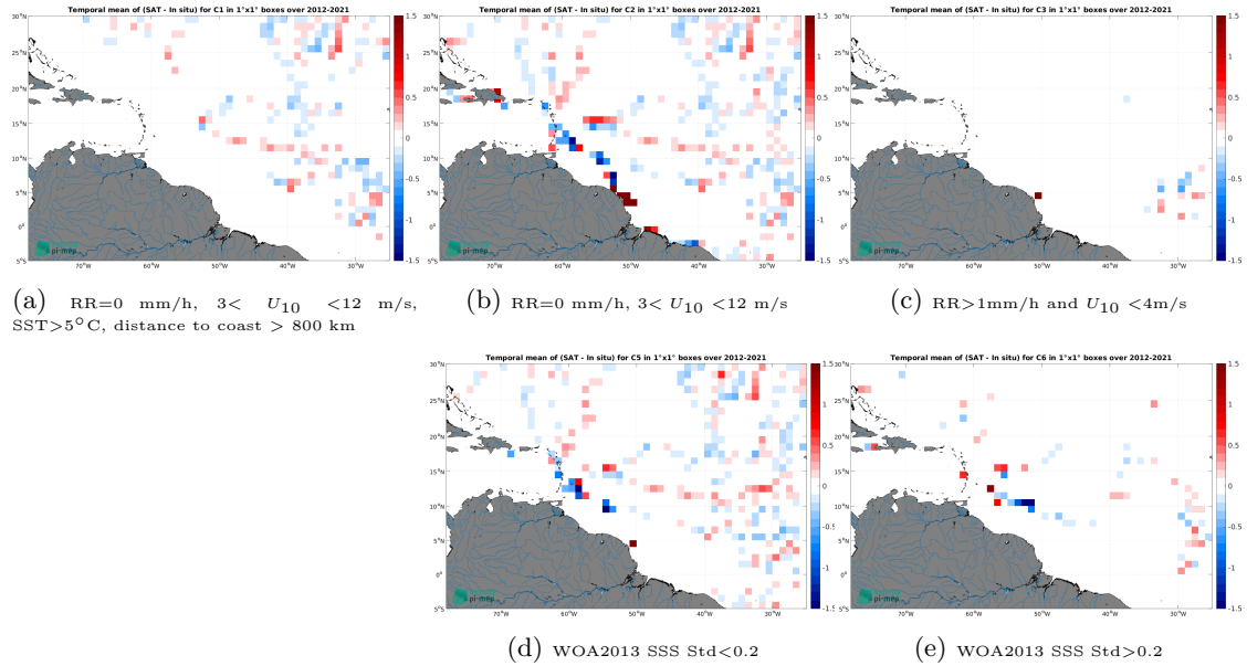
Figure 12: Temporal mean gridded over spatial boxes of size 1^{\circ}\times 1^{\circ} of \Delta SSS (SMOS SSS L3 v8 - 9 Days (CATDS-CEC-LOCEAN) - TSG (GOSUD-Sailing-ship)) for 5 different subdatasets corresponding to:RR=0 mm/h, 3 < U_{10} < 12 m/s, SST >5^{\circ}\text{C} , distance to coast > 800 km (a), RR=0 mm/h, 3 < U_{10} < 12 m/s (b), RR >1 mm/h and U_{10} < 4 m/s (c), WOA2013 SSS Std <0.2 (d), WOA2013 SSS Std >0.2 (e).
