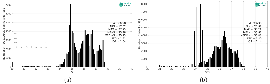
Figure 2: Histograms of SSS from TSG (GOSUD-Sailing-ship) (a) and SMOS SSS L3 v8 - 9 Days (CATDS-CEC-LOCEAN) (b) considering all match-up pairs per bins of 0.1 over the Amazon and Orinoco river plumes Pi-MEP region and for the full satellite product period.
