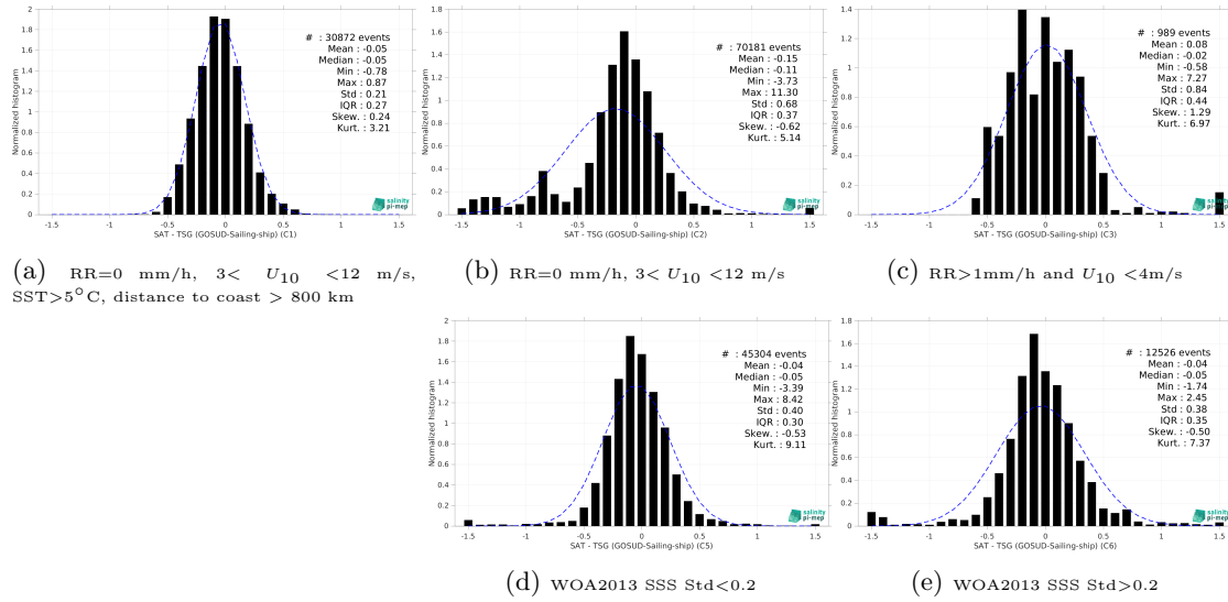
Figure 13: Normalized histogram of \Delta\text{SSS} (SMOS SSS L3 v8 - 9 Days (CATDS-CEC-LOCEAN) - TSG (GOSUD-Sailing-ship)) for 5 different subdatasets corresponding to: RR=0 mm/h, 3 < U_{10} < 12 m/s, SST>5°C, distance to coast > 800 km (a), RR=0 mm/h, 3 < U_{10} < 12 m/s (b), RR>1mm/h and U_{10} < 4 m/s (c), WOA2013 SSS Std<0.2 (d), WOA2013 SSS Std>0.2 (e).
