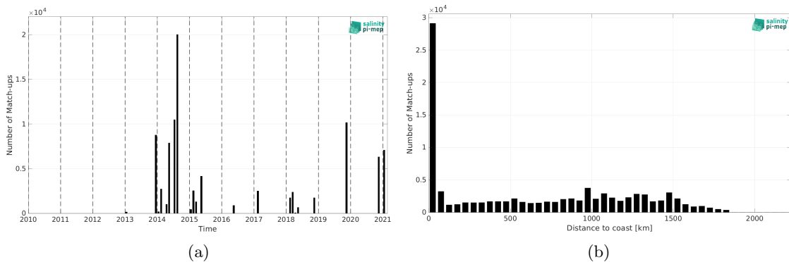
Figure 1: Number of match-ups between TSG (GOSUD-Sailing-ship) and SMOS SSS L3 v8 - 9 Days (CATDS-CEC-LOCEAN) SSS as a function of time (a) and as function of the distance to coast (b) over the Amazon and Orinoco river plumes Pi-MEP region and for the full satellite product period.
