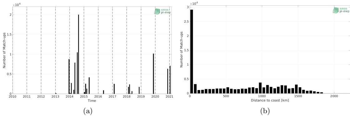
Figure 1: Number of match-ups between TSG (GOSUD-Sailing-ship) and SMOS SSS L3 v8 - 9 Days (CATDS-CECOS-LOCEAN) SSS as a function of time (a) and as function of the distance to coast (b) over the Amazon and Orinoco river plumes Pi-MEP region and for the full satellite product period.
