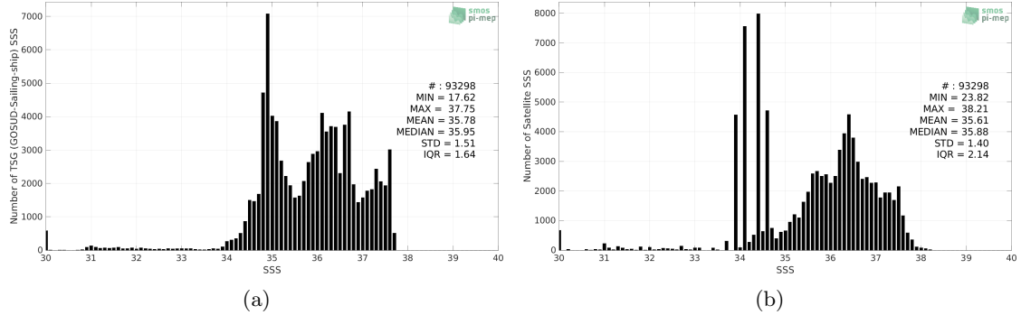
Figure 2: Histograms of SSS from TSG (GOSUD-Sailing-ship) (a) and SMOS SSS L3 v8 - 9 Days (CATDS-CECOS-LOCEAN) (b) considering all match-up pairs per bins of 0.1 over the Amazon and Orinoco river plumes Pi-MEP region and for the full satellite product period.
