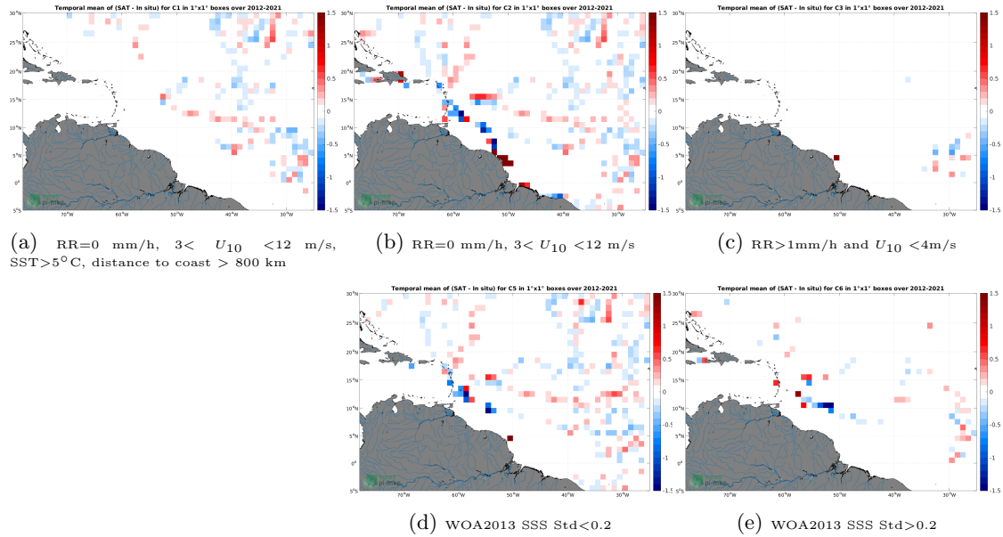
Figure 12: Temporal mean gridded over spatial boxes of size 1^{\circ}\times 1^{\circ} of \Delta SSS (SMOS SSS L3 v8 - 9 Days (CATDS-CECOS-LOCEAN) - TSG (GOSUD-Sailing-ship)) for 5 different subdatasets corresponding to:RR=0 mm/h, 3 < U_{10} < 12 m/s, SST >5^{\circ}\text{C} , distance to coast > 800 km (a), RR=0 mm/h, 3 < U_{10} < 12 m/s (b), RR >1 mm/h and U_{10} < 4 m/s (c), WOA2013 SSS Std <0.2 (d), WOA2013 SSS Std >0.2 (e).
