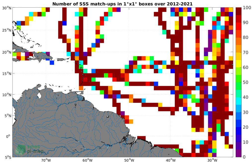
Figure 4: Number of SSS match-ups between TSG (GOSUD-Sailing-ship) SSS and the SMOS SSS L3 v8 - 9 Days (CATDS-CECOS-LOCEAN) SSS product for the Amazon and Orinoco river plumes Pi-MEP region over 1^\circ \times 1^\circ boxes and for the full satellite product period.
