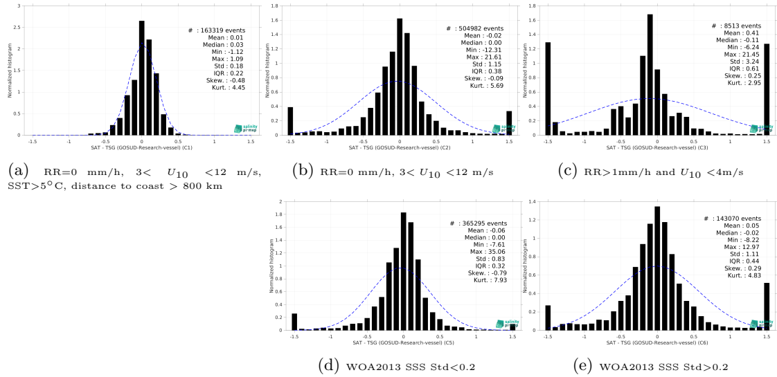
Figure 13: Normalized histogram of \Delta SSS (SMOS SSS L3 v8 - 9 Days (CATDS-CEC-LOCEAN) - TSG (GOSUD-Research-vessel)) for 5 different subdatasets corresponding to: RR=0 mm/h, 3 < U_{10} < 12 m/s, SST>5°C, distance to coast > 800 km (a), RR=0 mm/h, 3 < U_{10} < 12 m/s (b), RR>1mm/h and U_{10} < 4 m/s (c), WOA2013 SSS Std<0.2 (d), WOA2013 SSS Std>0.2 (e).
