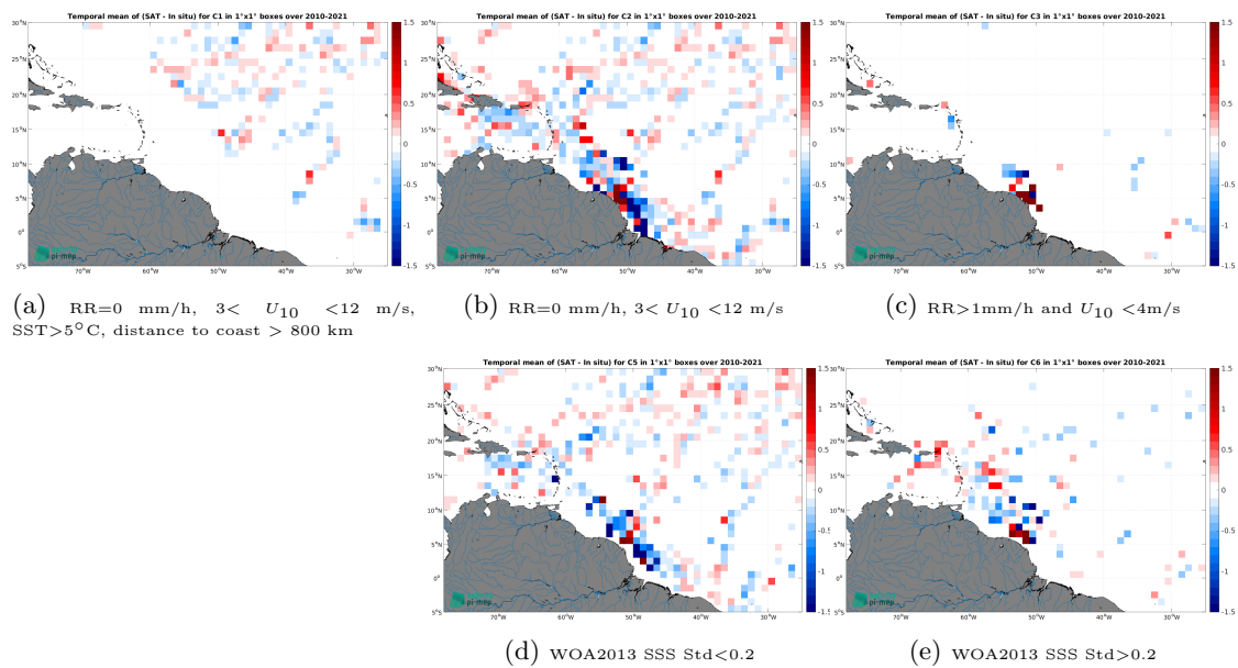
Figure 12: Temporal mean gridded over spatial boxes of size 1^\circ \times 1^\circ of \Delta SSS (SMOS SSS L3 v8 - 9 Days (CATDS-CEC-LOCEAN) - TSG (GOSUD-Research-vessel)) for 5 different subdatasets corresponding to:RR=0 mm/h, 3 < U_{10} < 12 m/s, SST >5^\circ C, distance to coast > 800 km (a), RR=0 mm/h, 3 < U_{10} < 12 m/s (b), RR >1 mm/h and U_{10} < 4 m/s (c), WOA2013 SSS Std <0.2 (d), WOA2013 SSS Std >0.2 (e).
