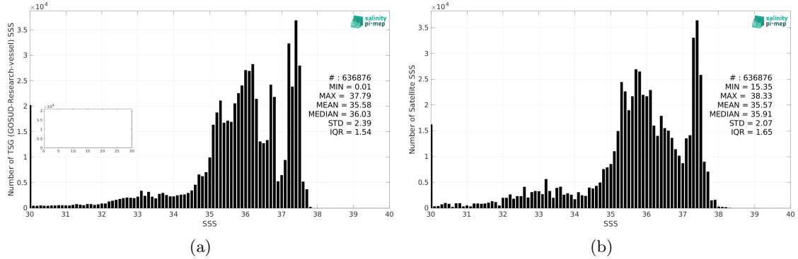
Figure 2: Histograms of SSS from TSG (GOSUD-Research-vessel) (a) and SMOS SSS L3 v8 - 9 Days (CATDS-CEC-LOCEAN) (b) considering all match-up pairs per bins of 0.1 over the Amazon and Orinoco river plumes Pi-MEP region and for the full satellite product period.
